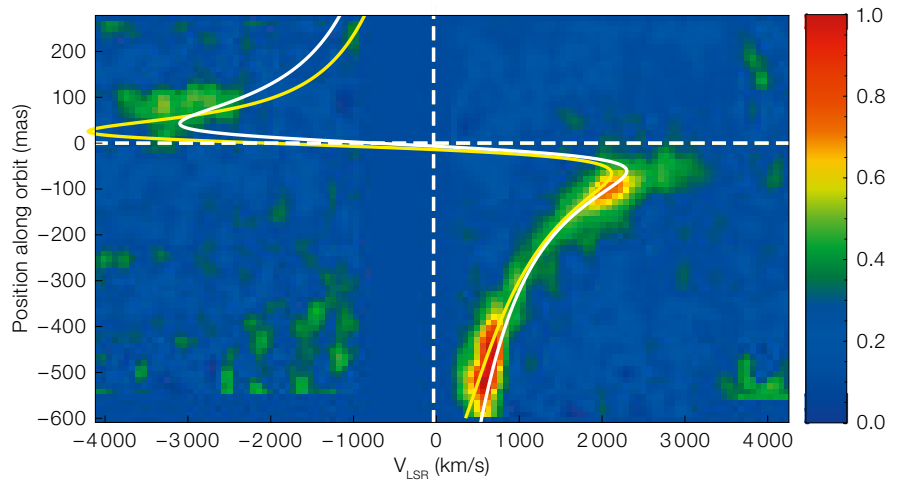
Figure 3. The full depth of the velocity–position diagram of G2 is revealed from the 24.4-hour 2013 SINFONI observation by extraction of the spectrum along the (curved) orbit path (from Gillessen et al., 2013b). The yellow line depicts the L -band orbit which differs slightly from the Brackett- \gamma one (white line).
