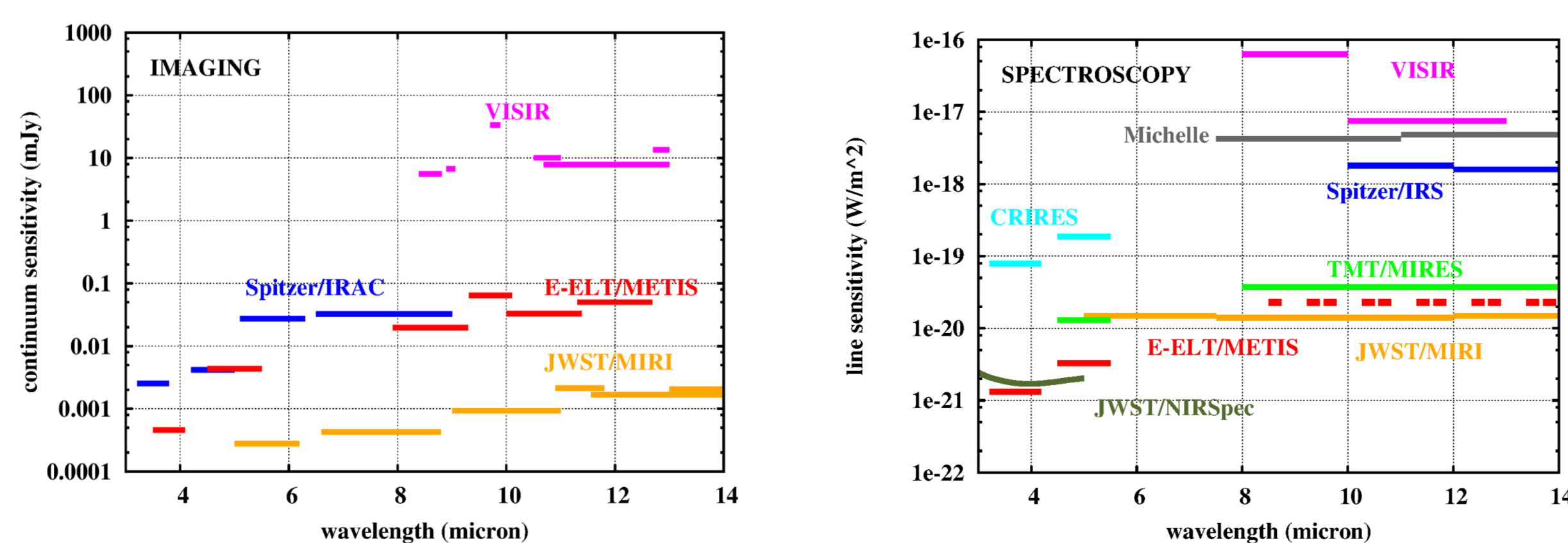
Sensitivity of the IFU-spectrograph and imager of METIS compared to other current and future instruments. Sensitivities are given for a one hour exposure of a point source (unresolved line, with 20% overhead and a signal-to-noise of 10). The calculations of the spectrometer sensitivities are based on an earlier version of the simulator developed by Kendrew et al.
