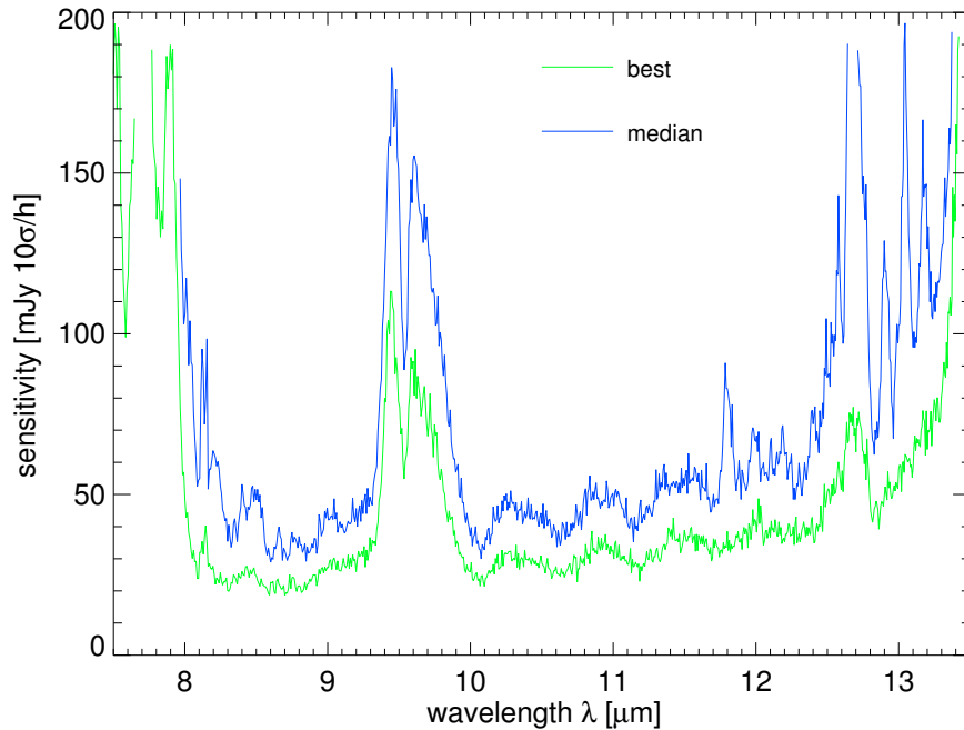
Figure 10: Median and best low resolution sensitivities [mJy/10 \sigma /h] observed during commissioning 2 under mediocre atmospheric conditions.
