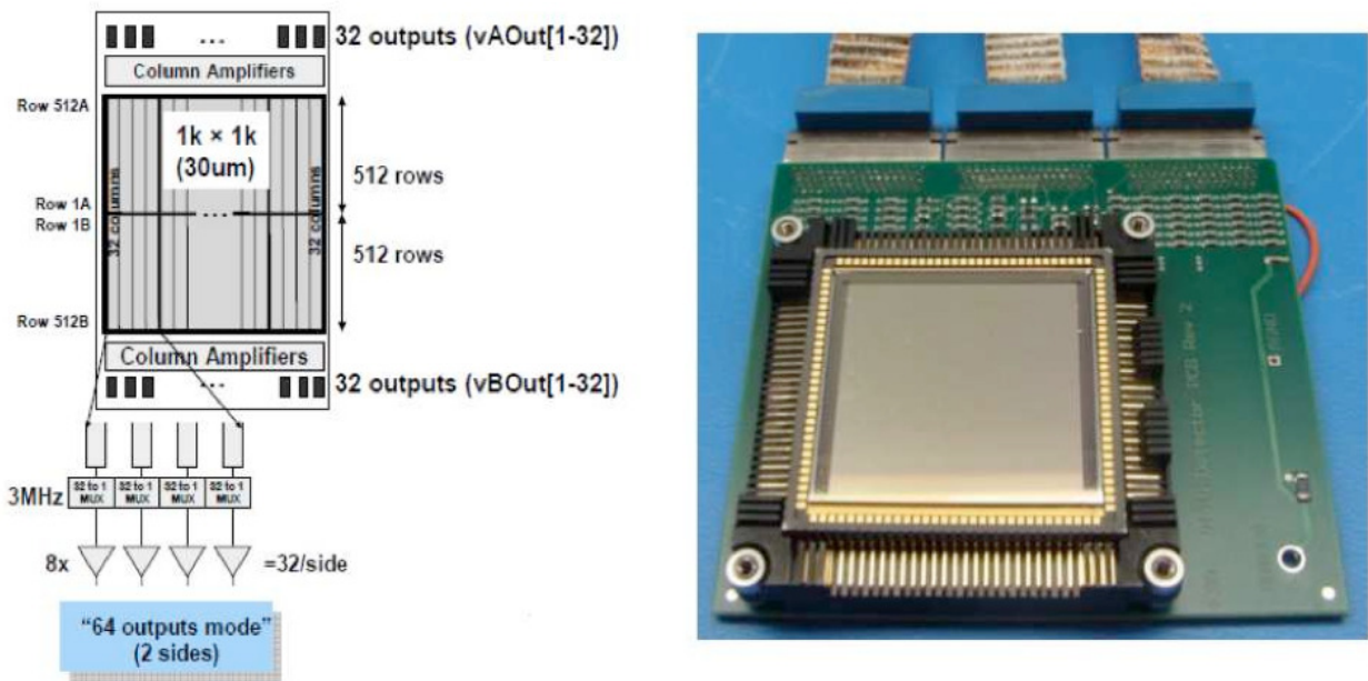
Figure 12: Left panel shows the AQUARIUS multiplexing readout scheme. Right panel shows the detector mounted in its socket.
