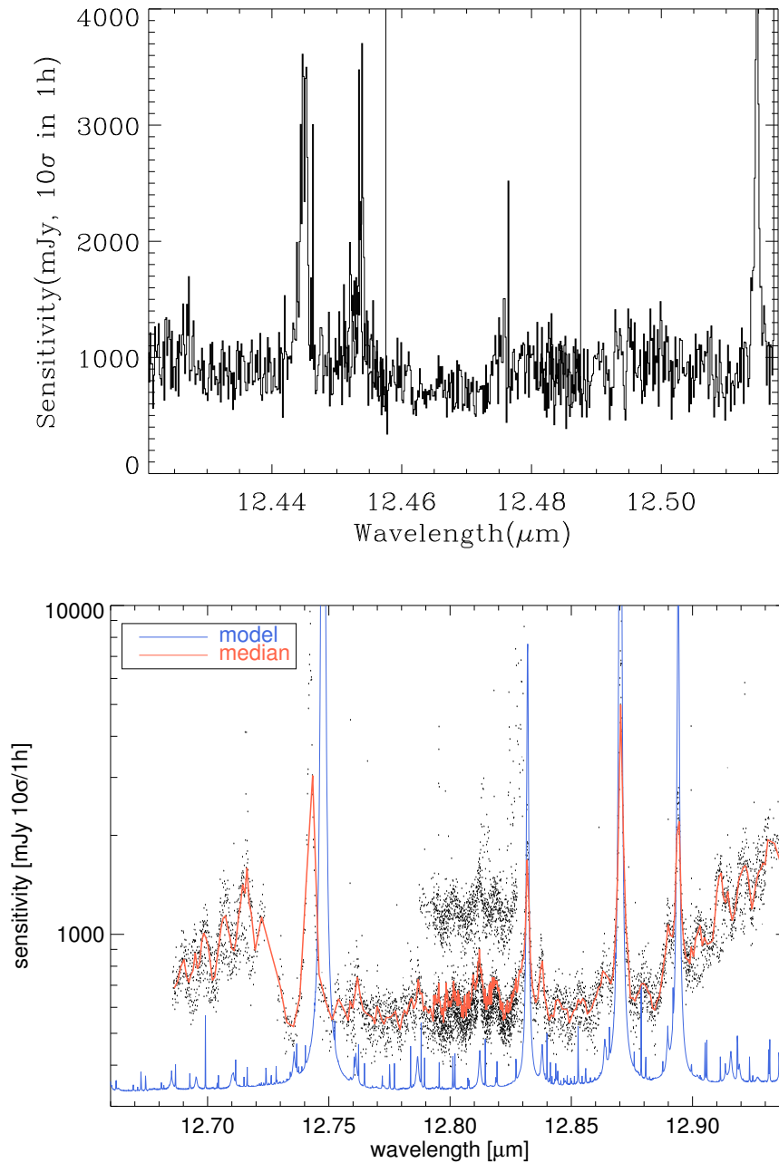
Figure 22: Observed sensitivity measured for the old DRS detector as a function of wavelength for high resolution mode (III). Offered sensitivity is typically a factor of 2 larger and still valid for Period 95. Bottom: Observed sensitivities obtained on various nights, compared with the theoretical model curves, corresponding to BLIP.
