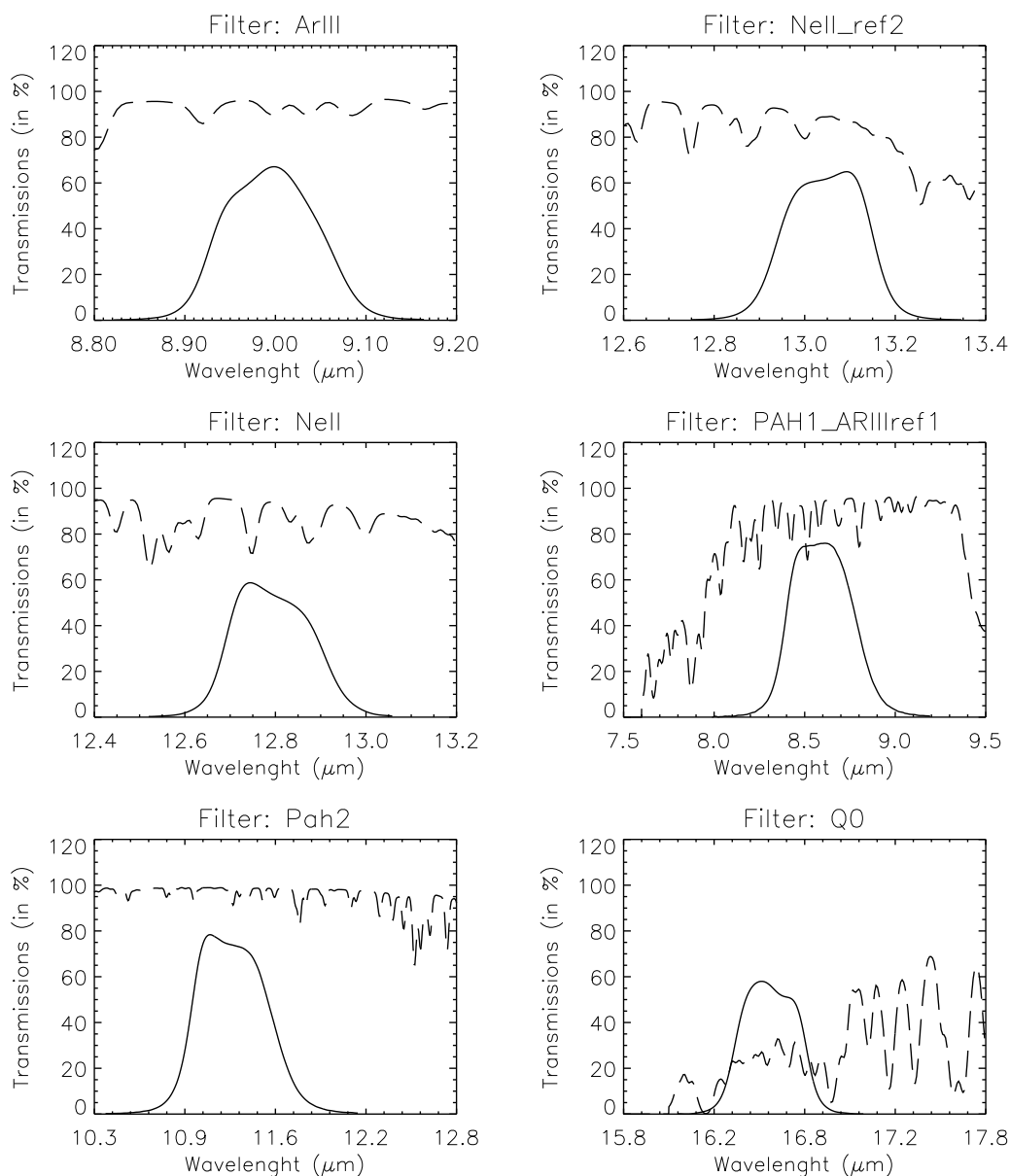
Figure 21: Transmission curves of VISIR imager filters, manufactured by READING. Overplotted (dashed) is the atmospheric transmission at low resolution. The absolute transmission values are given, expressed in percent.
