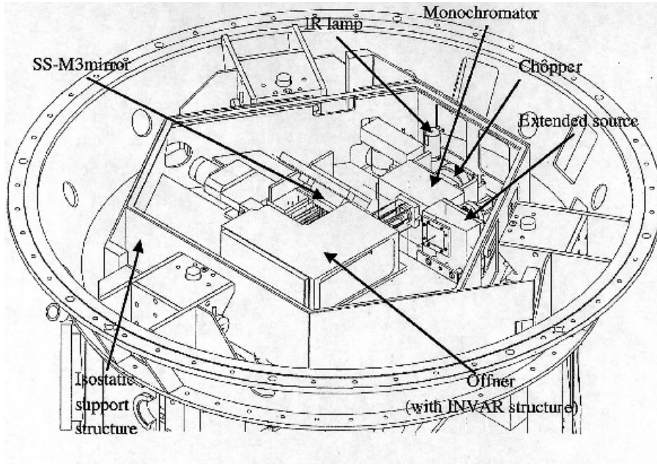
Figure 11: Schematic drawing of the warm calibration unit on top of the VISIR vessel.
