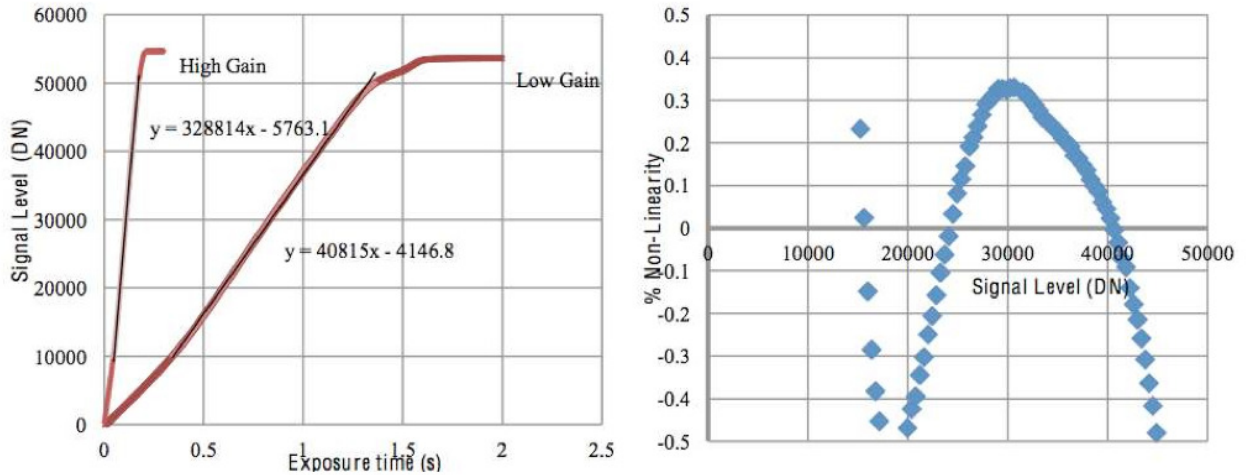
Figure 13: Left panel displays the measured AQUARIUS detector linearity for both high and low gain read modes. Right panel displays the non-linearity as a function of the signal level, as computed for the high gain setup.
