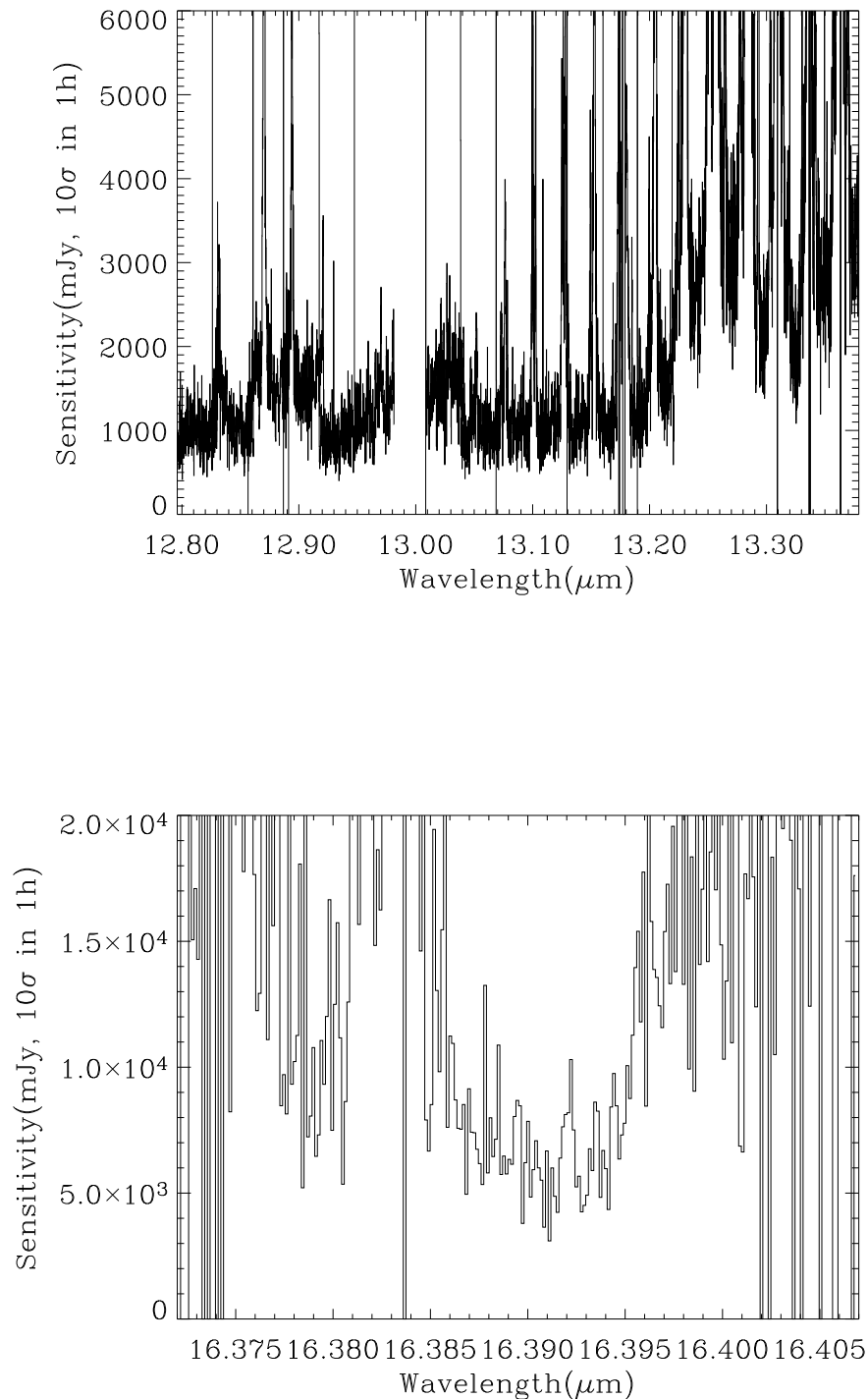
Figure 23: Observed sensitivity measured for the old DRS detector as a function of wavelength for high resolution mode (IV). Offered sensitivity is typically a factor of 2 larger and still valid for Period 95. Top : Sensitivities over an extended region encompassing the observed wavelength of [NeII] up to z \approx 0.038 .
