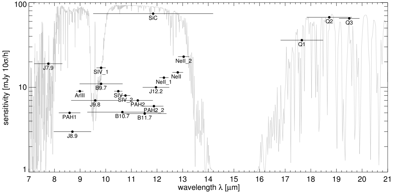
Figure 6: Sensitivities for the VISIR imager in various filters in the N- and Q-bands determined with the new AQUARIUS detector during the re-commissioning. The atmospheric transparency spectrum for PWV = 3 mm at an airmass of 1.5 is plotted in the background.
