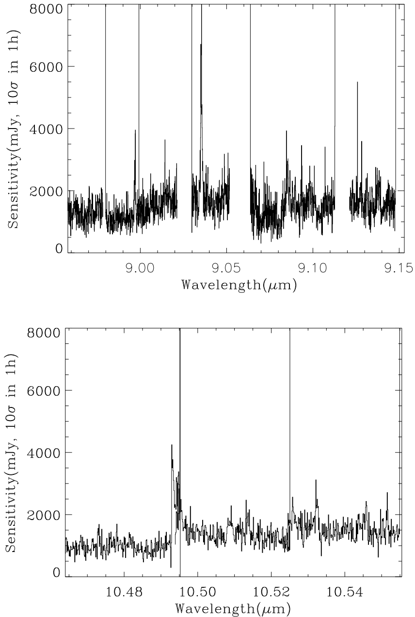
Figure 20: Observed sensitivity measured for the old DRS detector as a function of wavelength for high resolution mode (I). Offered sensitivity is typically a factor of 2 larger and still valid for Period 95.
