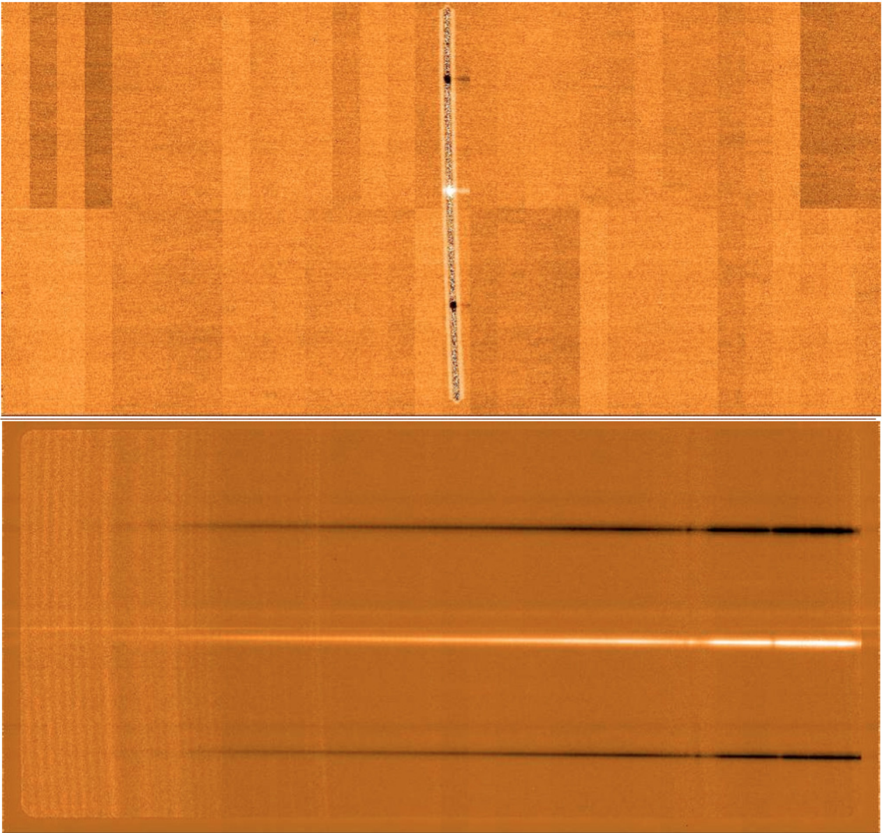
Figure 14: Upper panel: An example of the good cosmetics on the new AQUARIUS detector, used for the acquisition of a Cohen standard in the 1''.0 slit. Note the central division of the detector due to the intrinsic central-outward readout, and how the target was placed slightly above. Lower panel: A sequence of chop/nod, reduced spectra obtained in the low resolution mode, covering the entire N-band with a single exposure. The TEL.CHOP.THROW was set to 10'' .
