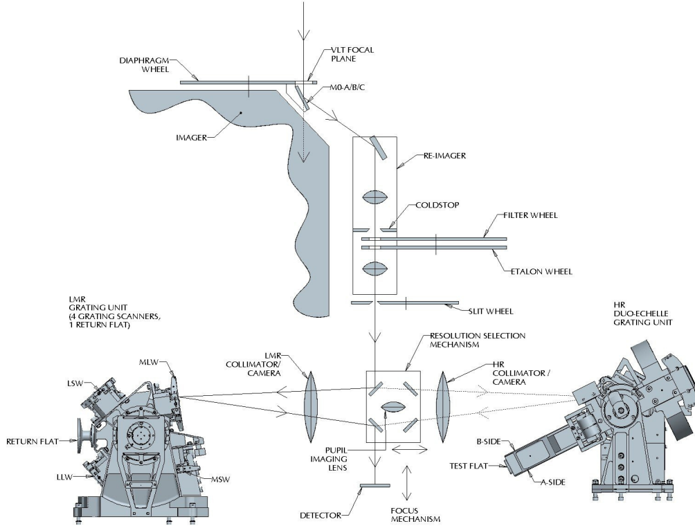
Figure 9: Schematic layout of the design of the VISIR spectrometer.
