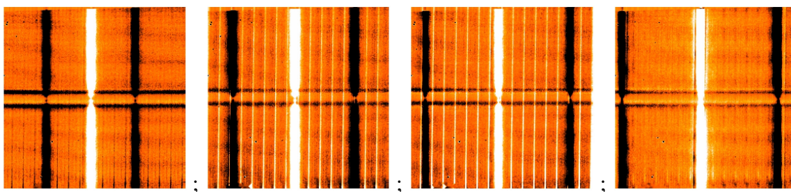
Figure 9: An example of the bad cosmetics on the old DRS detector. Sequence of chop/nod, reduced spectra obtained in the Medium Resolution mode with a central wavelength = 8.8\mu\text{m} . The TEL.CHOP.THROW = 8, 11, 13 and 14'' from left to right. Note the presence of significant striping when the ‘left’ beam hits some hot pixels at the lower left of the detector. For the location of the object along the slit (pixel X=123 at row Y = 128), this occurred for TEL.CHOP.THROW between 10 and 13'', approximatively. The horizontal lines at the middle of the images are caused by the lack of detector response at 8.8\mu\text{m} .
