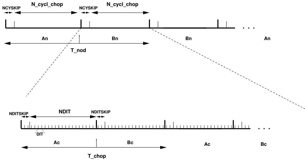
Figure 10: Data timing in VISIR. Ac and Bc refer to the two chopper positions, An and Bn refer to the two nodding (telescope) positions. Note the AnBnBnAn cycle sequence for the nodding to save observing time.
