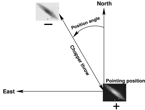
Figure 12: Definition of chopping parameters from the telescope point-of-view. If the position angle ( PA ) is measured counter-clockwise from North to East with PA between 0 and 360°, then TEL.CHOP.POSANG is 360^\circ - PA . The positive beam (+) is obtained when the M2 is at Chopping Position A and corresponds to the pointing position of the telescope as given in the FITS header (idle position). The negative beam (-) is obtained by moving the M2 so that it points to a position angle on the sky given by PA and a throw of TEL.CHOP.THROW from the telescope pointing position (Chopping Position B). If TEL.CHOP.POSANG = TEL.ROT.OFFANGLE = 360° - PA , the resulting image on the detector will appear as in one of the nodding position images illustrated in Fig. 14.
