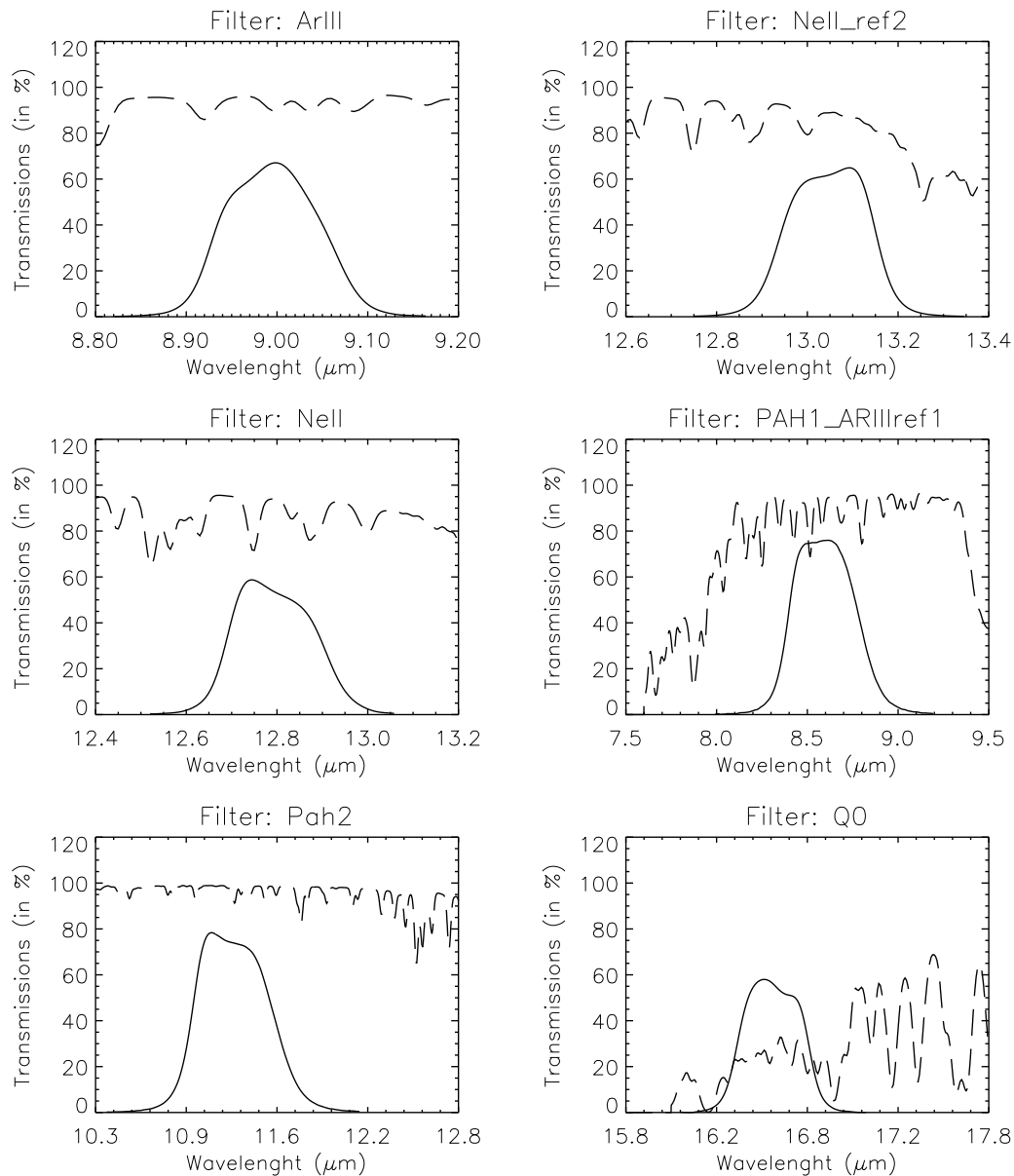
Figure 16: Transmission curves of VISIR imager filters, manufactured by READING. Overplotted (dashed) is the atmospheric transmission at low resolution. The absolute transmission values are given, expressed in percent.
