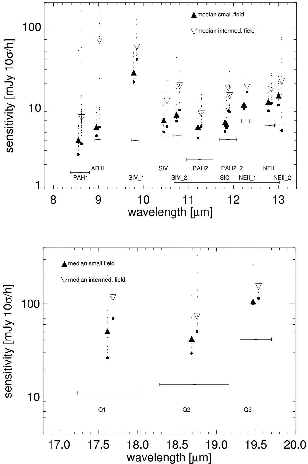
Figure 5: Measured on the old DRS detector but also valid for Period 90. Sensitivities for the VISIR imager for the N (top) and Q-band (bottom). Small and intermediate field observations are displaced for clarity. Background noise limits are indicated for the individual filter bandpasses.
