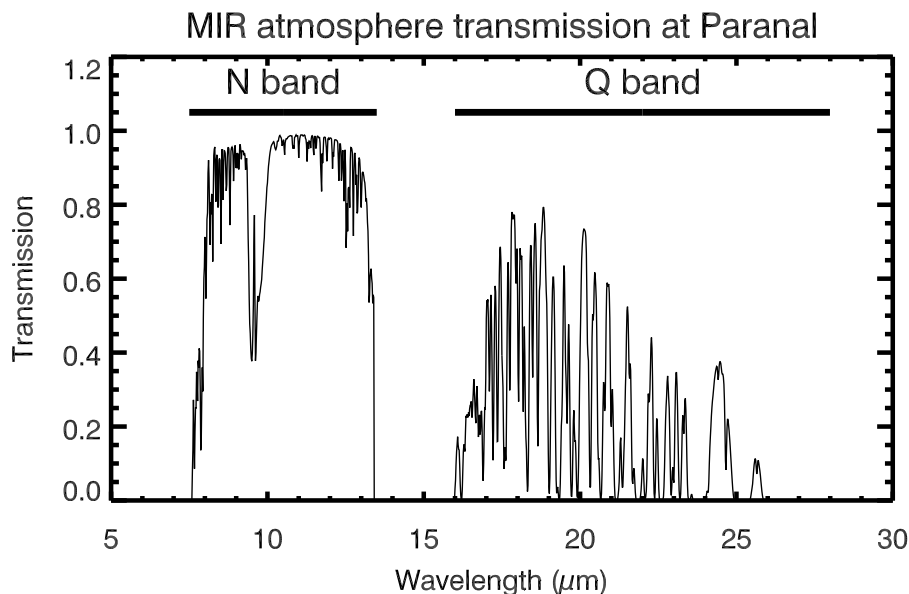
Figure 1: MIR atmospheric transmission at Paranal computed with HITRAN for an altitude of 2600 m and 1.5 mm of precipitable water vapor at zenith. The US standard model atmosphere is used.
