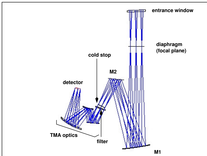
Figure 6: The optical path of the imager in the intermediate field (0'.076) is shown from the entrance window down to the detector.
