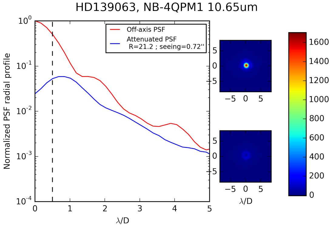
Figure 8: Coronagraphic (blue) PSF profile compared to the non-coronagraphic PSF profile for HD139063 observed during commissioning in 2015.
