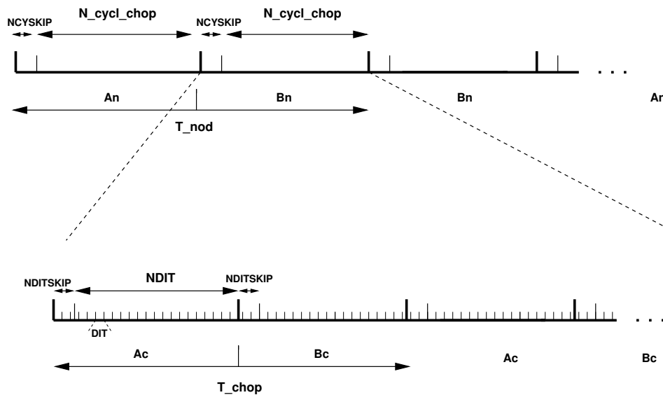
Figure 16: Data timing in VISIR. Ac and Bc refer to the two chopper positions, An and Bn refer to the two nodding (telescope) positions. Note the AnBnBnAn cycle sequence for the nodding to save observing time.
