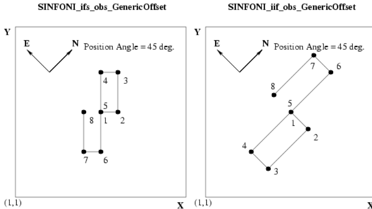
Figure 20: An illustration of the offset sequence taken with the GenericOffset template. Left side: Offset coordinate type "DETECTOR"; Right side: Offset coordinate type "SKY". This figure is meant to illustrate where on the detector the image of a point source is showing up, if the telescope is doing the offset sequence as specified for the parameters "List of offsets in RA or X" and "List of offsets in DEC or Y" in the above table, and if the source is centered on the detector at the start of the template.
