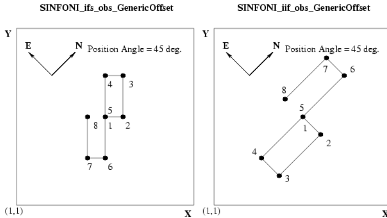
Figure 25: An illustration of the offset sequence taken with the GenericOffset template. Left side: Offset coordinate type “DETECTOR”; Right side: Offset coordinate type “SKY”. This figure is meant to illustrate where on the detector the image of a point source is showing up, if the telescope is doing the offset sequence as specified for the parameters “List of offsets in RA or X” and “List of offsets in DEC or Y” in the above table, and if the source is centered on the detector at the start of the template.
