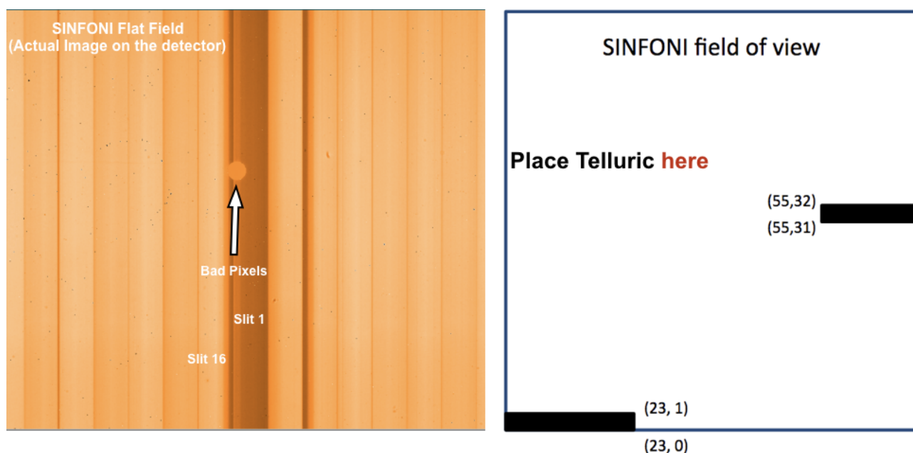
Figure 9: Left: This is a SINFONI Flat Field image. The disc of bad pixels near the centre of the detector mostly falls on slit #1, which crosses the centre of the field of view of SINFONI. Right: This is the reconstructed FOV of SINFONI, showing the location of the blind spots. Slit #16 corresponds to y=31 and 32 . Slit #1 corresponds to y=0 and 1 .
