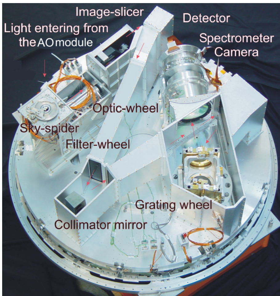
Figure 18: An inside view of SPIFFI: The cryostat cover and the reinforcing structure have been removed to provide a free view on the opto-mechanical components of SPIFFI. The light enters from the top, and passes the sky-spider. The pre-optics with a filter-wheel and interchangeable lenses provides three different image scales. The image slicer re-arranges the two-dimensional field into a pseudo-long slit, which is perpendicular to the base plate. Three diamond turned mirrors collimate the light onto the gratings. In total, four gratings are implemented on the grating drive. A multiple-lens system then focuses the spectra on a Rockwell HAWAII array. The diameter of the instrument is 1.3m.
