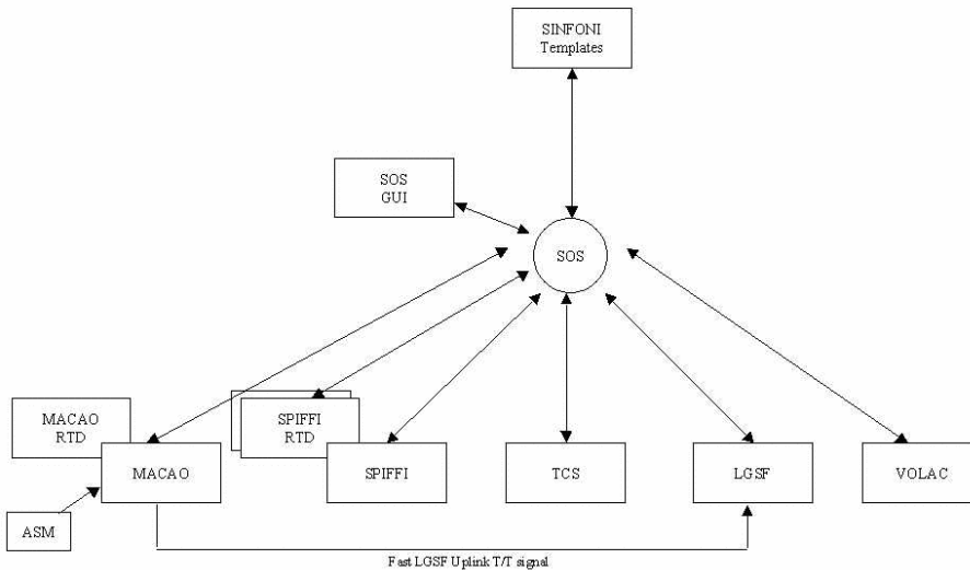
Figure 22: SINFONI software overview
