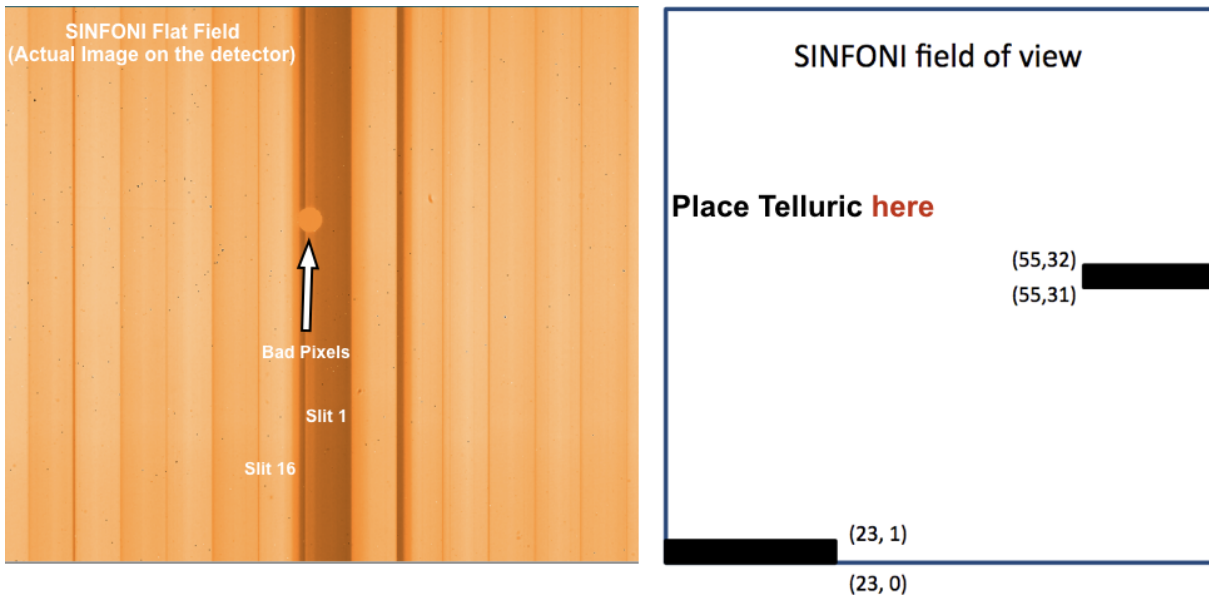
Figure 8: Left : This is a SINFONI Flat Field image. The disc of bad pixels near the centre of the detector mostly falls on slit #1, which crosses the centre of the field of view of SINFONI. Right : This is the reconstructed FOV of SINFONI, showing the location of the blind spots. Slit #16 corresponds to y=31 and 32 . Slit #1 corresponds to y=0 and 1 .
