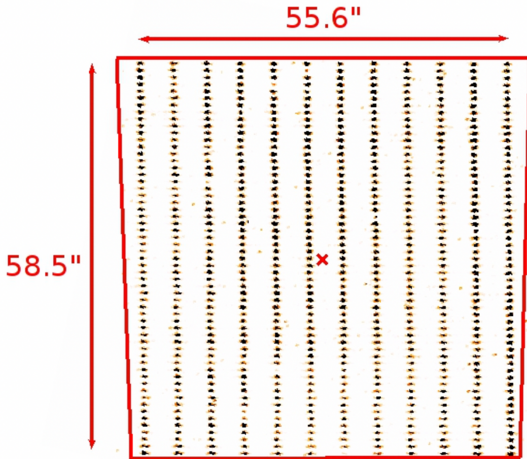
Figure 49: Arrangement of the WFM_SMP mask used for geometrical calibration, as viewed on a reconstructed image when illuminated with internal lamps. We overlay the trapezoidal shape of the FOV in red.
