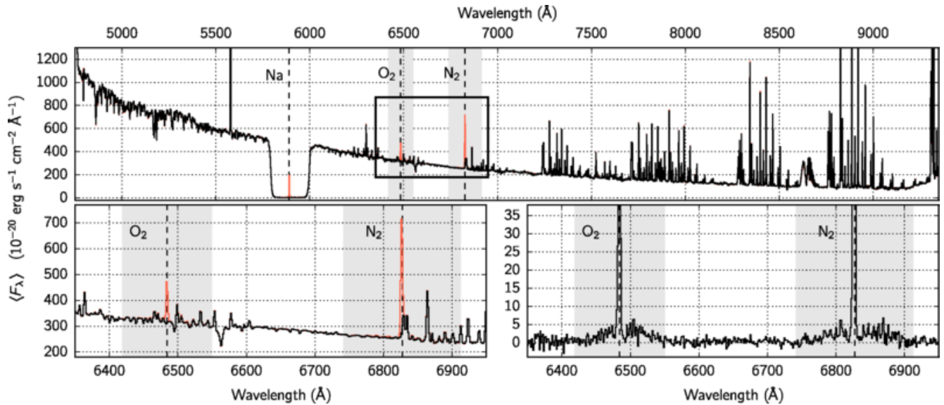
Figure 44: Sky spectrum seen by MUSE with 4LGSF on.
