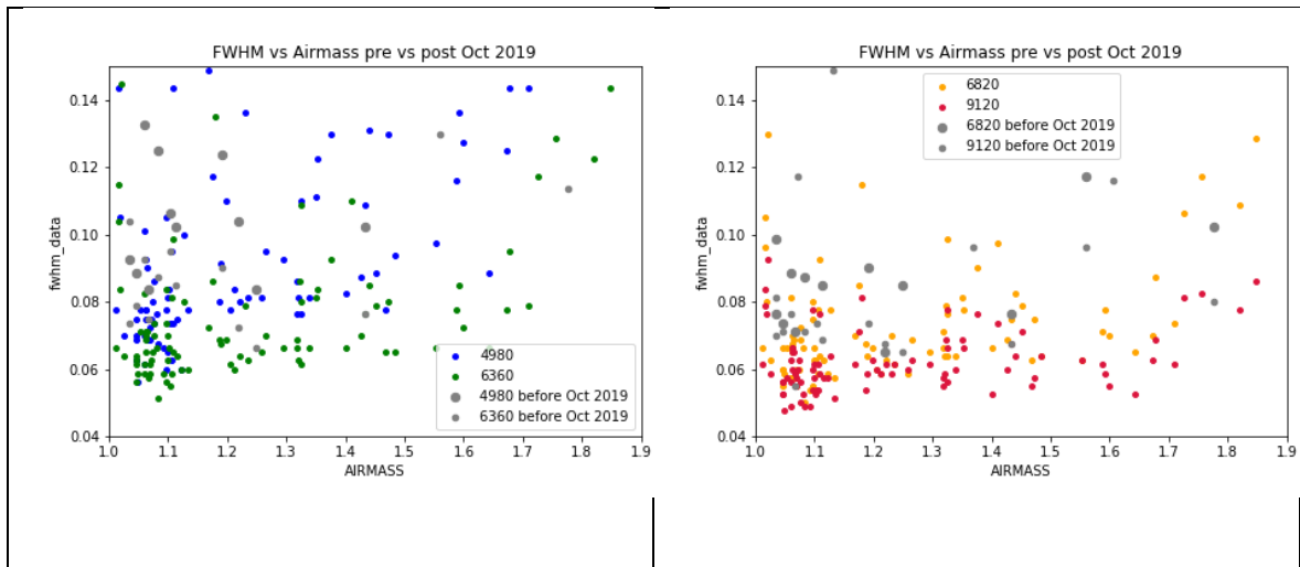
Figure 37 FWHM of the core of the NFM PSF for different airmasses before the 2019 campaign, grey, and after the campaign, in color, for selected wavelengths as indicated in the legends.
