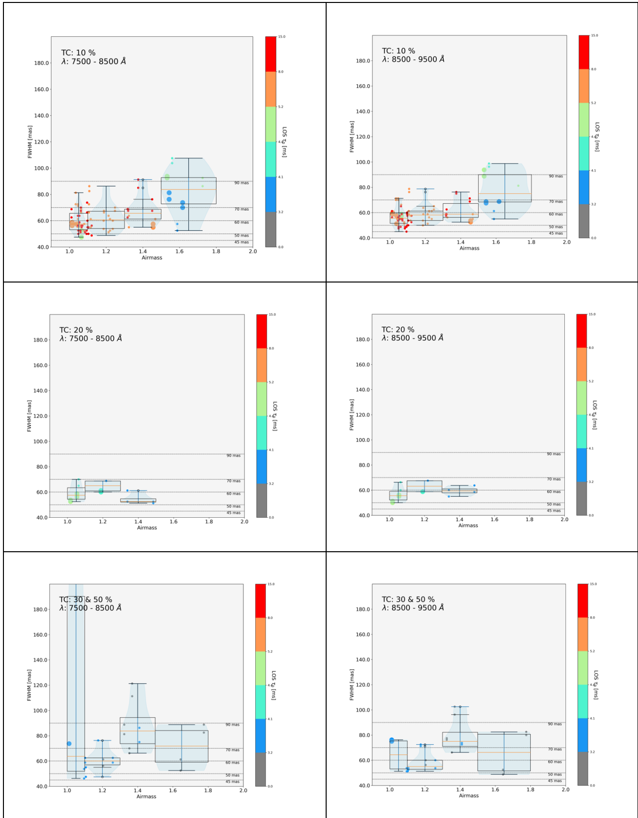
Figure 40 (cont) FWHM vs airmass for several TC and wavelength ranges. The colour bar gives the coherence time corrected to the airmass of observation.
