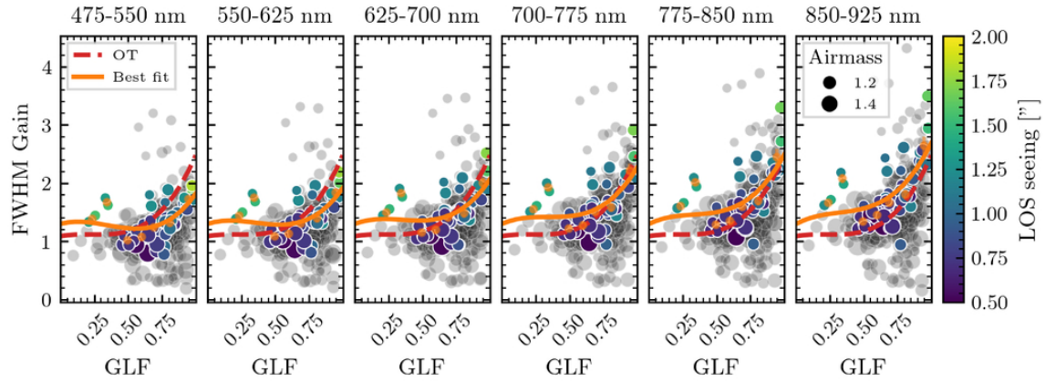
Figure 29 (top) Gain in image quality as function of GLF in six wavelength bins for observations in degraded mode (opaque points). For reference, operations in standard mode are shown with grey points, including poor data outliers (From Hartke et al. 2020).
