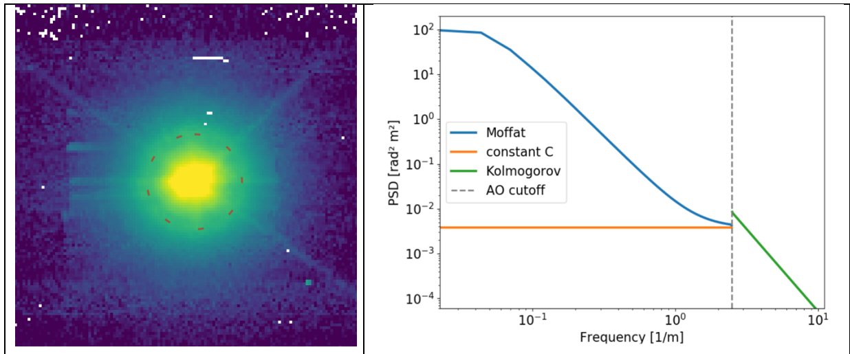
Figure 42 (left) MUSE NFM PSF for an image extracted between 889 - 935 nm. Red circle shows the AO cutoff of 0.432'' . Right, Fig 2 from Fétick et al. (2019) showing the maoppy PSF described in that paper.
