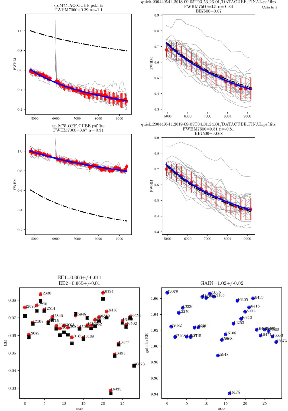
Figure 31: Performance of 3 lasers vs 4 lasers. (a, top) FWHM versus wavelength for all stars in one of the astrometric fields. The two left panels plots the data for 4 lasers with AO ON (top) and OFF (bottom); the two right panels show the performance with 4 (top) and 3 (bottom) lasers. (b, bottom) EE for 4 lasers (red circles) and 3 laser (black squares) and gain in EE for 4 vs 3 lasers. It should be noted that conditions were very stable during the observations that led to these figures. Even so, sometimes 3 lasers were ahead. External seeing conditions at the time \sim 0.90'' @ 550 nm.
