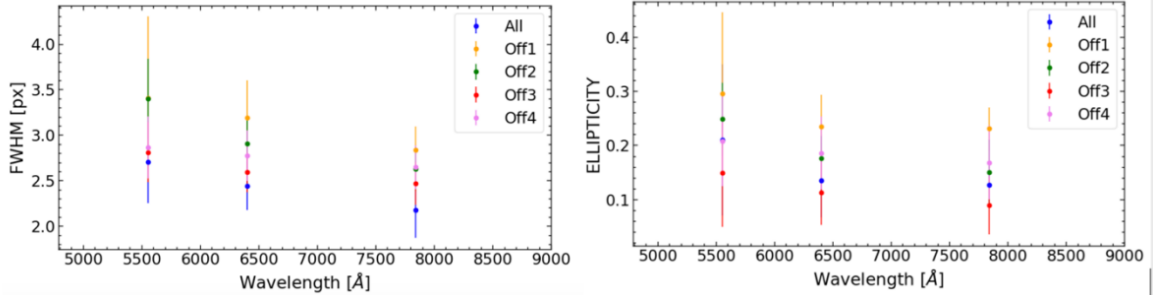
Figure 32: Distribution of the average of FWHM and ellipticity ( 1-B/A ) (right) as measured using the stars selected in the V, R and I MUSE field of view images. On the X-axis we adopted the nominal peak of the throughput of the filters. A and B are the lengths of the semi-major and semi-minor axes, respectively. The FWHM is measured in pixels. The label 'All' represents all four lasers are working, and label 'Off#' represents one of the lasers is turned off.
