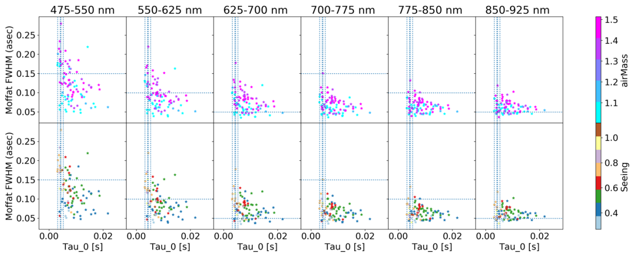
Figure 38 NFM FWHM in milli-arcsec [mas] from Moffat fits to the core of the PSF versus coherence time for six wavelength ranges. Data points are colour-coded according to the observed airmass (upper panels) and ambient seeing (lower panels). Note the strong airmass effect, especially for the bluer wavelengths. The horizontal lines are drawn at 150 mas, 100 mas, and 50 mas.
