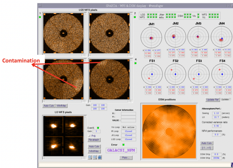
Figure 43 4LSF FoV contamination by bright star as seen in the SPARTA GUI.
