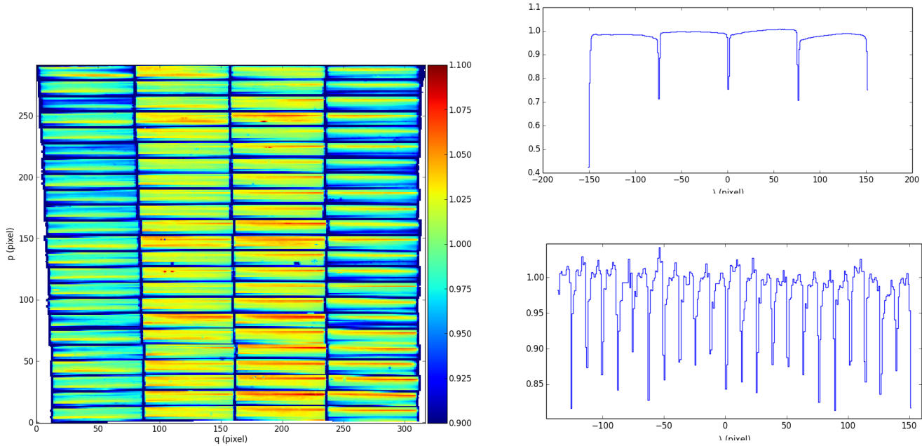
Figure 19: (left) normalized reconstructed image of the continuum flat-field in WFM. (right) horizontal (top) and vertical (bottom) cuts through the normalized image showing the horizontal and vertical variations in illumination.
