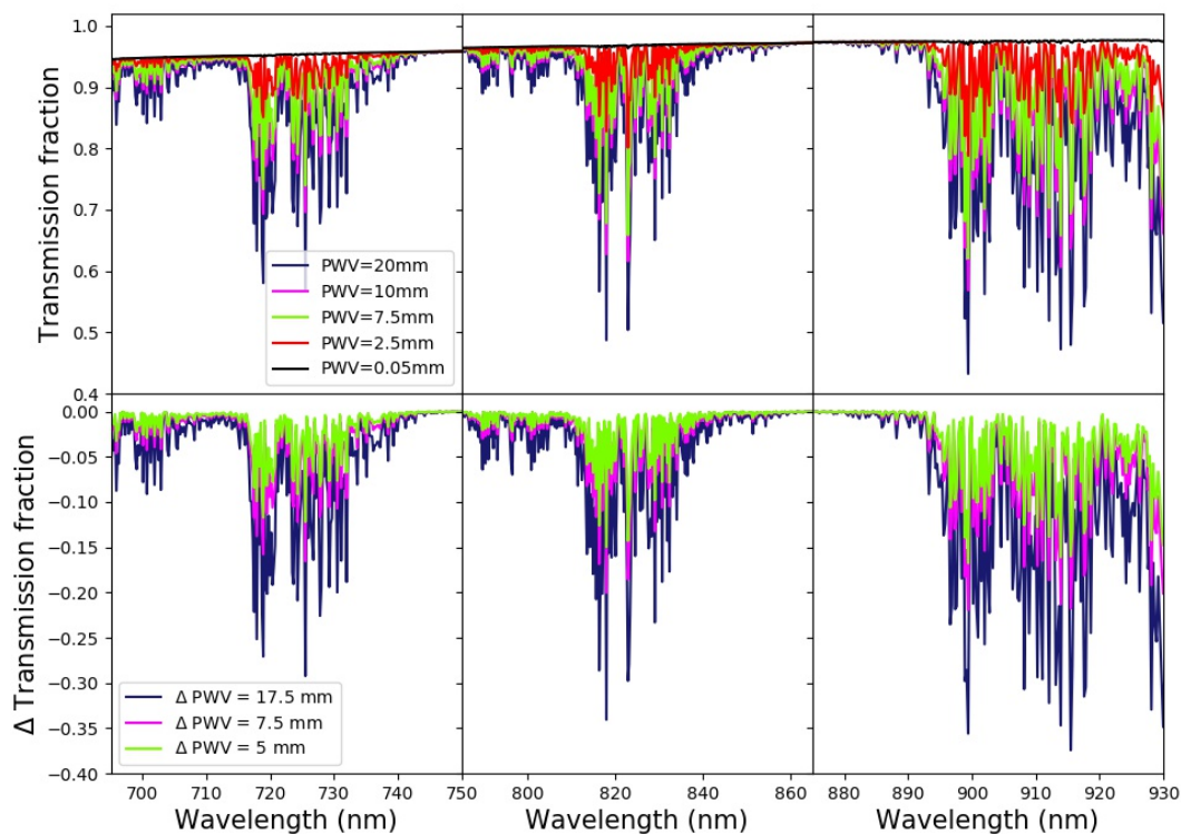
Figure 48 Water vapour telluric absorption. The top panels show the fractional atmospheric transmission as a function of wavelength for several values of PWV, while the bottom panels show for each PWV the absorption difference from the median Paranal value absorption at 2.5 mm of H 2 O.
