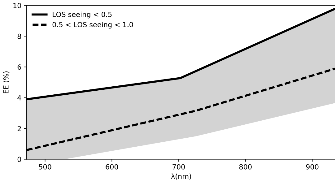
Figure 36: Ensquared Energy (EE) in a 25mas (one spaxel) box as a function of wavelength. As in Figure 35, the continuous line shows the best performance for a LOS seeing < 0.5". The dashed line shows the median performance and the grey area indicates the range observed during the commissioning runs for a LOS seeing between 0.5 and 1 arcsec.
