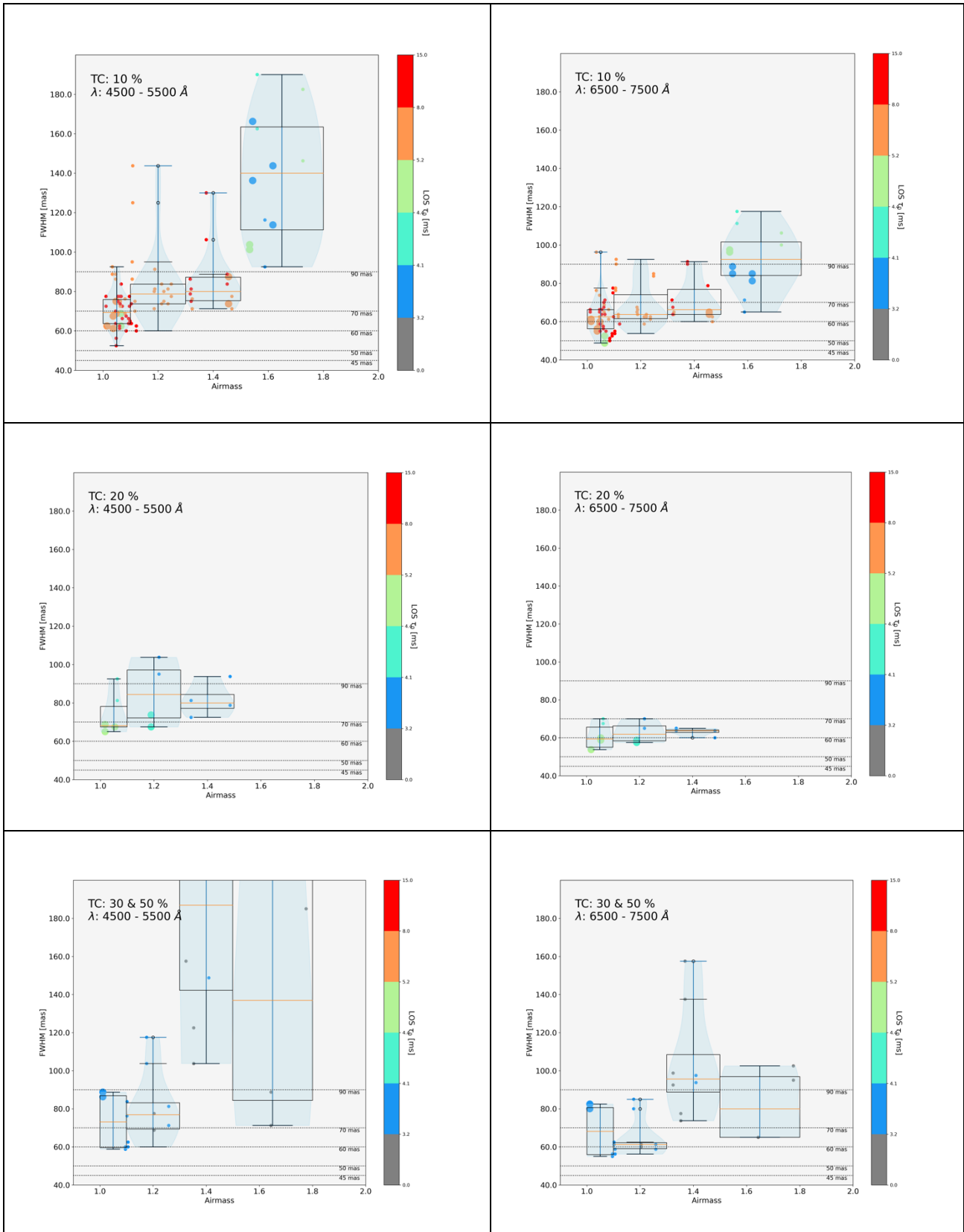
Figure 39 FWHM vs airmass for several TC and wavelength ranges. The colour bar gives the coherence time corrected to the airmass of observation.
