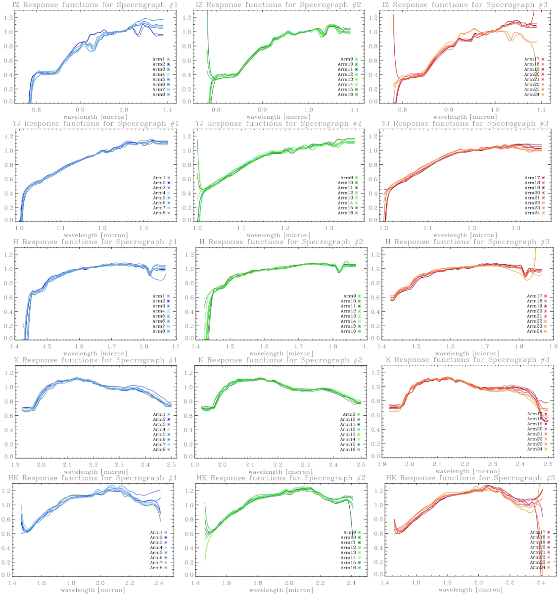
Figure 24: Response function as a function of wavelength obtained per arm and per grating. Ordinates are in arbitrary units.
