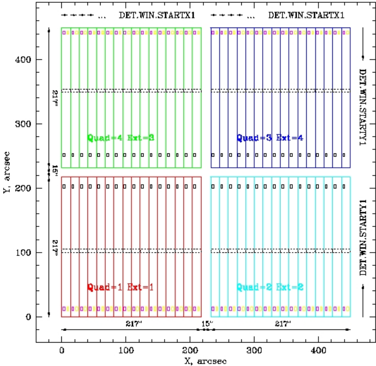
Figure 22: Definition of the windows. The location of the four HAWK-I detectors on the focal plane is shown, as well as the 16 stripes in which each detector is being read. The sizes of the detectors and the gaps, projected on the sky in arc-secs are also given. The binaries generated from quadrants 1, 2, 3, and 4 are usually (but not always) stored in fits extensions 1, 2, 4, and 3. Arrows indicate the direction in which the parameters DET.WIN.STARTX, DET.WIN.STARTY, DET.WIN.NX and DET.WIN.NY increase. Note, that the parameter DET.WIN.STARTX defines the starting point of the window, counted from the beginning of each detector stripe, not from the beginning of the detector. All these parameters are defined in pixels, although this figure is plotted in arc-secs. As examples, four different sets of windows are shown in violet, yellow, solid and dashed black lines.
