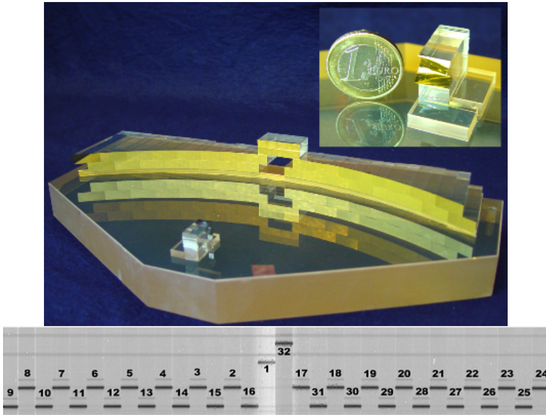
Figure 12: Top: SPIFFIER image slicer (a): The light enters through the hole in the big slicer. A stack of 32 small mirrors, the small slicer (also shown in the sub-panel), slices the image and redirects the light to-wards the 32 mirrors of the big slicer, which re-arranges the slitlets into a 31 cm long pseudo-slit. Bottom: Illustration of the slitlet layout in raw SPIFFIER images, light is dispersed vertically on the science detector.
