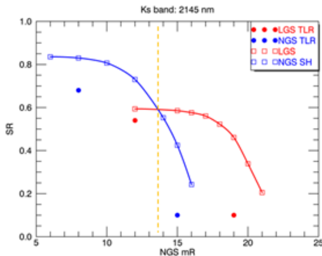
Figure 17: The SR in K band as a function of the reference star magnitude in R band for NGS and LGS case. SR values are given on the y-axis in this plot.
