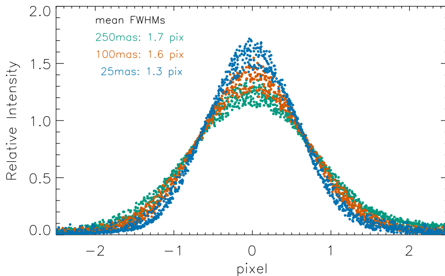
Figure 30: Fine sampled SPIFFIER line profiles in all grating configurations and pixel scales.
