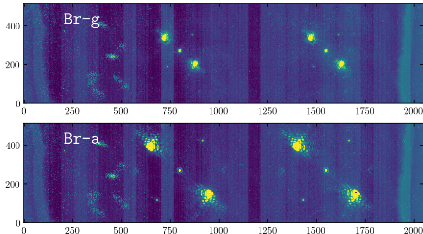
Figure 31: A composite image of the acquisition position for APP observations (800, 1536), and the recommended offset position at (1550, 1550) within the recommended window4 sub-array for K -band (top) and L -band (bottom).
