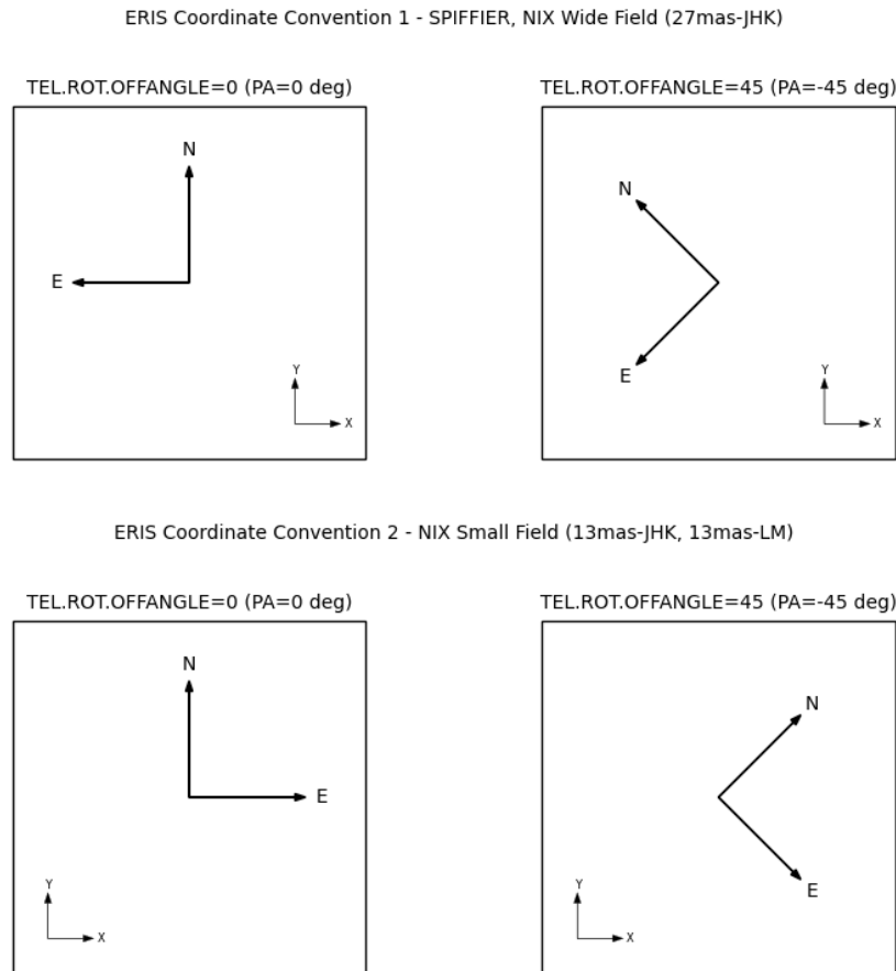
Figure 32: Coordinate system definitions for ERIS.
