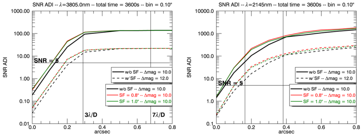
Figure 23: The SNR for L' (left) and K band (right) computed with numerical simulations when AO corrected images are combined by using ADI technique. The SNR saturates quickly in the L' case because of the large contribution from sky background.
