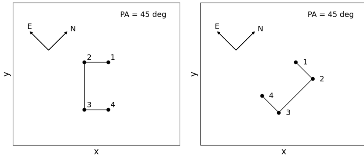
Figure 33: An illustration of the offset sequence for a point source with the on-sky position angle of 45 deg taken with the ERIS_ifs_obs_GenericOffset template. Left side: Offset coordinate type DETECTOR ; Right side: Offset coordinate type SKY . This figure is meant to illustrate where on the detector the image of a point source is showing up, if the telescope is doing the following offset sequence: (0, +1, 0, -1) in x or RA and (0, 0, +2, 0) in y or DEC. The numbers illustrate the order of the offsets.
