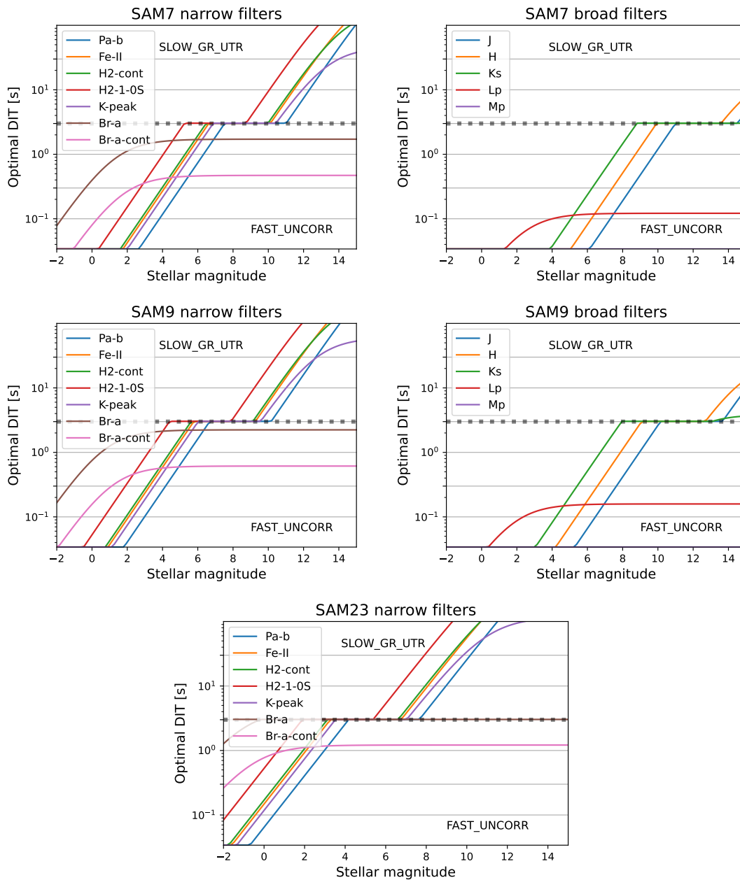
Figure 29: Optimal DIT used in combination with each SAM mask and each filter as a function of stellar magnitude of the target. These values were derived from the ERIS ETC.
