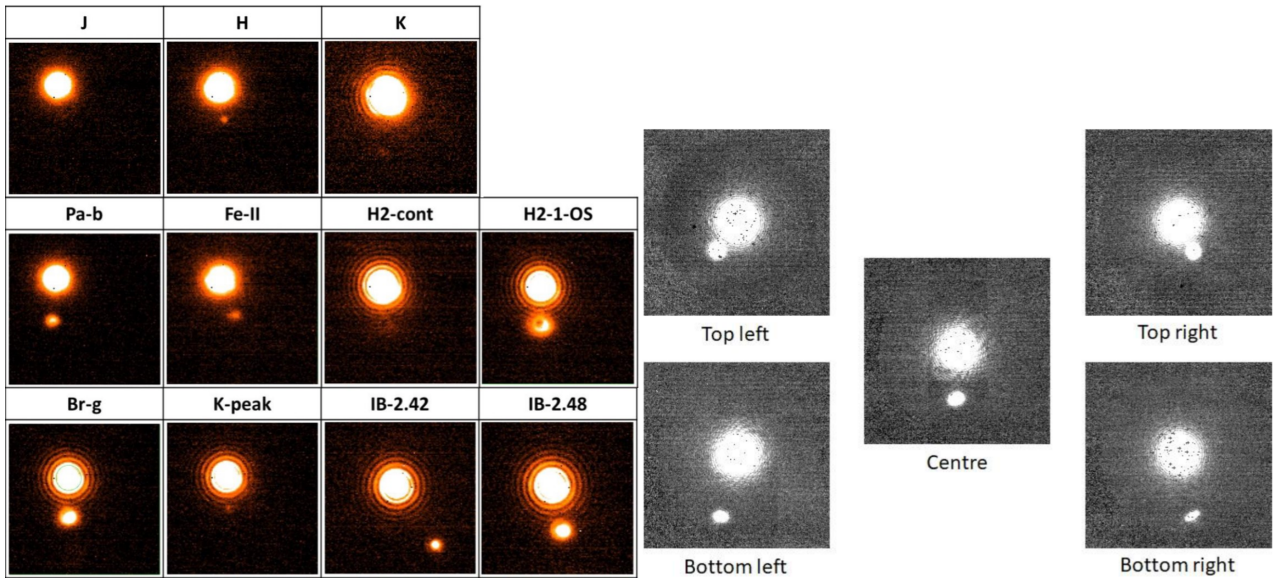
Figure 25: (left panel) Relative positions and strengths of ghosts in the centre of the field. (right panel) Dependency of relative ghost position on location in field, illustrated with the Pa-b filter.
