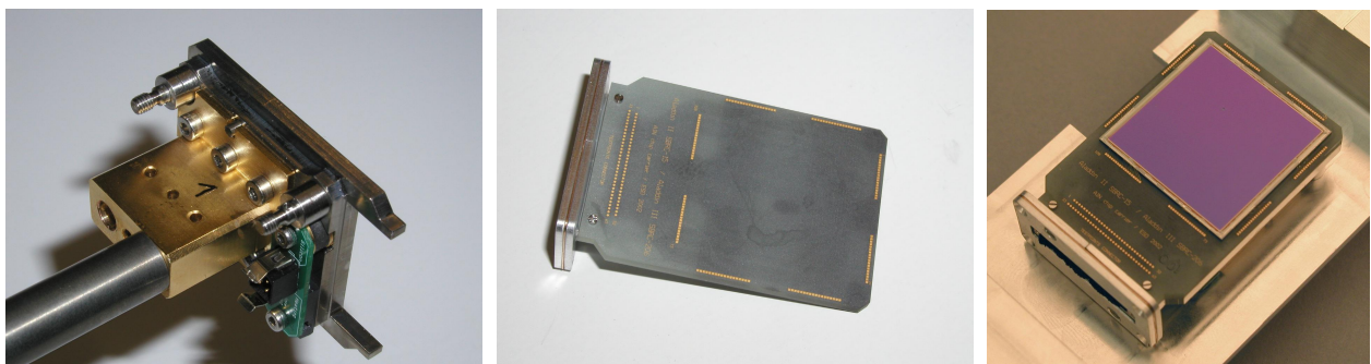
Figure 2 Pictures of the invar baseplate with the copperblock, the 8 layer AlN ceramics and the final mounted Aladdin device
