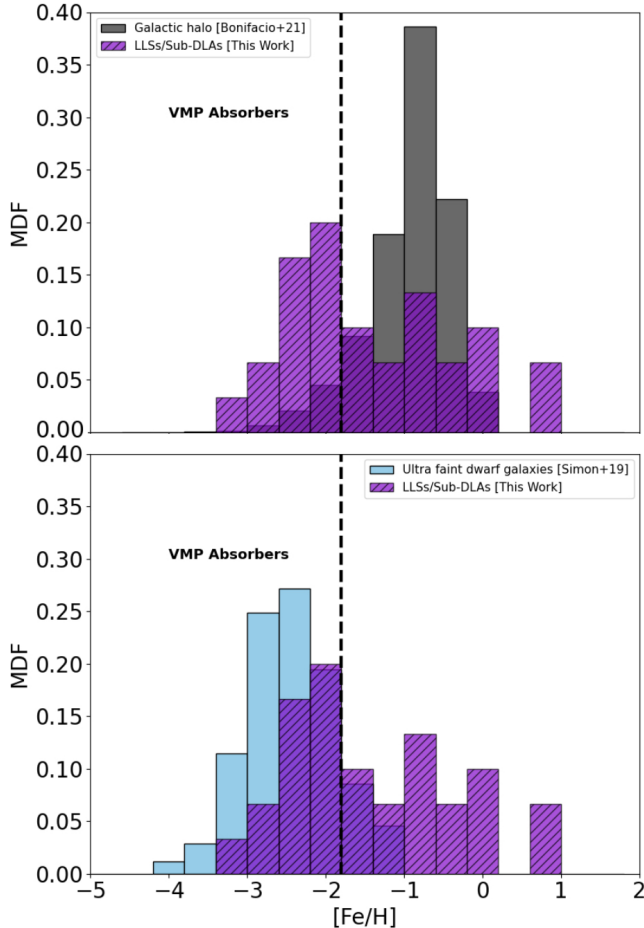
Figure 2. Comparison between the Metallicity distribution functions (MDFs) of our 30 absorbers, assuming Cayrel’s relative abundances in the photoionization model, and the MDF of \sim 140000 stars in the Galactic halo (Bonifacio et al. 2021) (top panel) and of 350 stars in 26 UFDs (Simon 2019) (bottom panel). A dashed line at [\text{Fe}/\text{H}] = -1.8 separates the very metal-poor (VMP) absorbers from the others.
