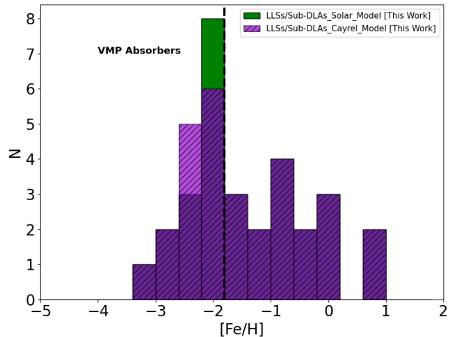
Figure 1. Metallicity distribution function (MDF) of our 30 absorbers assuming solar relative abundances (green) and Cayrel’s relative abundances (purple) in the photoionization model. A dashed line at [\text{Fe}/\text{H}] = -1.8 separates the very metal-poor (VMP) absorbers from the others.
