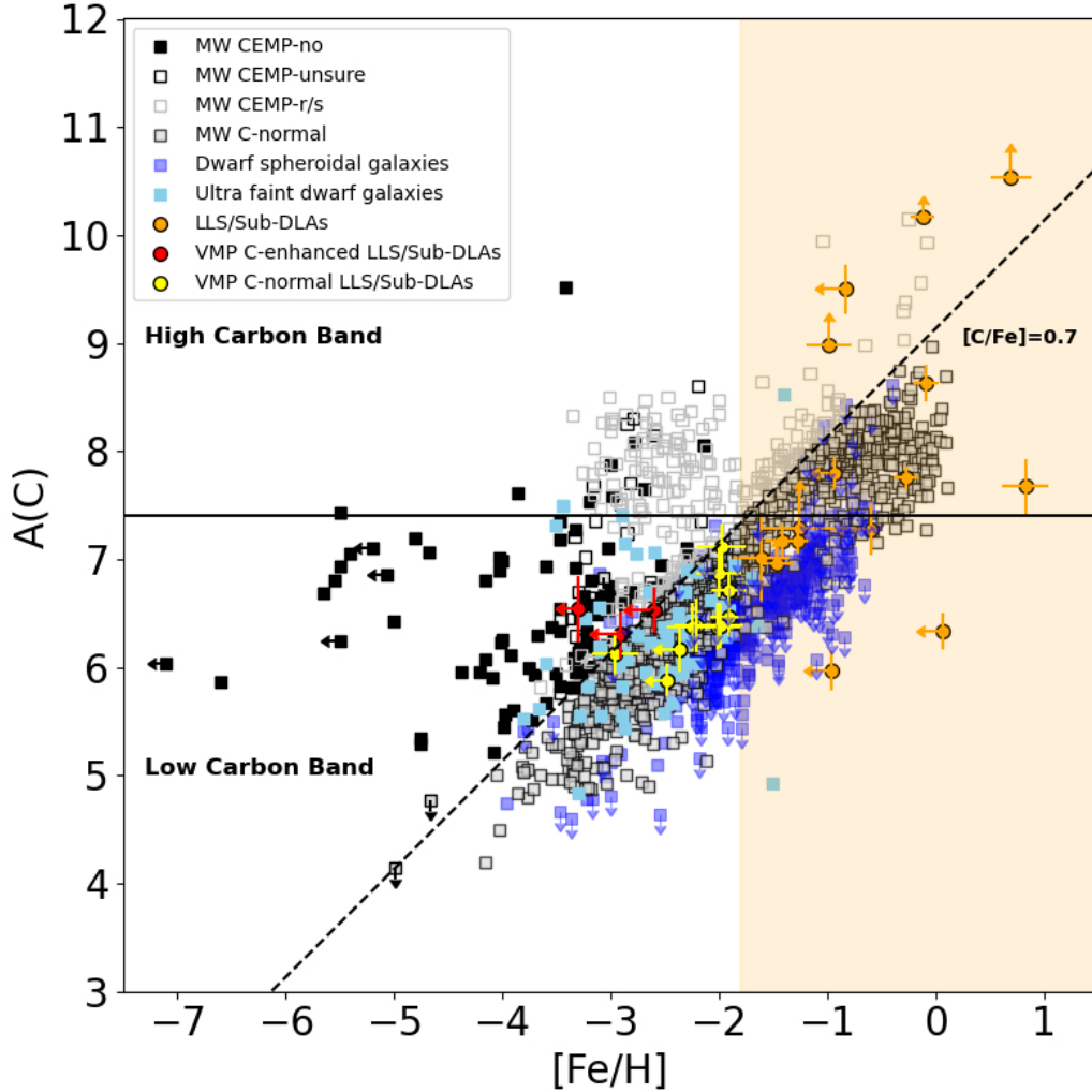
Figure 5. Absolute carbon abundance ( A(C) ) as a function of [Fe/H] of all our gaseous absorption systems (filled circles) and of stars in ultra-faint dwarf galaxies (light blue squares), dwarf spheroidal galaxies (blue squares) and the Milky Way (grey/black squares). CEMP-no halo stars are shown as filled black symbols, C-normal halo stars as filled bordered light grey squares and open symbols are CEMP-s/r stars. We distinguish among C-enhanced (red) and C-normal (yellow) very metal-poor absorbers. Orange circles are iron-rich absorbers. Stellar measurements have typical 1\sigma errors of 0.2 dex. We used the same stellar sample of Fig. 4 (upper left panel). The horizontal line separates the low-C from the high-C band, while the dashed one indicates the value [C/Fe]=+0.7 . The orange shaded area identifies the region where chemical abundances could be affected by dust depletion.
