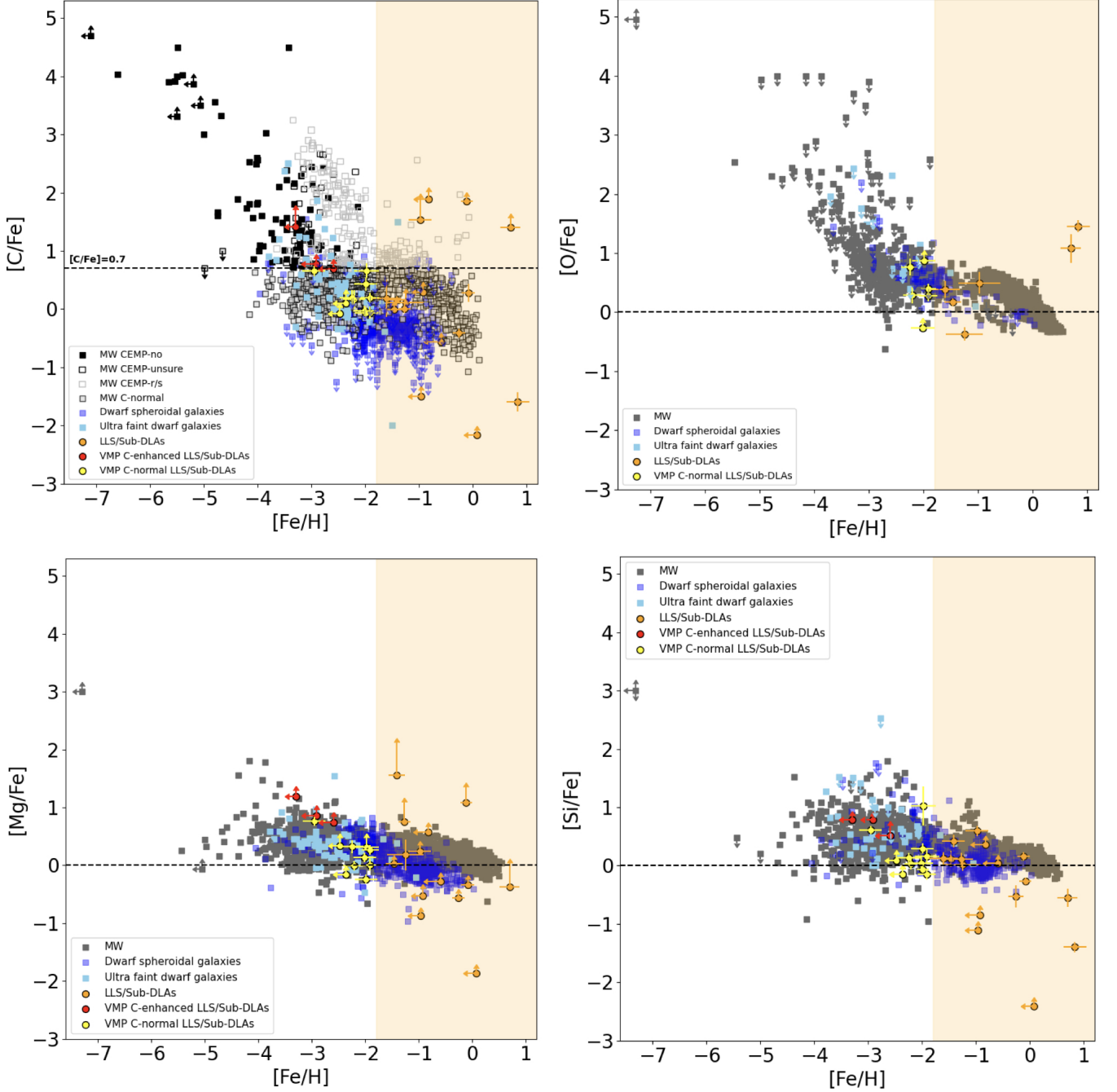
Figure 4. Upper left panel: carbon-to-iron ratio as a function of [\text{Fe}/\text{H}] of all our gaseous absorption systems (filled circles) and of stars in ultra-faint dwarf galaxies (light blue squares), dwarf spheroidal galaxies (blue squares) and the Milky Way (grey/black squares). CEMP-no halo stars are shown as filled black symbols, C-normal halo stars as filled bordered light grey squares and open symbols are CEMP-s/r stars. Stellar measurements have typical 1\sigma errors of 0.2 dex. We distinguish among C-enhanced (red) and C-normal (yellow) very metal-poor absorbers. Orange circles are iron-rich absorbers. Other panels: Comparison between the chemical abundances of the very metal-poor gaseous absorption systems (circles) and of the stars (squares) in the Milky Way (grey), ultra-faint dwarf galaxies (light blue) and dwarf spheroidal galaxies (blue). Red and yellow circles are respectively C-enhanced and C-normal, very metal-poor absorbers. Orange circles are iron-rich absorbers. Stellar data are taken from the SAGA database (Suda et al. 2008). In all the panels the orange shaded area identifies the region where chemical abundances could be affected by dust depletion.
