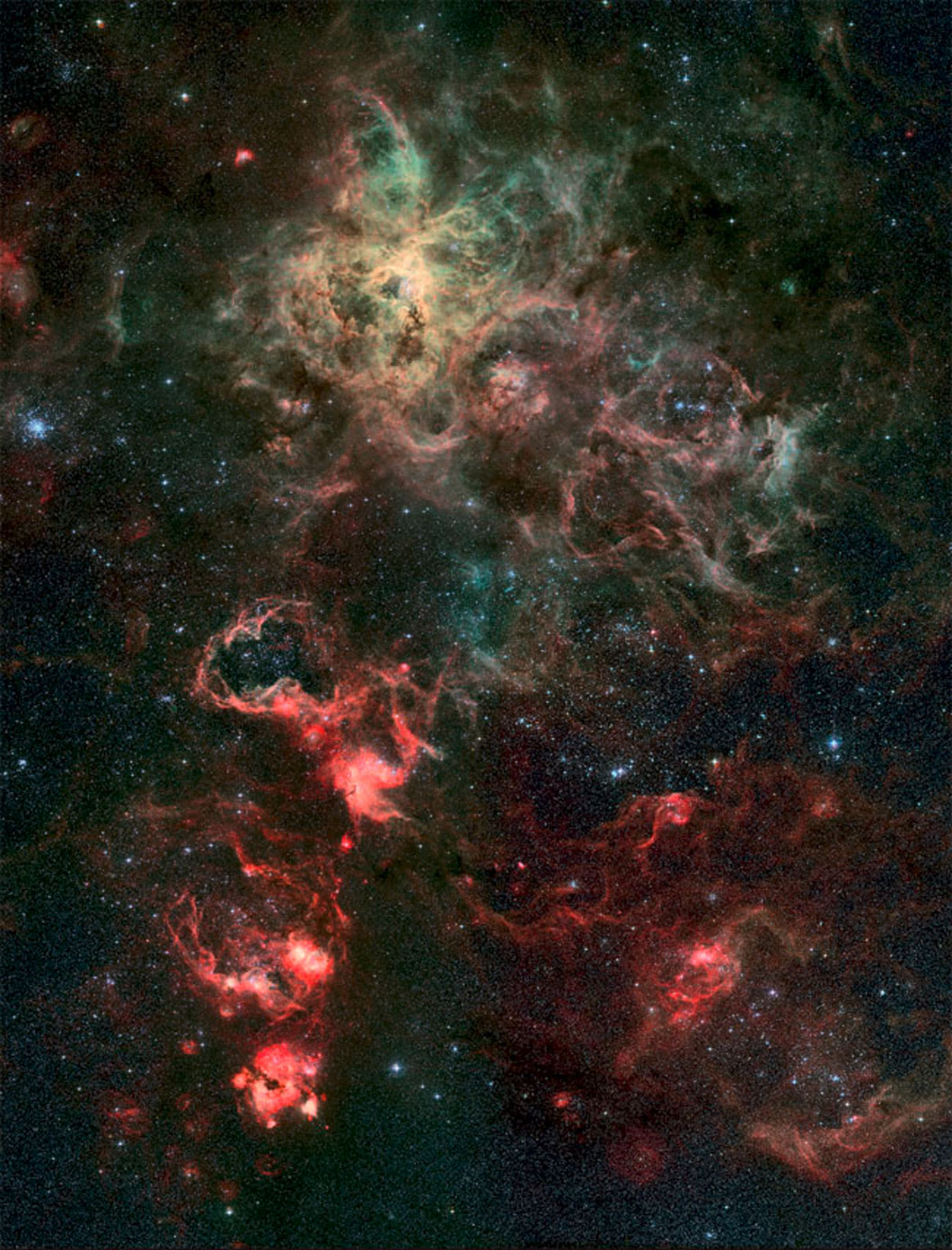
The Tarantula Nebula (WFI/2.2-m)
