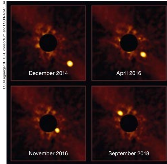
Figure 1. SPHERE images at different epochs of the giant exoplanet \beta Pictoris b (left) and of arch-like disc features in the debris disc of AU Microscopii (bottom). High-precision relative astrometry is fundamental to measuring the slow motions observed, from south-west to north-east for the planet and away from the star for the disc features. In the bottom panel, the scale bar at the top of the picture indicates the diameter of the orbit of the planet Neptune in the Solar System.
