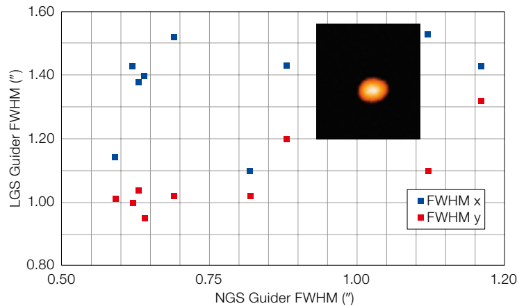
Figure 3. The laser guide star spot size versus the natural guide star (NGS) image full width half maximum (FWHM) measured by the telescope guider. The two values of FWHM are plotted separately.
