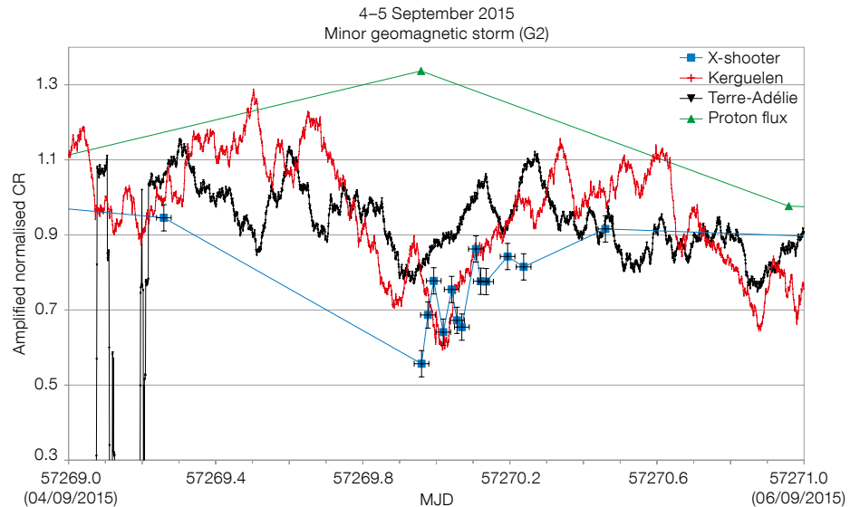
Figure 1. Relative evolution of the cosmic ray rate during the minor geomagnetic storm of 4–5 September 2015. The x-axis gives the Modified Julian Day (time) and the y-axis corresponds to the relative CR rates. The X-shooter (blue squares), Kerguelen Islands (red), Terre-Adélie (black) CR rates all show first a decrease then a return to the normal level once the solar wind intensity is back to normal (Forbush effect). The density of protons carried out by the fast dense solar wind, which causes the storm, is shown in green.
