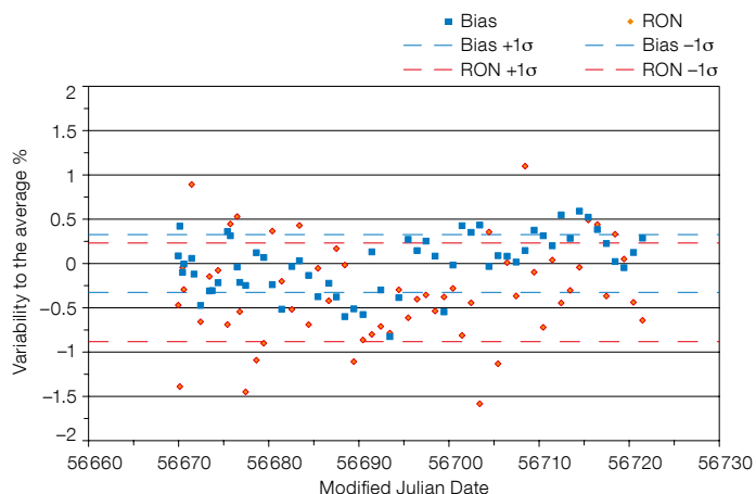
Figure 1. X-shooter AGCCD variability (or relative difference) in the bias level (blue squares) and RON level (orange diamonds) in % from the average with time are plotted. For each of the curves the \pm 1\sigma spread is shown.
