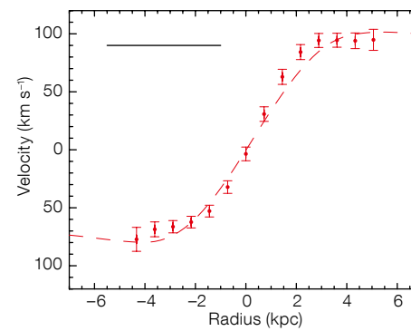
Figure 3. Left: Position-velocity diagram along the major axis of the disc model with our best fit rotating disc model overlaid as contours. Centre: Rotation curve extracted along the major axis with our best-fit model overplotted as a dashed line. Right: The variation in velocity dispersion as a function of radius in the disc. The low V/\sigma \sim 3 value shows this is a
