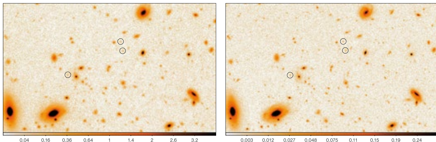
Figure 2. The centre of the deepest GOODS-S field as observed with HAWK-I is shown in the K -band (left) and with WFC3/IR in the H -band (right). The displayed area is 1 arcminute wide. Objects circled have H \approx 26 mag and a colour ( H - K ) \approx 0.5 , typical of faint galaxies.
