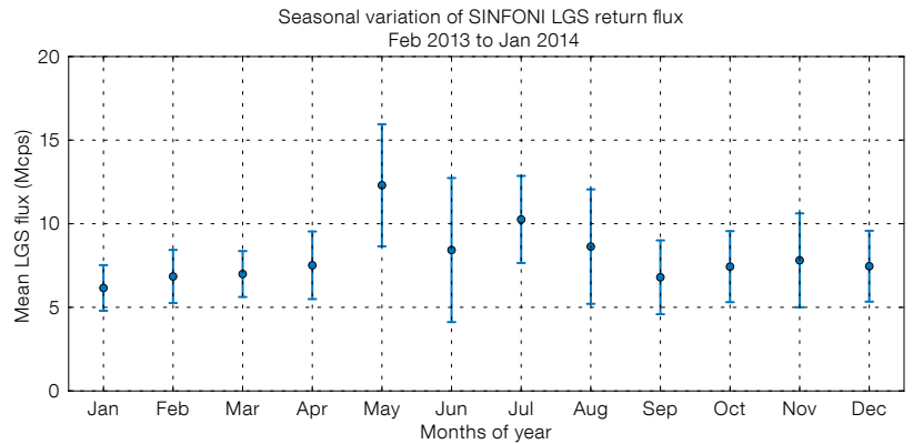
Figure 9. Monthly means and standard deviations of the counts, recorded by the SINFONI wavefront sensor, for the laser guide stars over the period of the upgraded LGSF.
