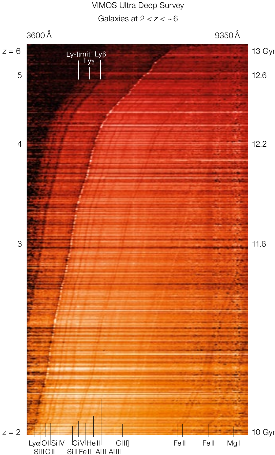
Figure 3. Stacked display of VUDS spectra between redshift 2 and \sim 6 (left-hand axis), covering between \sim 10 and 13 billion years back into the history of the Universe (right-hand axis). Prominent absorption and emission lines and the Lyman limit are indicated.
