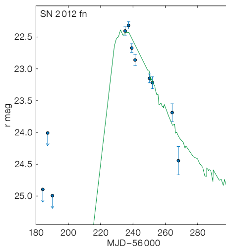
Figure 4. Light curve and spectrum of SN 2012fn, a Type Ic at z = 0.28 discovered by SUDARE. The green spectrum is the best-fit template obtained by GELATO.
