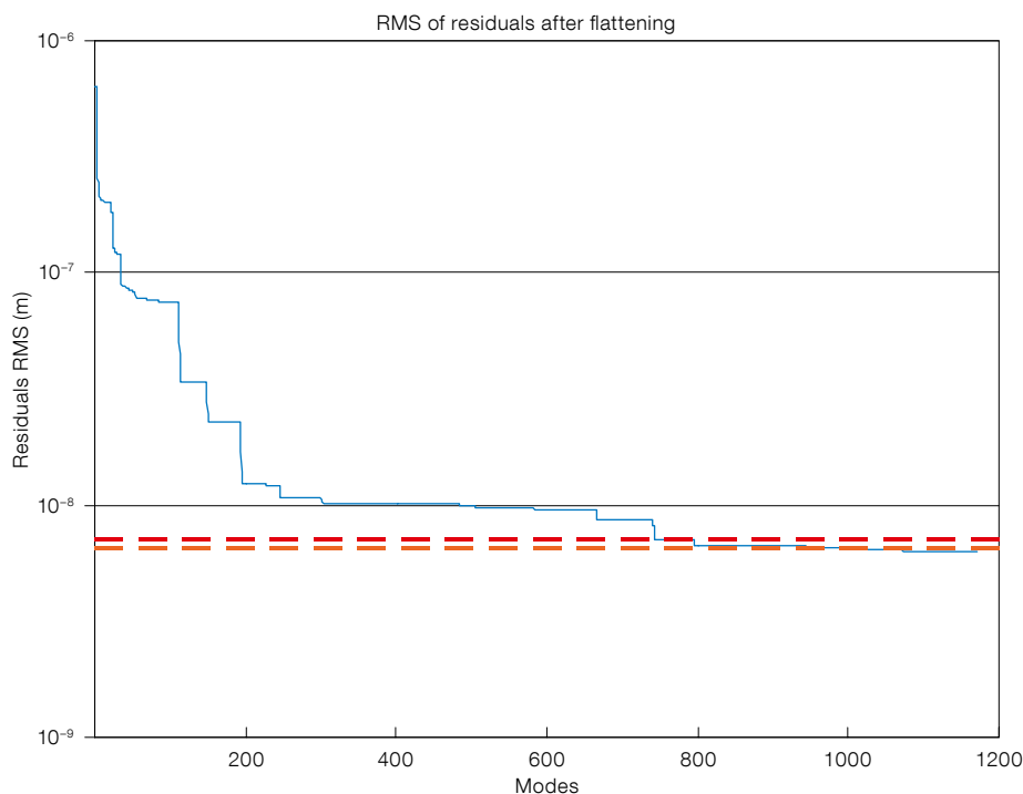
Figure 4. The simulated convex shape of the DSM after correction; showing the surface error residuals (rms) in metres versus the number of modes used to achieve the correction.
