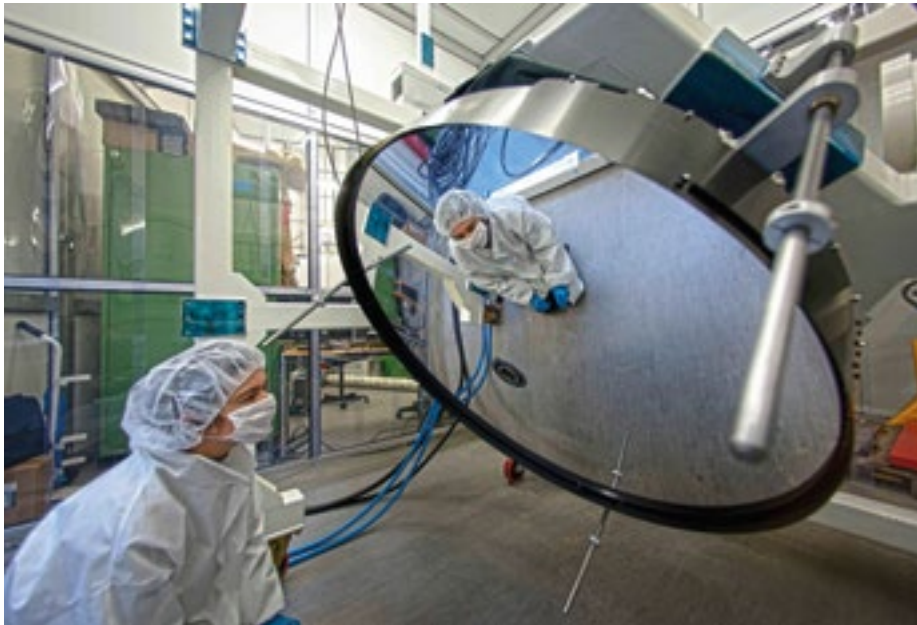
Figure 1. The deformable secondary mirror in its test stand. In operation the thin-shell mirror is held by the actuators with a gap of 65\ \mu\text{m} between the shell back face and the reference body front face. The black metallic structure surrounding the mirror is called the "EMC skirt" and shields the system from electromagnetic interference.
