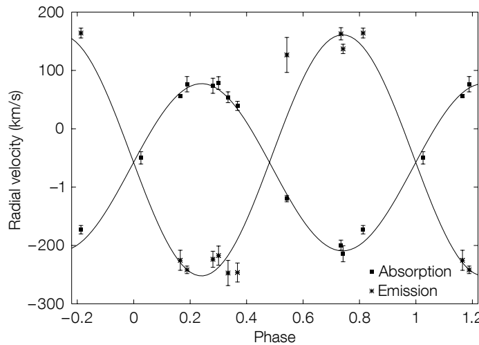
Figure 6. Radial velocity curve for both components of the WNL+OB binary Wd1-13 folded on the \sim 9.27 -day orbital period.
