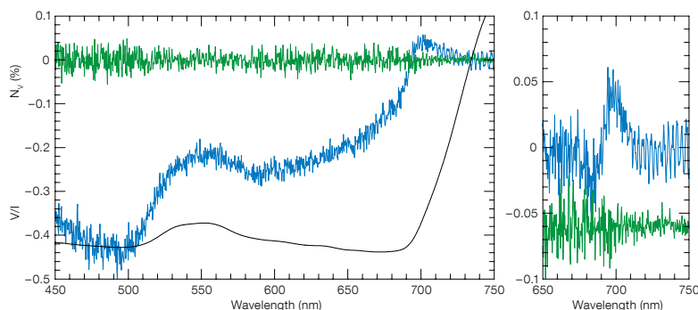
Figure 2. The Philodendron leaf is shown at left and its polarised spectrum measured with EFOSC2 at middle and right. The blue lines show the circular polarisation ( V/I ). In the rightmost panel, V/I is rectified to zero. The green lines show the null profile (offset by -0.06\% in the rightmost panel, for display purposes) demonstrating the statistical errors. The black line is the reflectivity (in arbitrary units).
