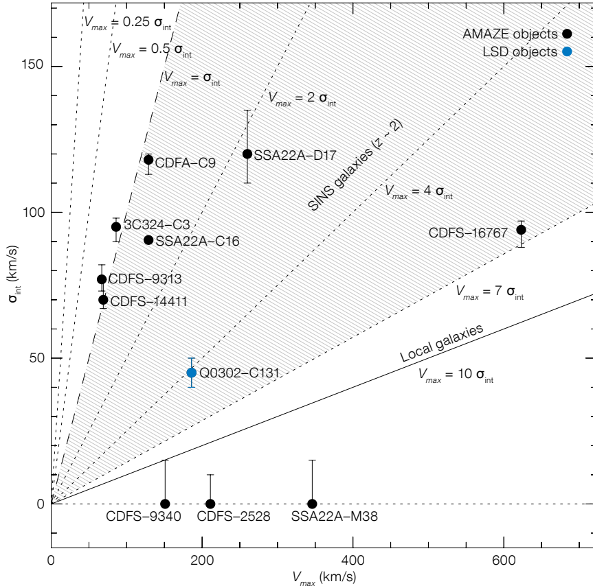
Figure 4. Velocity dispersion ( \sigma ) versus rotational velocity ( V_{\max} ) is shown for disc galaxies at z \sim 3.3 with a regular rotation pattern. The solid line shows the relation V_{\max}/\sigma = 10 typical of local galaxies. Note that discs at z \sim 3.3 are much more turbulent than local galaxies, many of them having V_{\max}/\sigma \sim 1 . From Gnerucci et al. (2010).
