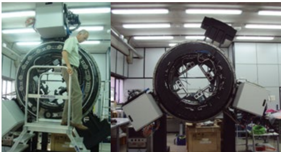
Figure 3. GRAAL's main structure is shown being integrated and tested at NTE SENER S.A. in Spain.
