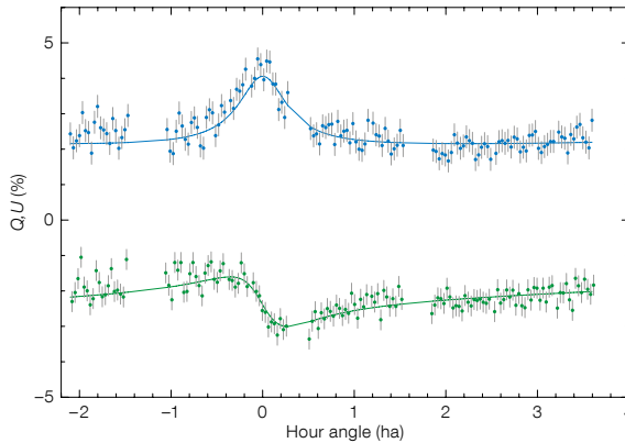
Figure 3. Stokes Q (in blue) and U (in green) parameters as a function of hour angle for IRS16C (linear polarisation 4.6% at PA18°, m_k = 9.55 ). The solid line is the best \chi^2 -fit of the model and the points represent observations from 2009. The fitting confirms the time dependency of the instrumental polarisation as predicted by the model and additionally allows the apparent polarisation of this star to be determined.
