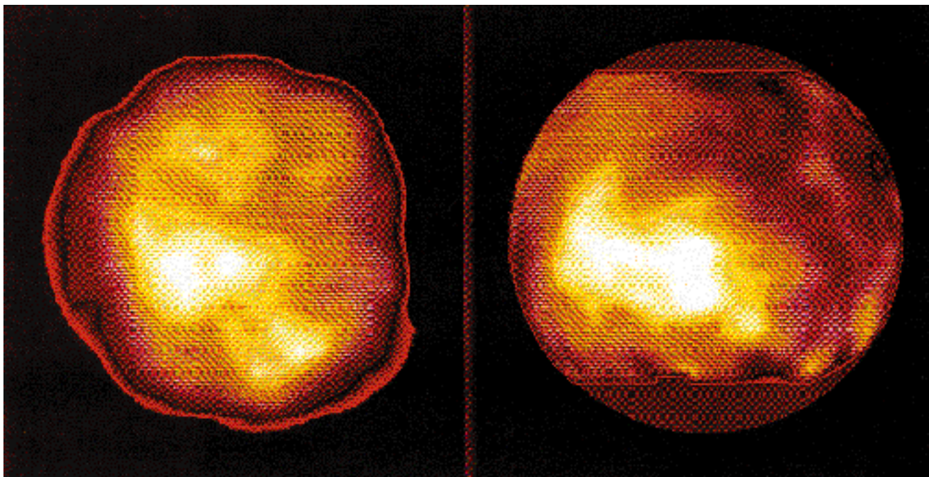
Figure 4: Titan's surface: ADONIS image at 2 micron on the left and Hubble Space Telescope image near 1 micron to the right. The central equatorial bright spot is observed on both, as well as indication of additional features near the limbs. The spatial resolution is similar, the contrast is about 3 times higher in the adaptive optics image.
