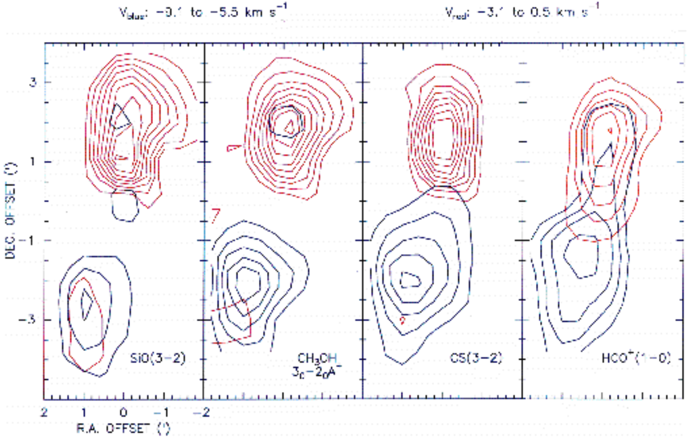
Figure 4. Contour maps of velocity integrated line wing emission from the Sandqvist 136 bipolar outflow. Blue contours correspond to the emission integrated in the velocity range from -9.1 to -5.5 \text{km s}^{-1} (blueshifted wing) and red contours to the integrated emission in the velocity range from -3.1 to 0.5 \text{km s}^{-1} (redshifted wing). The lowest contour and contour interval are, respectively, 0.1 and 0.1 \text{K km s}^{-1} for the \text{SiO}(J=3 \rightarrow 2) line (left), 0.3 and 0.3 \text{K km s}^{-1} for the \text{CH}_3\text{OH}(3_0 \rightarrow 2_0)\text{A}^+ line (middle-left), 0.2 and 0.15 \text{K km s}^{-1} for the \text{CS}(J=3 \rightarrow 2) line (middle-right), and 0.4 and 0.3 \text{K km s}^{-1} for the \text{HCO}^+(J=1 \rightarrow 0) line (right).
