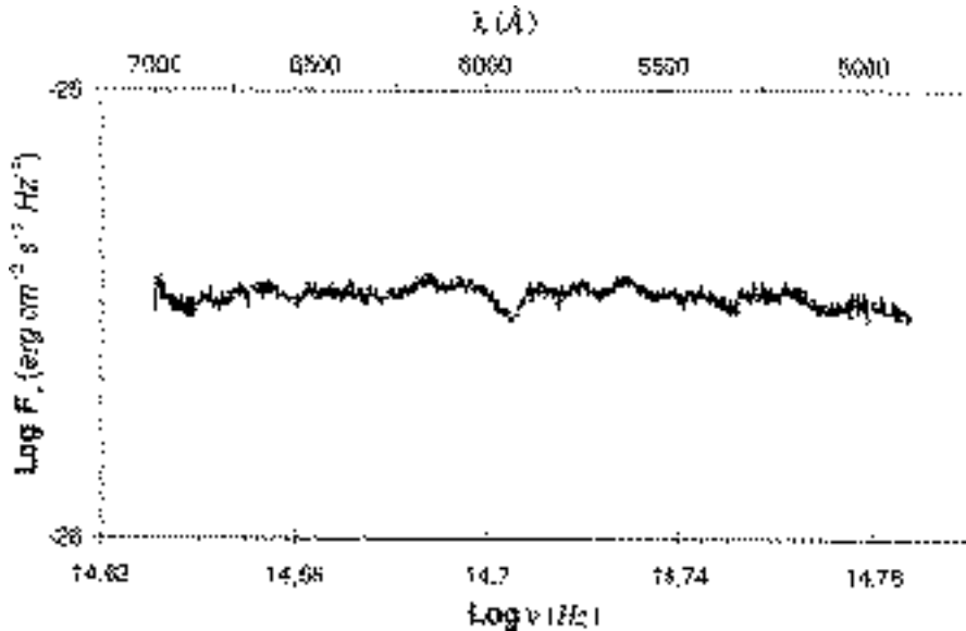
Figure 1: Spectrum of the Crab Pulsar in the wavelength range 4900–7000 Å as measured with EMMI after a 40-min exposure. The spectrum has been sky subtracted and corrected for interstellar absorption. The flux distribution is modelled by a power law with a best fitting spectral index \alpha = -0.10 \pm 0.01 . A broad ( \Delta\lambda \sim 100 Å) absorption feature centred on \lambda = 5900 Å is visible.
