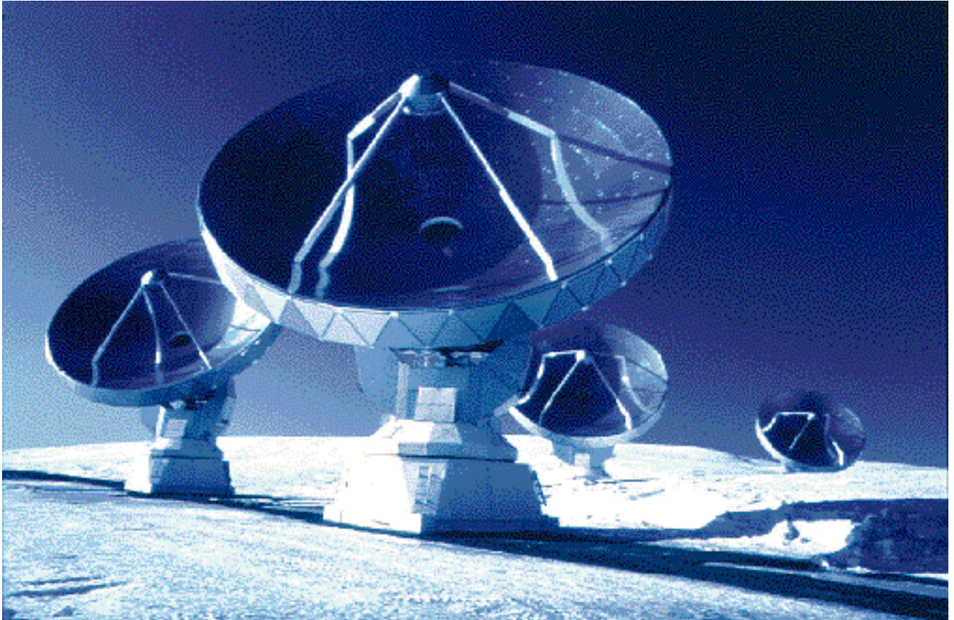
Current state-of-the-art in millimetre arrays: the four 15-m antennas of the IRAM interferometer on Plateau de Bure, France. Photo: A. Rambaud, IRAM.
