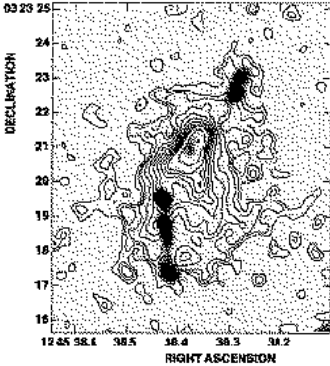
Figure 2: A contour plot of the \text{Ly}\alpha halo of the radio galaxy 1243+036 at z = 3.6 , with a grey-scale plot of the 8.3-GHz VLA map superimposed.
