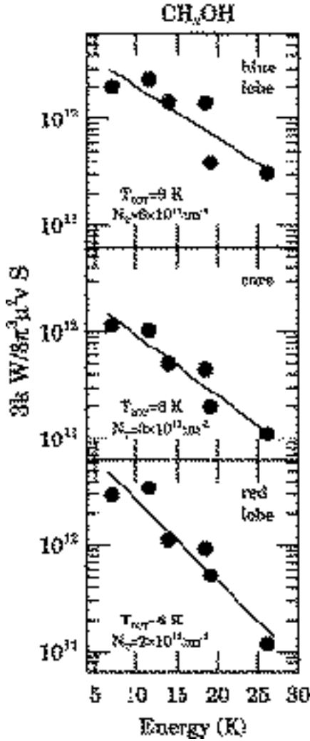
Figure 5. Rotation diagrams for the methanol transitions observed toward the red lobe, central core, and blue lobe of Sandqvist 136. The lines correspond to least squares linear fits to the observed data. The derived values of the rotational temperature and total column density are given in the lower left corner.
