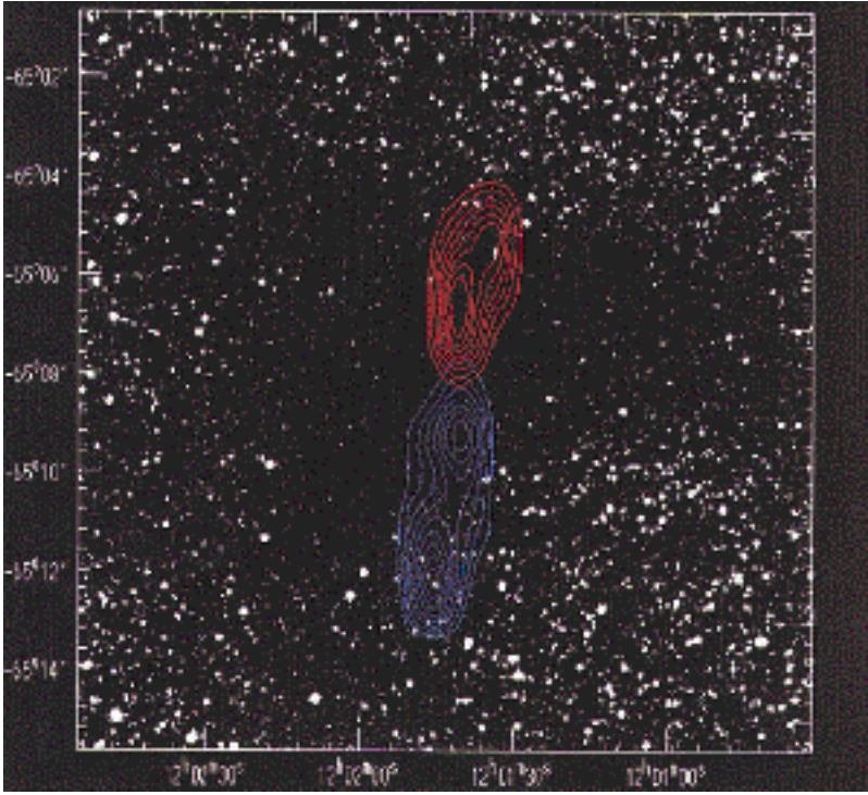
Figure 1: Contour map of velocity integrated CO(1→0) line wing emission from the Sandqvist 136 bipolar outflow, superimposed on a V-band image of the globule taken from the Digitised Sky Survey. Co-ordinate labels are J2000. Blue contours correspond to the emission integrated in the velocity range from -13.5 to -8.5 \text{km s}^{-1} (blueshifted wing) and red contours to the integrated emission in the velocity range from -0.5 to 4.5 \text{km s}^{-1} (redshifted wing). The lowest contour and contour interval are, respectively, 1.8 and 0.8 \text{K km s}^{-1} for the redshifted emission and 1.0 and 0.5 \text{K km s}^{-1} for the blueshifted emission.
