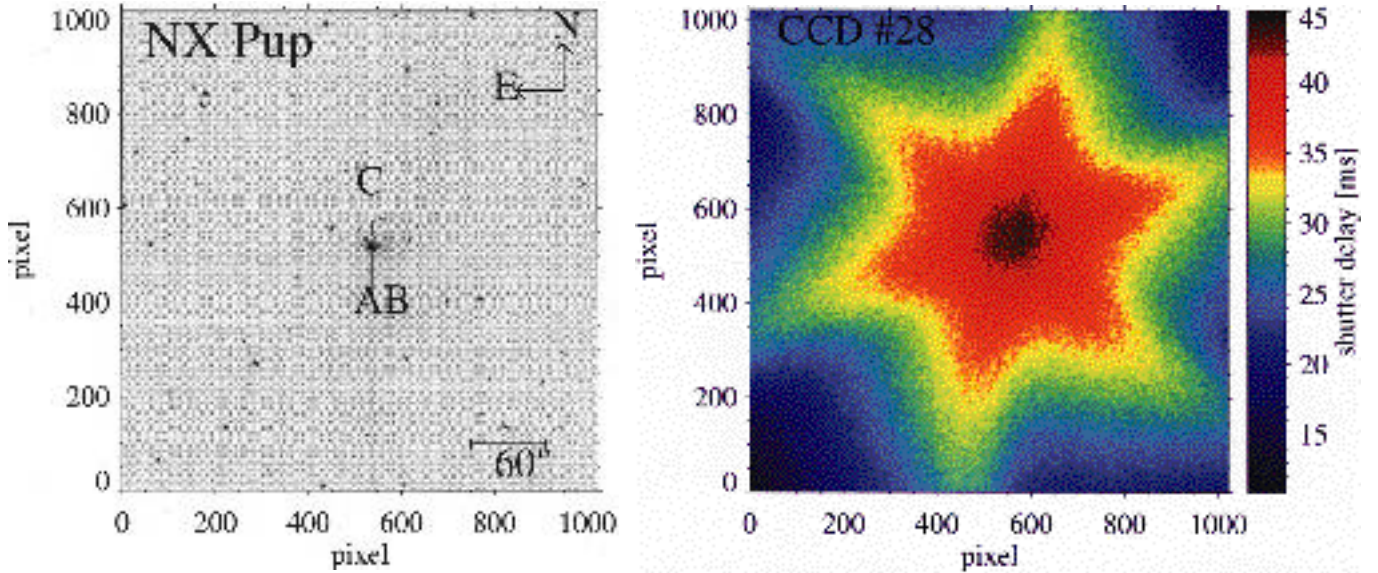
Figure 2: 1.5-s R exposure of the region around NX Pup obtained with the CCD camera at the D1.54-m telescope in 1995 March 11 (left). NX Pup AB (unresolved) and the associated classical T Tauri star NX Pup C are marked. The shutter delay in the central part of the CCD amounts to 45 ms, which in the 1.5-s exposure image induces a photometric error of 3%. The corresponding shutter map is shown on the right.
