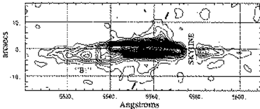
Figure 4: A two-dimensional representation of the 2.8 Å resolution spectrum of Ly \alpha of 1243+036 ( z = 3.6 ) taken through a slit oriented along the main axis of the radio emission.
