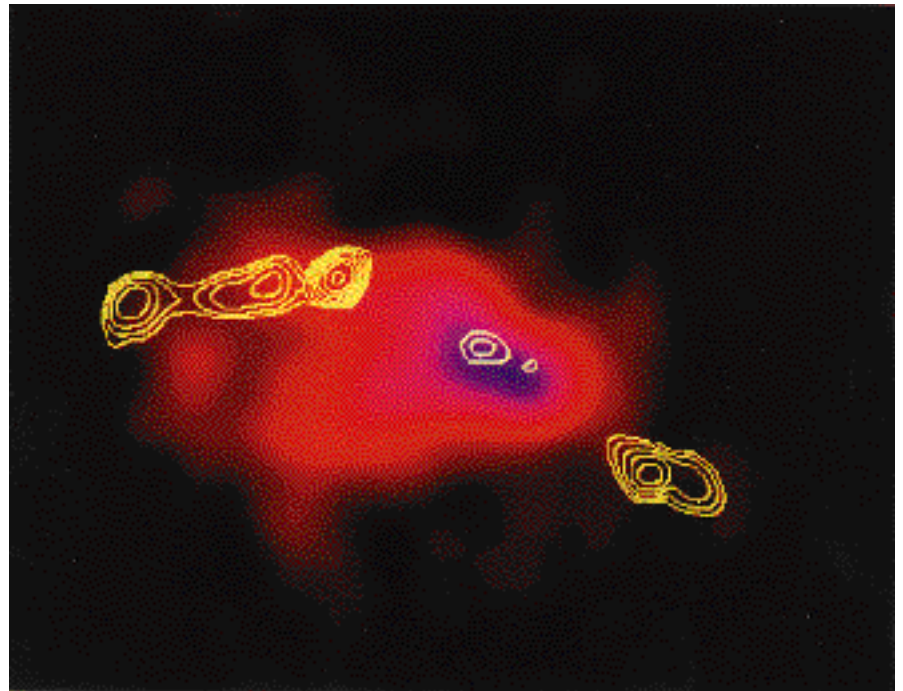
Figure 3: A colour representation of the \text{Ly}\alpha halo of the radio galaxy 1243+036 at z = 3.6 , with a contour plot of the 8.3-GHz VLA map superimposed.
