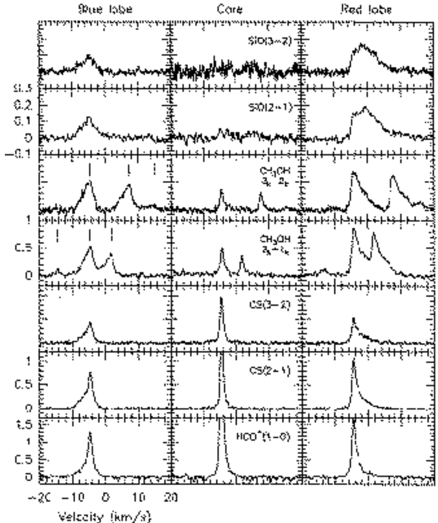
Figure 3. Spectra of the spatially integrated line emission from the blue and red lobes of the Sandqvist 136 outflow and from the central position (Middle column).
