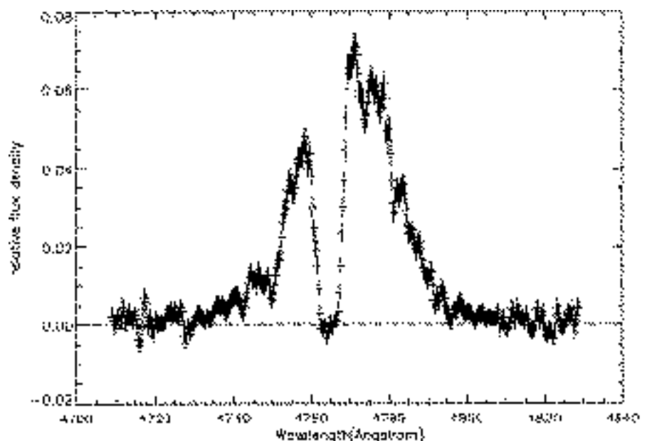
Figure 5: Part of the high-resolution spectrum (1.5 Å) of the Ly \alpha region of the z = 2.9 radio galaxy 0943-242. (see also Röttgering et al., 1995).
