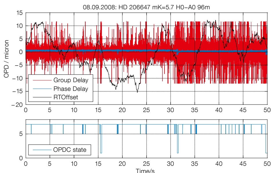
Figure 3. By the end of the PRIMA Big Bang, fringes from stars with K \sim 6 were not only being detected, but actively tracked. The upper panel shows the phase delay (blue), group delay (red) and delay line offset (black) in microns of optical path delay as a function of time for star HD 206647 with ATs at VLT stations A0 and H0 for a separation of 96 m. The lower panel shows the optical path delay controller (OPDC) state during this time, with a high state (7) indicating fringe lock, low (1) a fringe search state, and a middle state (5) reflecting a minor loss being waited out.
