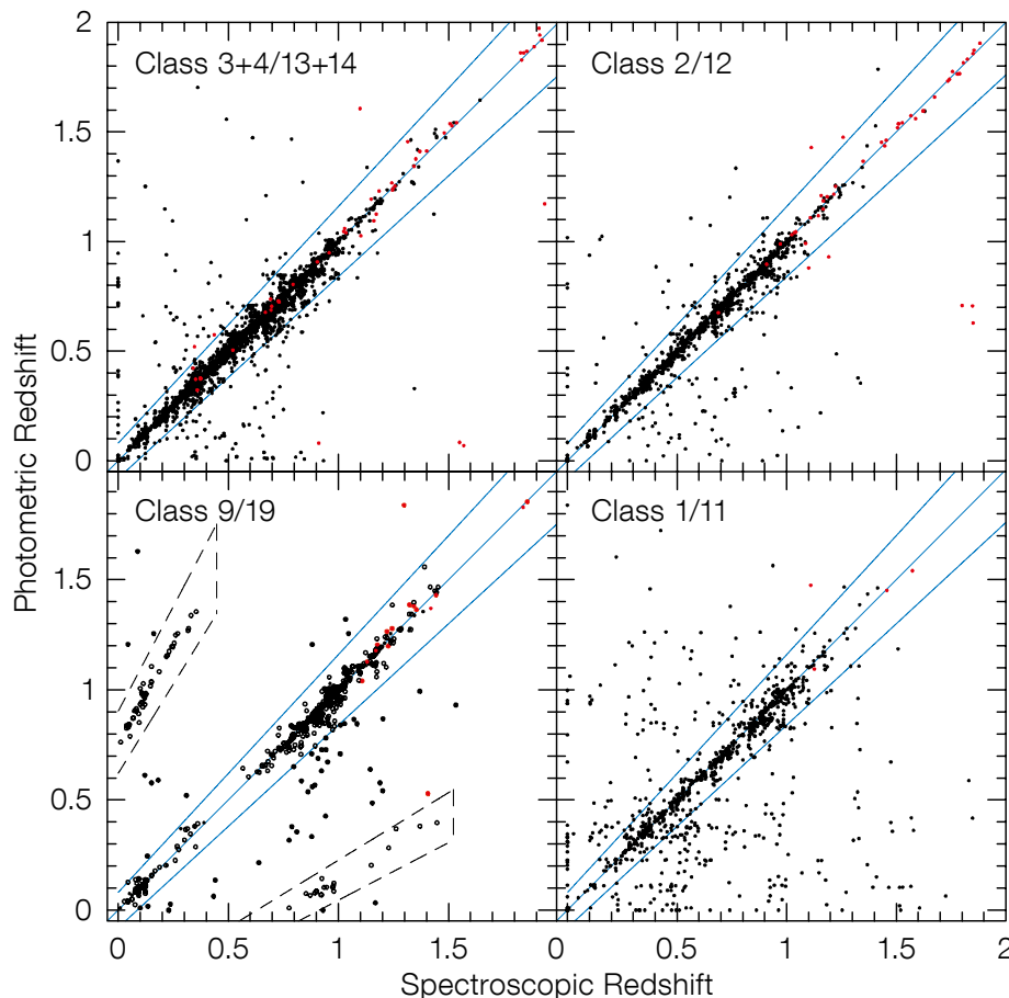
Figure 1. Comparison of photometric and spectroscopic redshifts of zCOSMOS-bright galaxies, as described in the text. Note that Class 9 redshifts are those based on a single emission line, which therefore have two alternative redshifts based on either a [O II] 3727 Å or H \alpha 6563 Å identification. A “1” preceding the Class (e.g. 4 \rightarrow 14) indicates a broad line AGN, indicated by red points on the figure.
