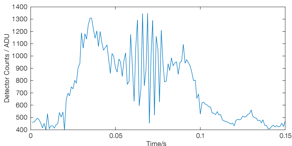
Figure 2. First fringes for PRIMA, obtained on Fringe Sensor Unit A on 3 September 2008, observing the star HD 19349 with two ATs separated by 32 m at VLT stations G0 and G2.
