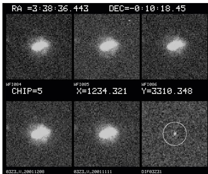
Figure 2. An example of a SNorAGN candidate discovered in the V -band (layout of images as in Figure 1). The variable source occurs near the galaxy nucleus. This candidate is actually an AGN and was also discovered by the Sloan Digital Sky Survey.
