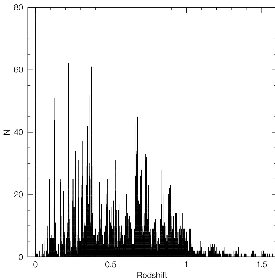
Figure 3. (Below) Redshift distribution of extra-galactic objects in the zCOSMOS-bright 10k sample with secure redshifts, binned in intervals \Delta z = 0.001 , which is larger than the redshift uncertainty by a factor of three at z = 0 and of two at z \sim 1 . Despite the large transverse dimension of the survey, the redshift distribution shows structure on all scales from the velocity resolution up to \Delta z \sim 0.05 .
