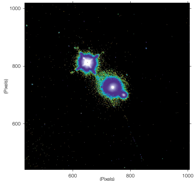
Figure 6. Example faint source for observation with PRIMA. NTT/SOFI image of ESO 548-81. The object is a Seyfert 1 galaxy, too dim for direct fringe tracking at K \geq 10.5 , but nearby there is a bright source (HD 23134, K = 6.02 ) that can be used to phase-up the interferometer.
