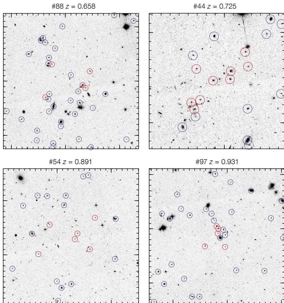
Figure 4. Four representative zCOSMOS groups at 0.6 < z < 1 . In the complete 10k sample there are 151 groups with four or more members and another 649 with two or three members. Group members are circled in red. Other galaxies with spectroscopic redshifts that are not in the group are circled in blue.
