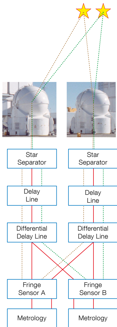
Figure 4. Schematic of the PRIMA system for the VLTI, highlighting the major subsystems along the optical paths of the facility.
