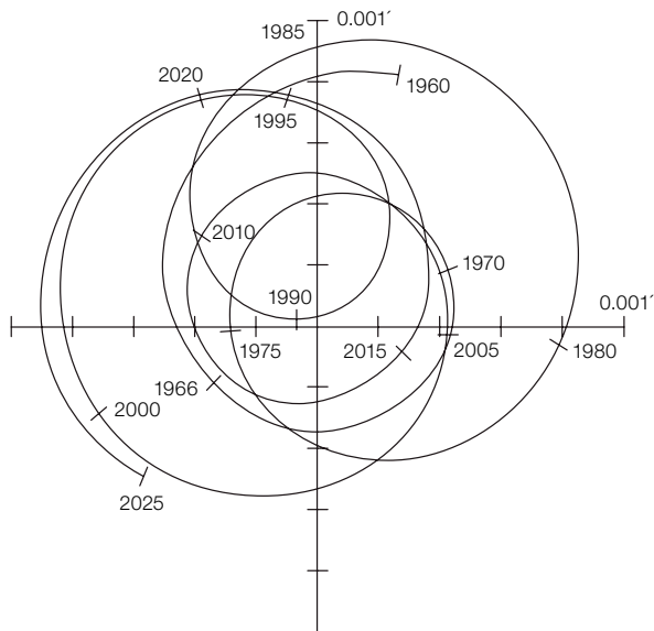
Figure 5. Apparent astrometric signature of our Sun as a function of time at a distance of 10 parsecs, exhibiting the astrometric reflex motion associated with all of the Solar System planets. Jupiter dominates, followed by Saturn and the other two gas giants. Earth's signature is masked by the plot line width at the \leq 1 \mu\text{as} level.
