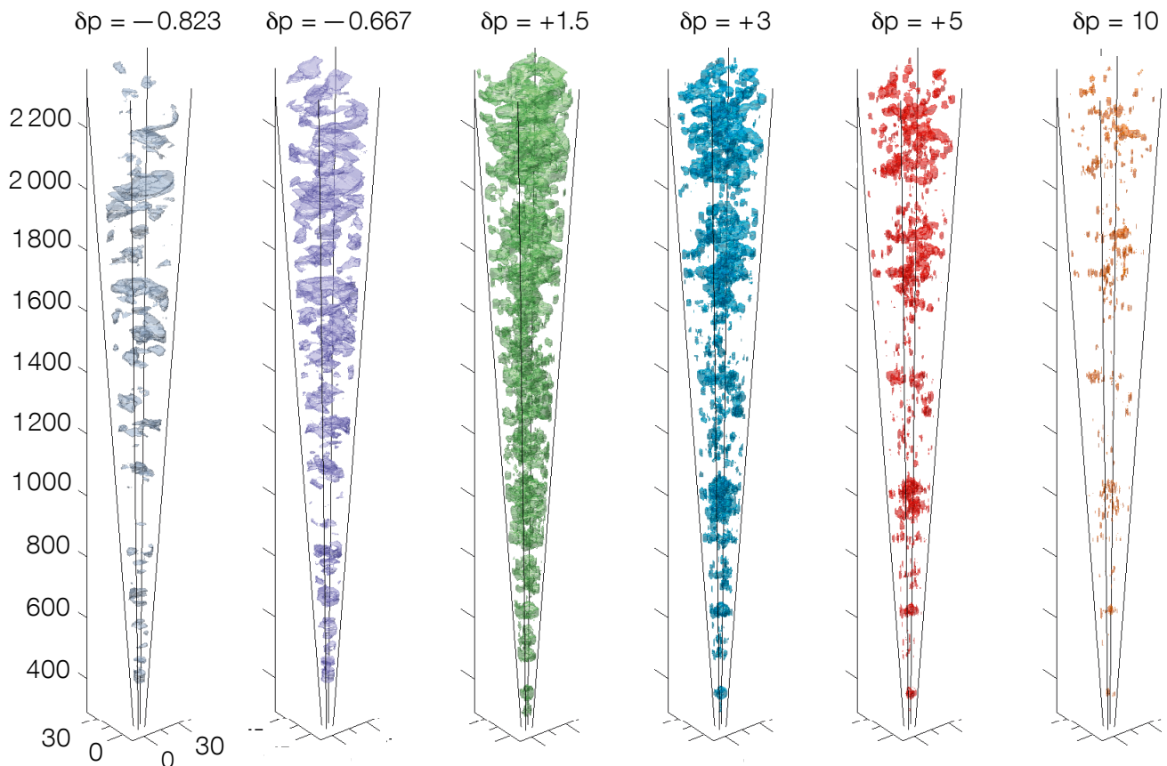
Figure 4. The galaxy density field reconstructed from the zCOSMOS 10k sample using the ZADE algorithm to include about 30 000 galaxies with photometrically estimated redshifts. The maximum comoving distance of 2400 Mpc corresponds to a redshift z = 1 . The cones show, from left to right, iso-density surfaces corresponding to underdensities of \delta\rho = -0.823 , \delta\rho = -0.667 and overdensities of \delta\rho = +1.5 , 3, 5 and 10 respectively. Because the density field is locally projected to avoid the effects of peculiar motions, the equivalent physical overdensities are significantly higher, approximately \delta \sim 3, 7, 13 and 35 for the four rightmost cones.
