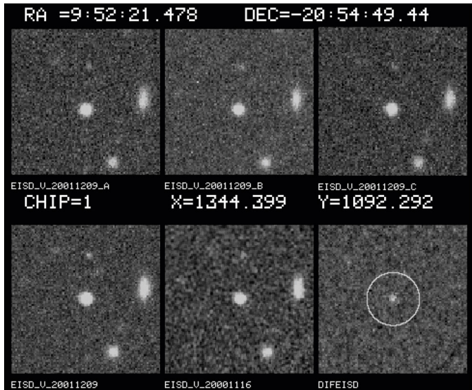
Figure 3. An example of a variable star discovered in the V-band (layout of images as in Figure 1). The source shows a stellar profile on all images.
