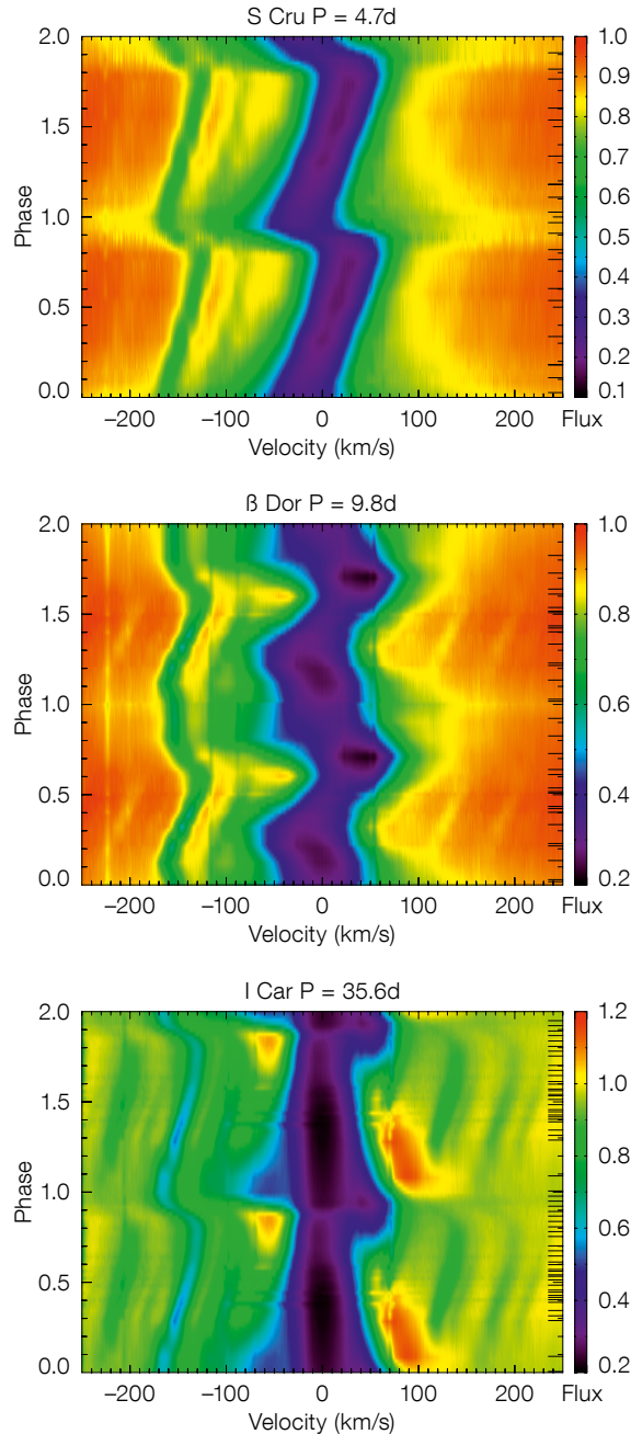
Figure 5. H\alpha line profiles of short, medium and long period Cepheids. Time series of HARPS spectra are interpolated to provide a two-dimensional map of the H\alpha profile in the [-250, 250] km/s velocity range. Diagrams are given in the stellar rest frame with positive velocities corresponding to receding motion (red-shifted). The pulsation phase is indicated on the left edge of each panel and on the right we quote the pulsation phases corresponding to our observations (data are duplicated over two pulsation cycles for clarity). For each star the colour bar indicates the continuum-normalised flux.
