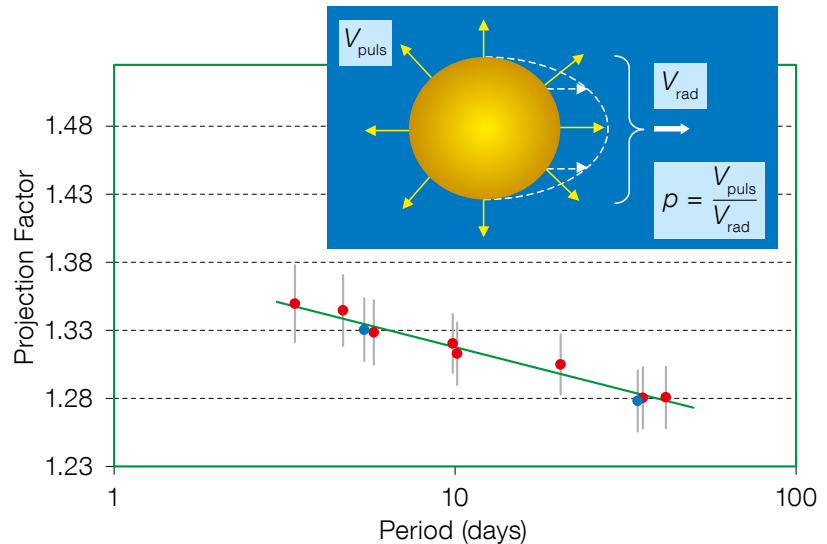
Figure 4. The projection factor ( p ) used in the interferometric Baade-Wesselink (IBW) and infrared surface brightness (IRSB) methods for determining the distance of Cepheids includes a geometrical effect (see inset box), a velocity gradient within the atmosphere and the relative motion of the line-forming region with respect to the corresponding mass elements. A relation was found between the projection factor and the logarithm of the period. Red points are semi-theoretical (including the HARPS determination of velocity gradients), while blue points are from hydrodynamical models.
