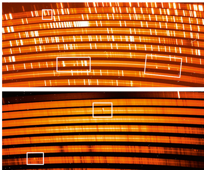
Figure 3. This 20-minute exposure of SN2008hg ( m_V \approx 17.5 ) taken at full Moon gives a hint of the capability of X-shooter. V-R and UV-B spectra of the SN with emission lines of the nearby H \Pi region (with the brightest highlighted in boxes) cover the range from 310 to 1000 nm. The spectra were taken with slit widths of 1.2 and 1.3 arcseconds in the V-R and UV-B ranges respectively in 1.4 arcsecond seeing. The resolving powers are 6000 and 4000 approximately. Using narrow slits, the instrument can reach resolutions of 14000 and 9000 in the V-R and UV-B bands respectively.
