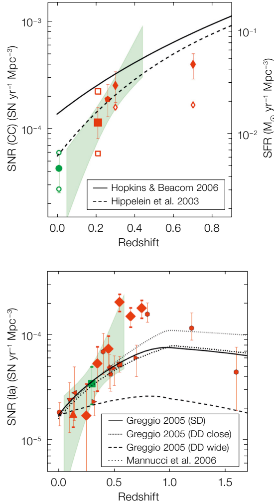
Figure 6. SN Ia rate measurements in the literature and predictions obtained by convolving the SFH of Hopkins & Beacom with various delay time distribution functions. The predicted paths are plotted as lines with different types (see inset box for key). The shaded area represents the 1\sigma confidence level of our estimate of SN Ia rate evolution as deduced from the likelihood fit. The circle is the measurement of Cappellaro et al. (1999); the inverted triangle from Madgwick et al. (2003); the leftward triangle for Hardin et al. (2000); the triangle for Blanc et al. (2004); the rightward triangles for Neill et al. (2007); the green square for Botticella et al. (2008); the rhombi for Barris & Tonry (2006); the small rhombus for Tonry et al. (2003); the pentagon for Neill et al. (2006); and the red square from Pain et al. (2002) and the hexagons for Dahlen et al. (2004).
