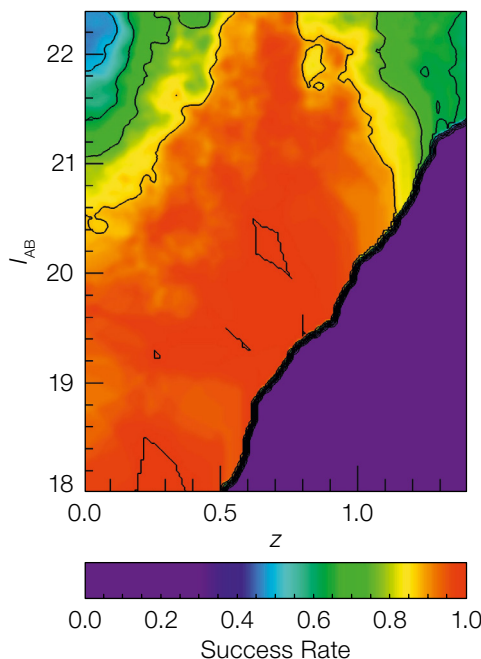
Figure 2. (Left) Fraction of spectra yielding a successful spectroscopic redshift measurement as a function of redshift (derived from the photo-z for the remainder) and I_{AB} magnitude. Notice how the success rate stays high in the key redshift range 0.5 < z < 0.8 all the way to the limiting depth of the survey.
