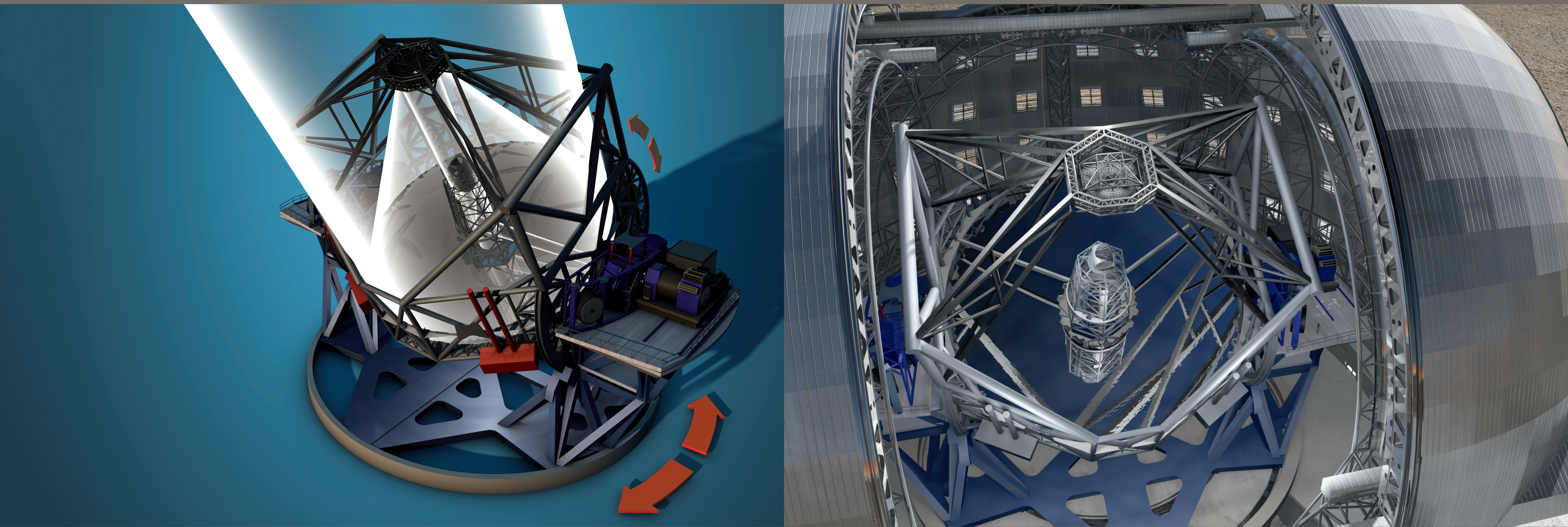
Schematic view of the E-ELT, showing the path light takes through its five-mirror design.
