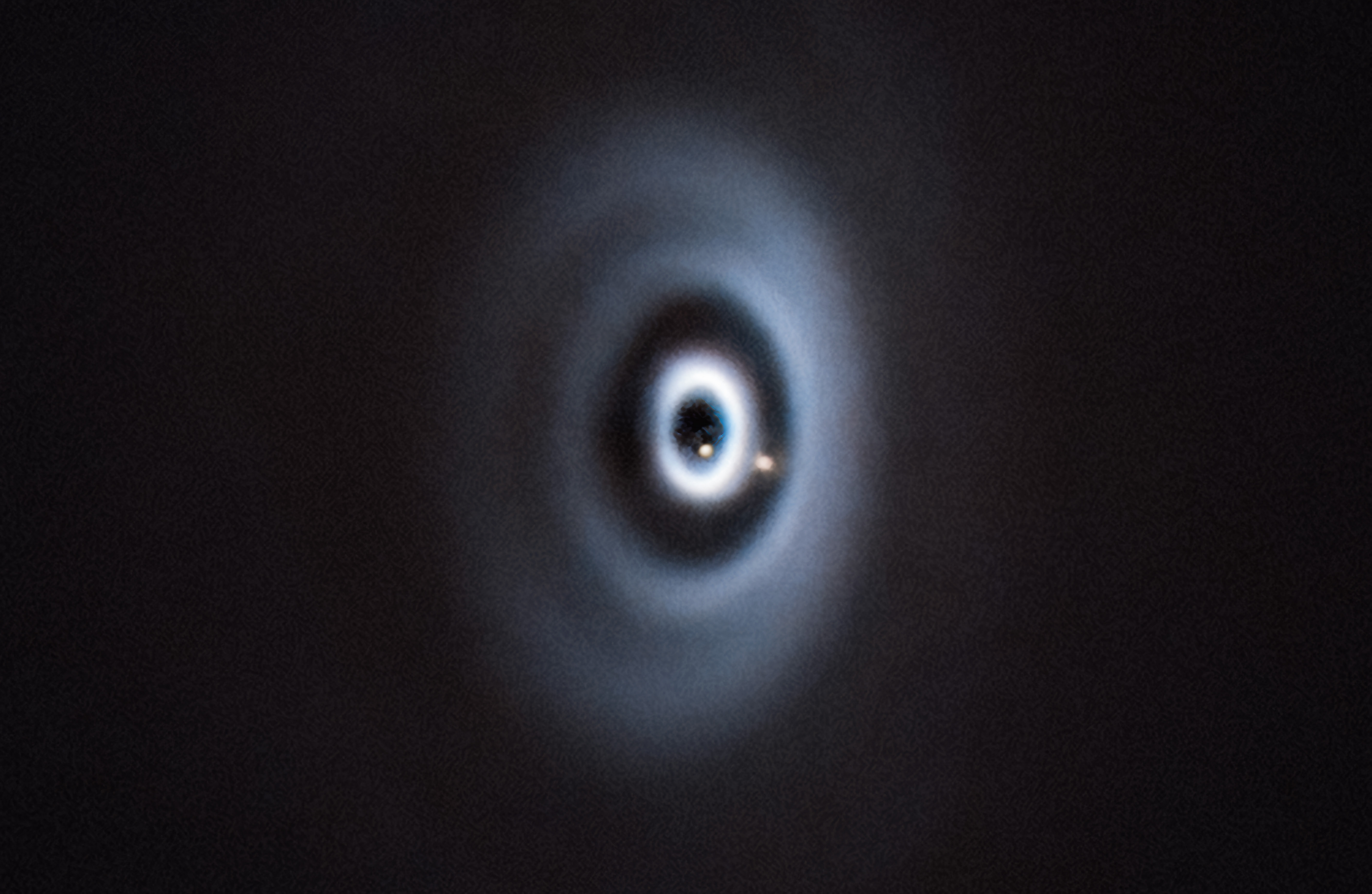
Composite VLT image of two planets around the star WISPIT 2
