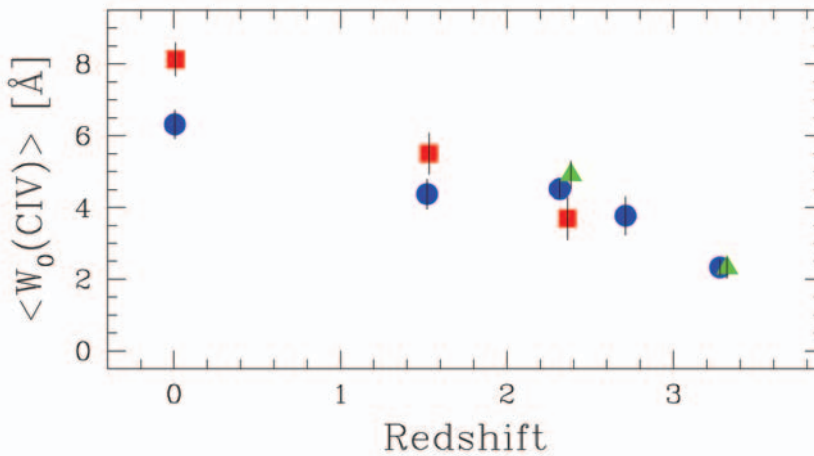
Figure 7: Mean strength of the resonance doublet of the carbon ion C^{++} in the spectra of FDF starburst galaxies as a function of redshift. Since in starburst galaxies the strength of this blend is approximately proportional to the abundance of heavy elements, the diagram illustrates directly the chemical enrichment of the universe with decreasing redshift (or increasing cosmic age).
