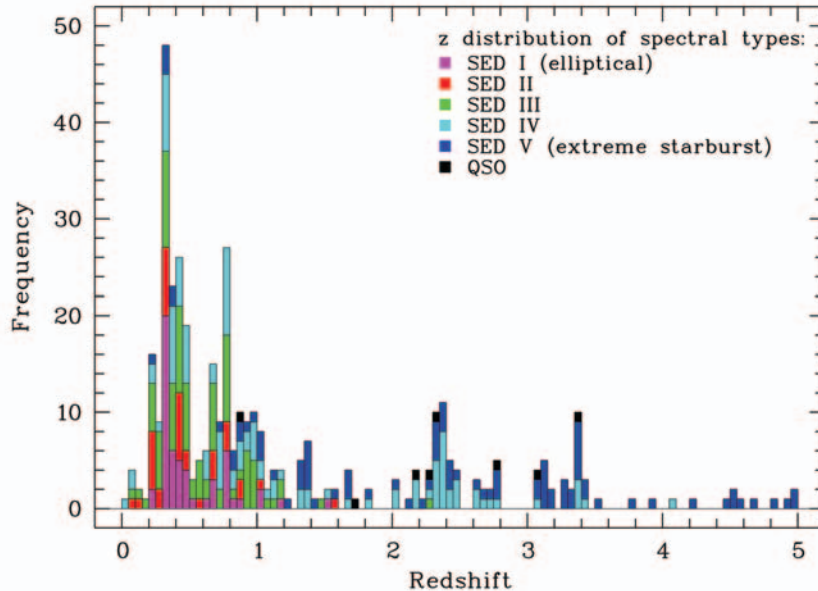
Figure 3: The distribution of the well measured spectroscopic redshifts in the FDF. The ordinate gives the number of galaxies per redshift interval of 0.05. The colours differentiate galaxies with different levels of star formation activity, ranging from insignificant star formation (magenta) to extreme starbursts (dark blue).
