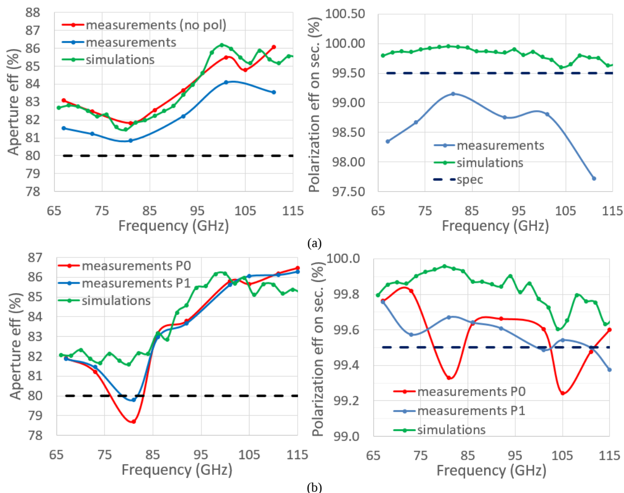
Figure 5. Measured and simulated aperture and polarization efficiencies. Thick dashed line in every graph indicates ALMA requirements. (a) System developed at Universidad de Chile. (b) System developed at INAF.
