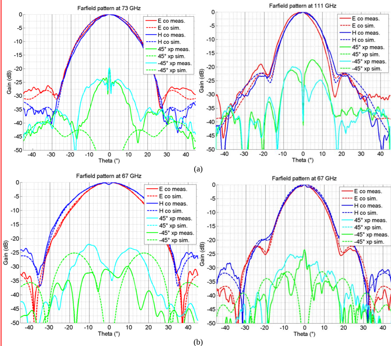
Figure 4. Far-field beam patterns of the two different systems at two different frequencies. (a) System developed at Universidad de Chile. (b) System developed at INAF.
