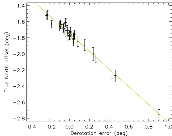
Figure 4. True North offset estimate as a function of the derotation error caused by missynchronization issues between the SPHERE and VLT internal clocks. A clear correlation (average fitting residuals 0.03^\circ ) is seen between large true North deviations and large derotation errors.
