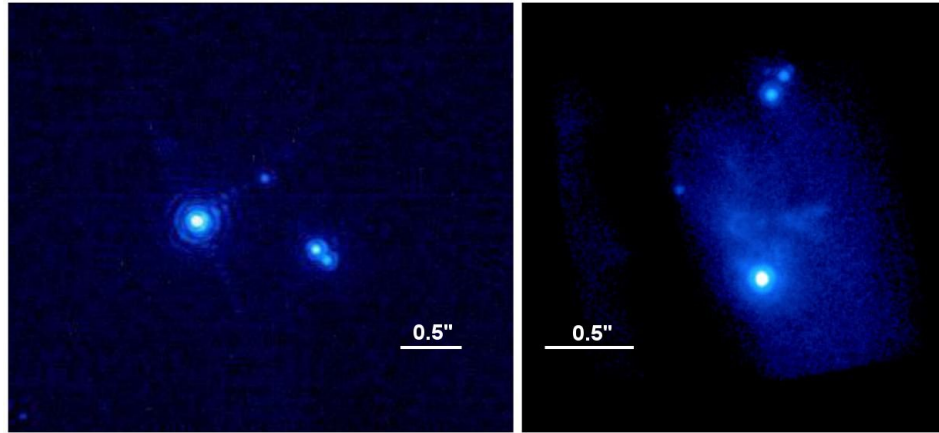
Figure 6. IRDIS (left) and IFS (right) images of the Orion Trapezium B1–B4 quadruple.
