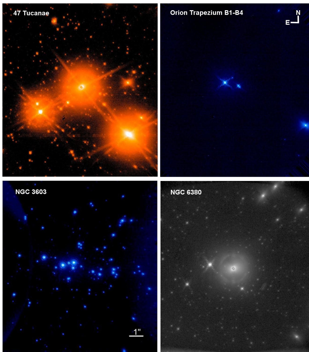
Figure 1. IRDIS images of the main reference SPHERE astrometric fields.
