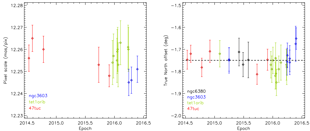
Figure 5. Individual measurements for the pixel scale (left) and true North (right) of IRDIS. For the pixel scale measurements, only the configuration H2 filter + N_ALC_YJH_S coronagraph is considered.
