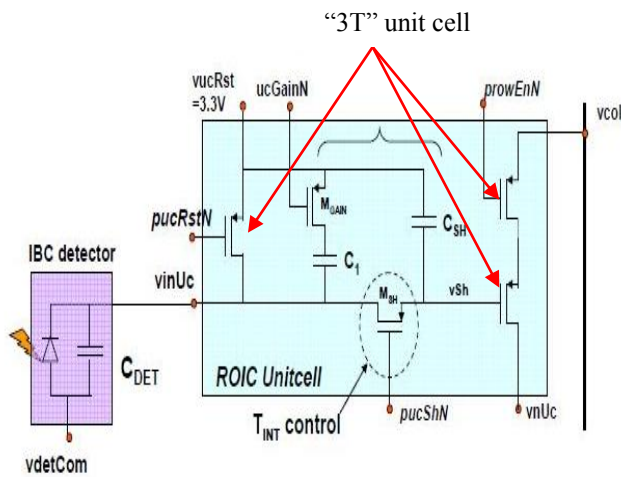
Figure 2a: AQUARIUS detector unit cell design
