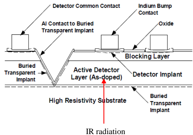
Figure 1b: Basic architecture of a back illuminated IBC detector, from AQUARIUS user manual.
