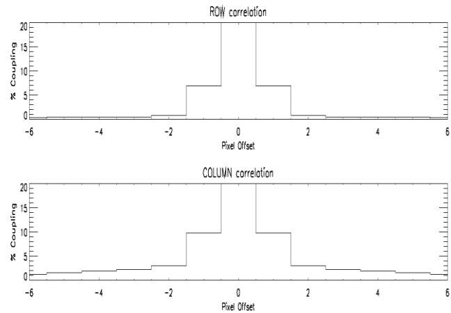
Figure 9b: 2D autocorrelation result for rows (top) and columns (bottom).
