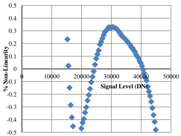
Figure 7b: Detector non-linearity as a function of signal level for high gain. Computed by fixing a slope to the data and measuring the difference to the slope.
