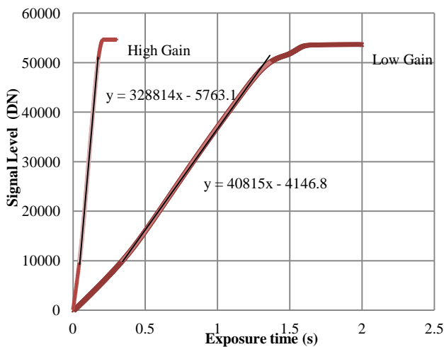
Figure 7a: Typical linear plot for both high and low gain read modes. The slope gives the gain change to be approximately \times 8 .
