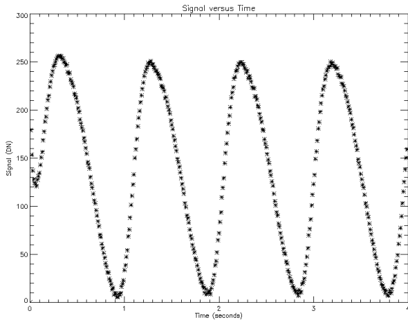
Figure 4a: Thermal oscillation seen on detector output as a plot of signal for constant flux against time
