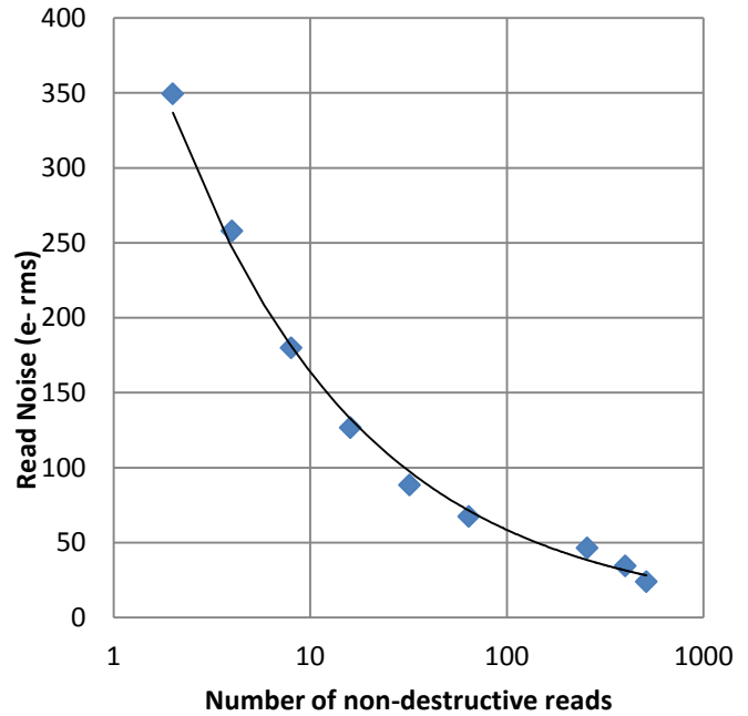
Figure 8b: Read noise versus number of non-destructive reads
