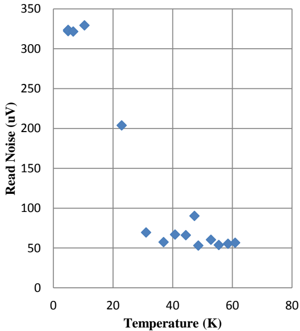
Figure 8a: Read noise versus detector operating temperature.
