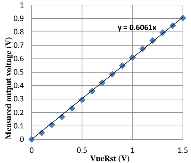
Figure 2b: AQUARIUS Internal Transfer Function
