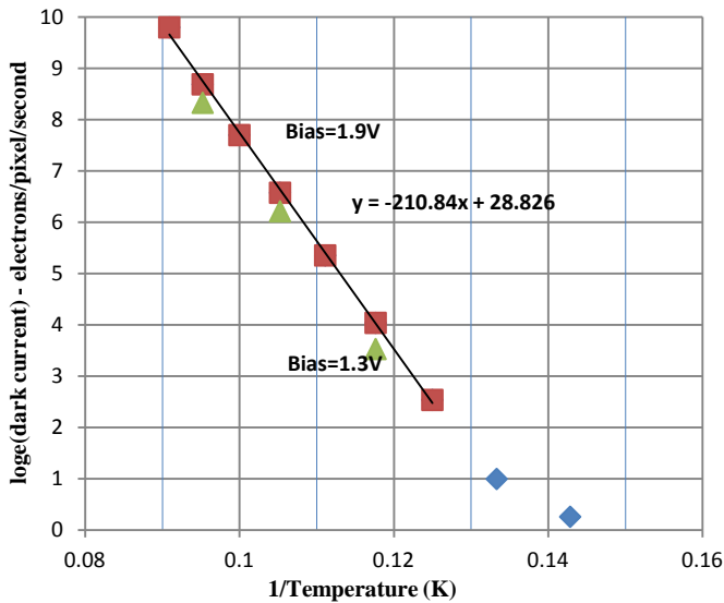
Figure 6a: Typical Arrhenius plot of dark current for two different reverse bias voltages, showing exponential dependence of thermal activation.
