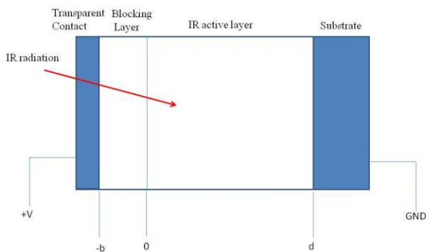
Figure 1a: Typical structure for an n-type IBC detector
