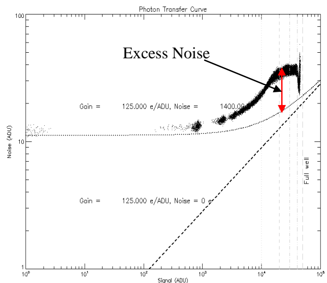
Figure 11b: Photon Transfer Curve for AQUARIUS detector in LOW gain configuration.
