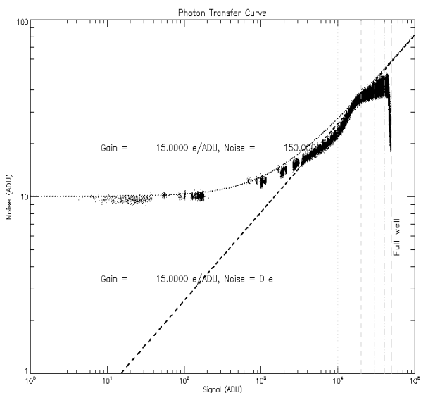
Figure 11a: Photon Transfer Curve for AQUARIUS detector in HIGH gain configuration. The dashed lines are for simulated data with and without read noise.
