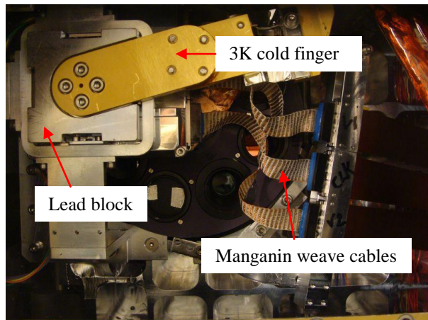
Figure 4b: Detector mount showing addition of lead to minimise thermal oscillation
