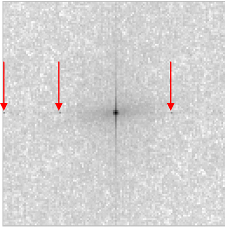
Figure 9a: 2D autocorrelation result for flat field. Image shows the correlation of any pixel to its nearest neighbouring pixels. Highlighted are pixels 32 columns away on same row.
