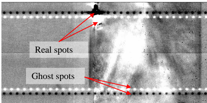
Figure 10a: Difference image for spot projected onto detector and then moved slightly for second image. Image highlights the “Ghosting” to all other outputs.
