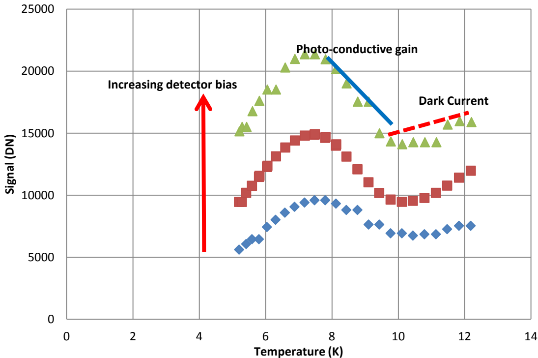
Figure 12a: Signal versus operating temperature for a constant flux and different detector biases. The plot shows the regions of photo-conductive gain and dark current.
