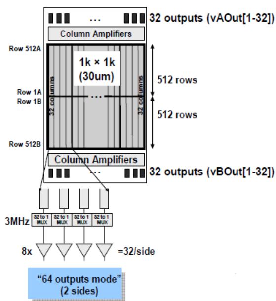
Figure 3a: AQUARIUS multiplexing readout scheme
