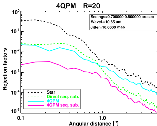
Figure 6: Rejection performances of VISIR in standard imaging mode and coronagraphic mode (assuming a seeing of 0.7"). The rejection factor is defined as the ability to detect a point source close to a bright source of flux unity. When observing in direct imaging (black dashed curve), a source 20 times fainter than the primary can be detected at a distance of 0.5". After PSF subtraction using a reference star (observed under slightly different conditions of seeing (0.8")), this factor grows to ~100 (green dashed line). When observing in coronagraphic mode, the rejection factors at the same distance are about 125 (light blue line) and 660 after PSF subtraction (magenta solid line).
