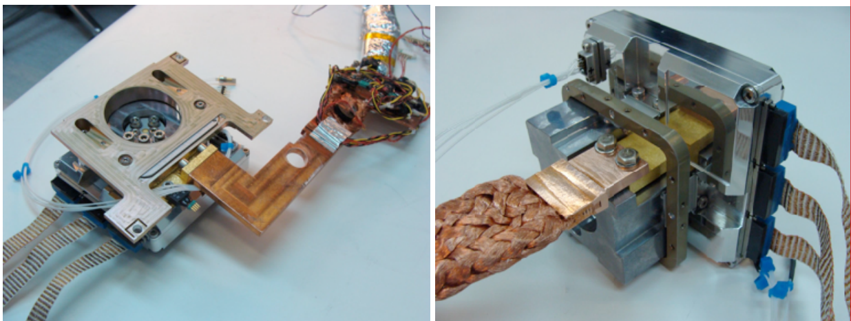
Figure 2. Left: The VISIR imager detector mount. Right: VISIR spectrometer detector mount.
