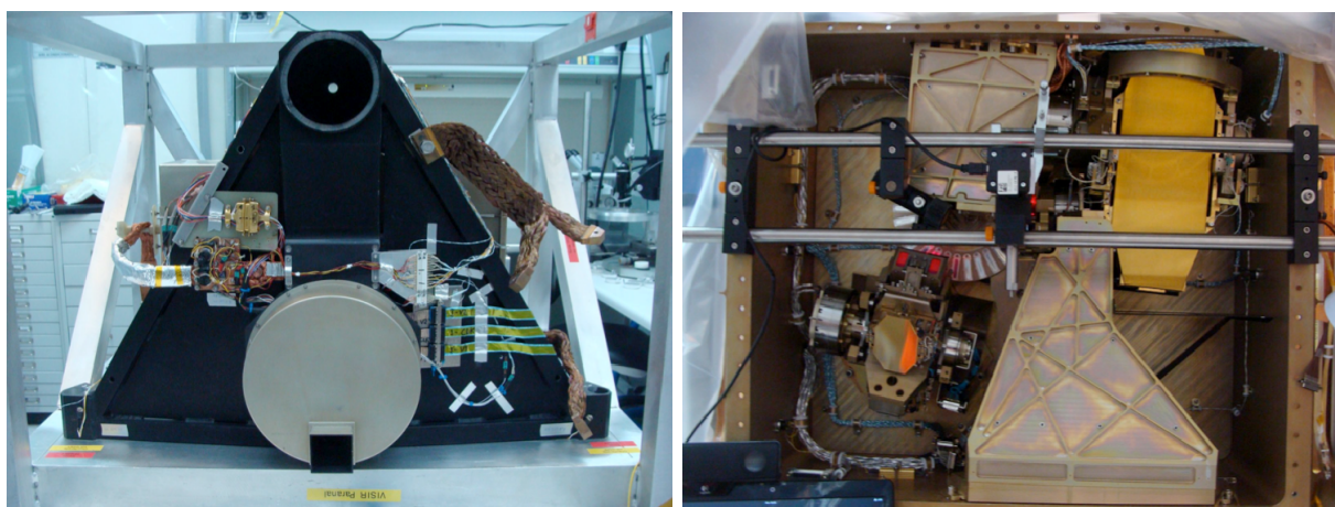
Figure 3. Left: The VISIR imager fully integrated after the intervention. Right: Optical alignment of VISIR spectrometer with CMOS camera and laser.
