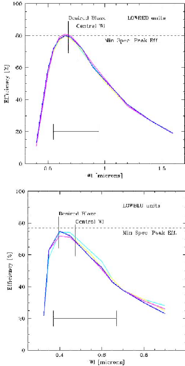
Figure A1: Efficiency curve of the low resolution grisms LR-red, LR-blue. The vertical lines mark the desired blaze and the central wavelengths. The spectral range refers to the slit in the center of the field. The cutoff wavelength is in most cases given by the order separation filters, the red CCD limit or the limit of the VIMOS optics in the blue.
