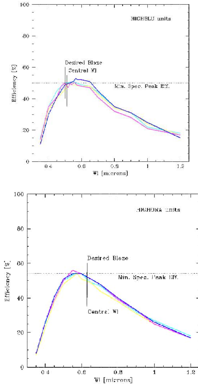
Figure A3: Efficiency curve of the high resolution gratings HR-blue, HR-orange. The vertical lines mark the desired blaze and the central wavelengths. The spectral range refers to the slit in the center of the field. The cutoff wavelength is in most cases given by the order separation filters, the red CCD limit or the limit of the VIMOS optics in the blue.
