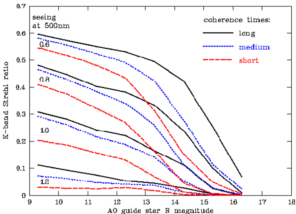
Figure 17: NGS performance for a wide range of optical seeing values (0.6 to 1.2'' ) and long, medium and short coherence times.
