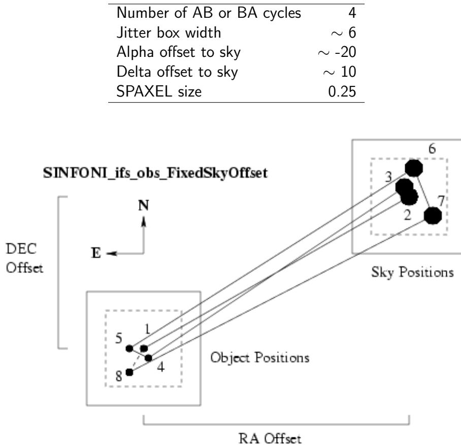
Figure 20: An illustration of the offset sequence taken with the FixedSkyOffset template. (“Number of exposure per Offset” = 1). The large circles for the sky position indicate that these observations are performed in open loop.
