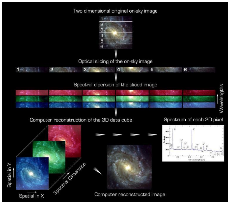
Figure 10: The function of the image slicer. The field of view (top) is slit into small slices which are recombined into a pseudo longslit before being dispersed. The dispersed planes can be recombined to an image, or used to extract spectra at a given point in the field of view.
