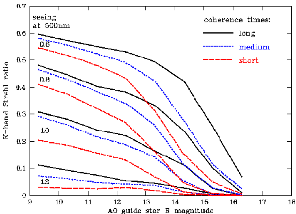
Figure 13: NGS performance for a wide range of optical seeing values (0.6 to 1.2'' ) and long, medium and short coherence times.
