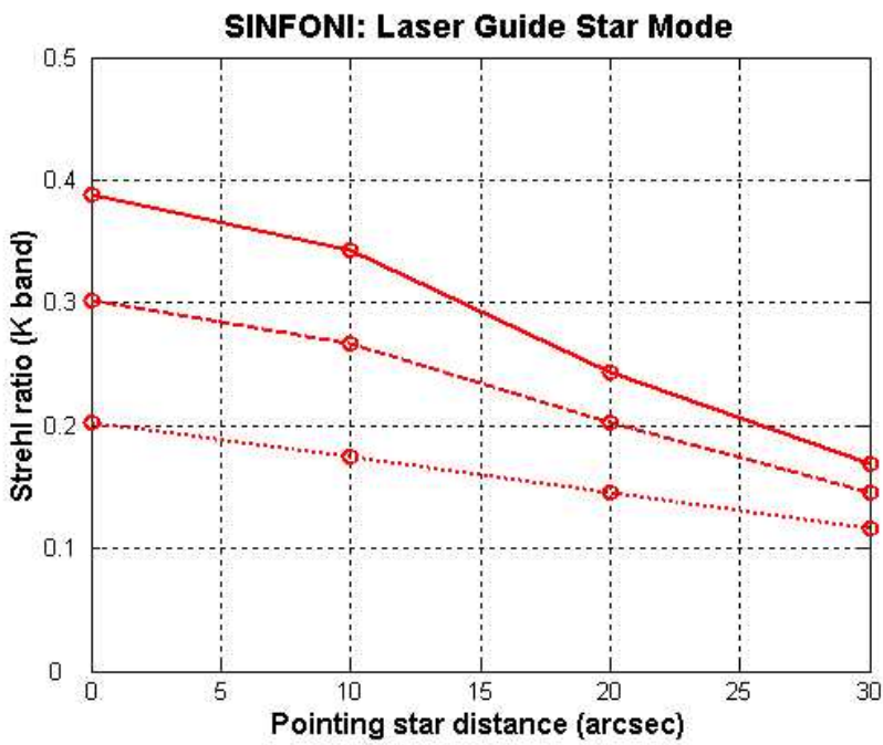
Figure 14: LGS Strehl performance
