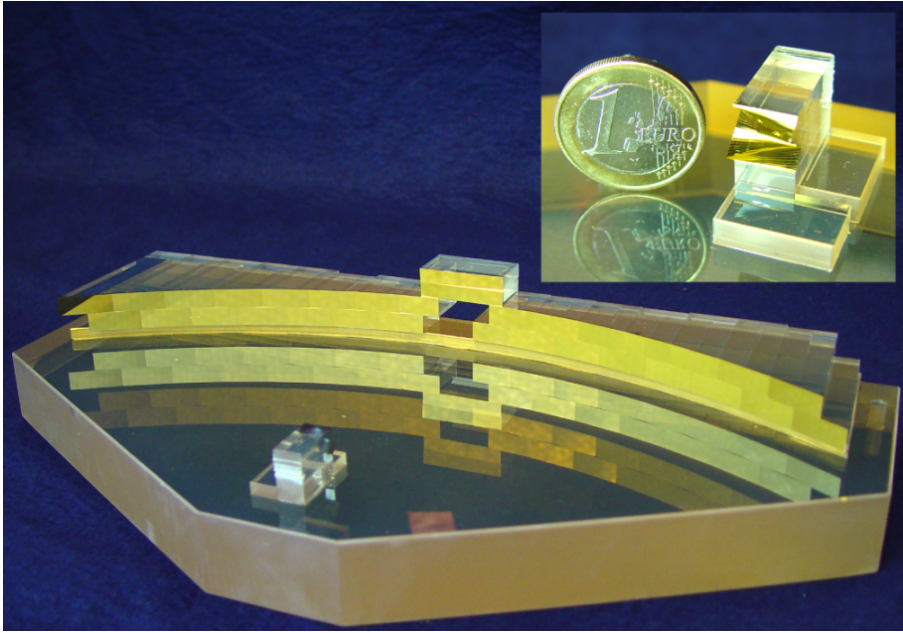
Figure 16: SPIFFI image slicer (a): The light enters through the hole in the big slicer. A stack of 32 small mirrors, the small slicer (also shown in the sub-panel), slices the image and redirects the light towards the 32 mirrors of the big slicer, which re-arranges the slitlets into a 31 cm long pseudo-slit.
