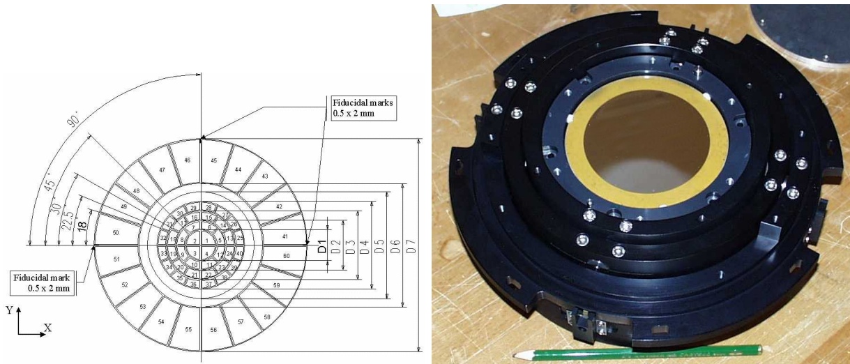
Figure 9: DM electrode geometry – DM/TTM assembly
