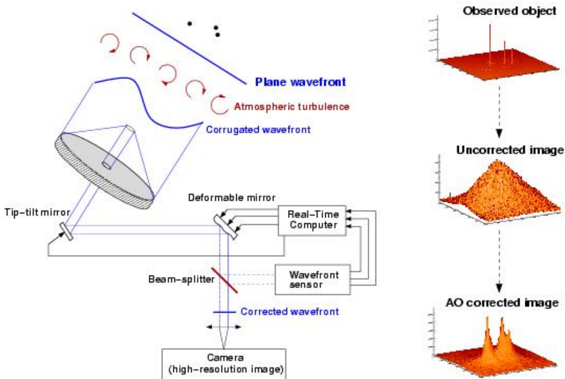
Figure 4: Principle of Adaptive Optics. Note that in practice, and contrary to this schematic design, SINFONI has no dedicated Tip-Tilt mirror, but performs low- and high-order corrections with a single deformable mirror (mounted on a tip-tilt stage).
