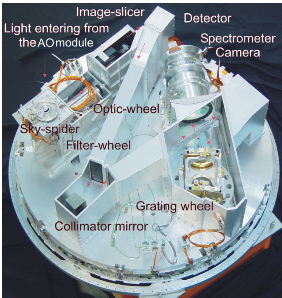
Figure 15: An inside view of SPIFFI: The cryostat cover and the reinforcing structure have been removed to provide a free view on the opto-mechanical components of SPIFFI. The light enters from the top, and passes the sky-spider. The pre-optics with a filter-wheel and interchangeable lenses provides three different image scales. The image slicer re-arranges the two-dimensional field into a pseudo-long slit, which is perpendicular to the base plate. Three diamond turned mirrors collimate the light onto the gratings. In total, four gratings are implemented on the grating drive. A multiple-lens system then focuses the spectra on a Rockwell HAWAII array. The diameter of the instrument is 1.3m.
