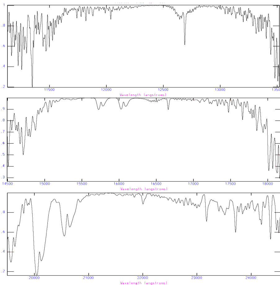
Figure 5: Atmospheric transmission in the J, H and K bands. These graphs are based on FTS data from Kitt Peak, produced by NSF/NOAO.
