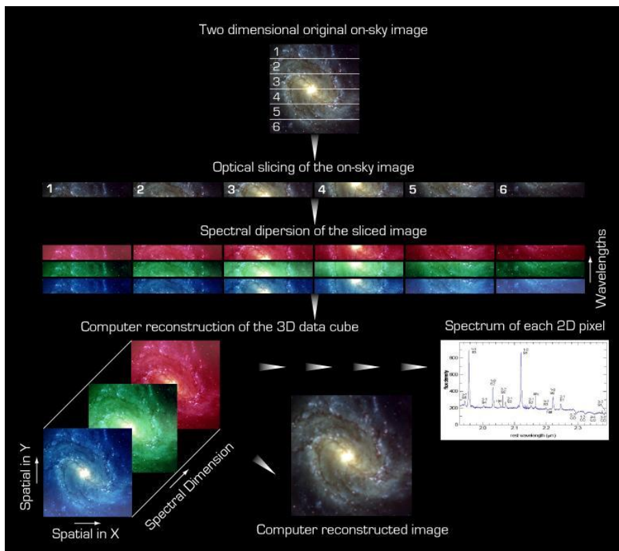
Figure 6: The function of the image slicer. The field of view (top) is slit into small slices which are recombined into a pseudo longslit before being dispersed. The dispersed planes can be recombined to an image, or used to extract spectra at a given point in the field of view.
