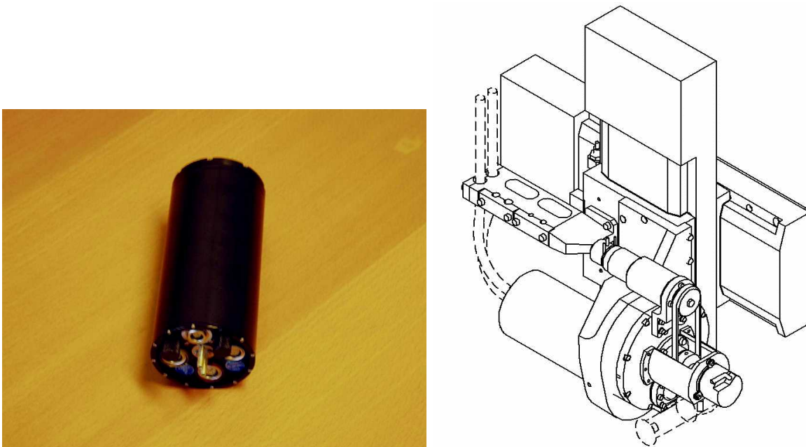
Figure 11: STRAP unit – STRAP assembly
