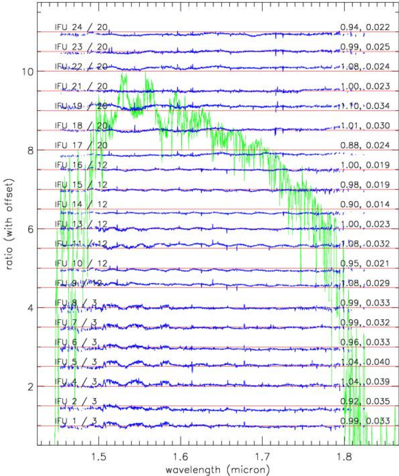
Figure 16: Comparison between the measurements of the 3-arm standard star template and all 24-arms sciencepattern standard star template (Davies et al. 2013, A&A, 558, A56). In the 3-arm standard star the IFUs used are number 3,12 and 20 (one per each spectrograph). The green curve in the background shows the extracted spectrum for a standard star in the H-band. The overplotted blue curves are the ratio (in arbitrary scales and offsetted) between the spectra in each IFU respect to those taken in just 3 reference arms (3,12,20) taken via the 3- arm standard star template, as labelled on the left hand side. For each IFU on the right the mean ratio and the standard deviation are indicated (for regions where the signal-to-noise is above a minimum threshold). This suggests that using just 3 arms to calibrate all IFUs is sufficient at the level of precision of a few percent.
