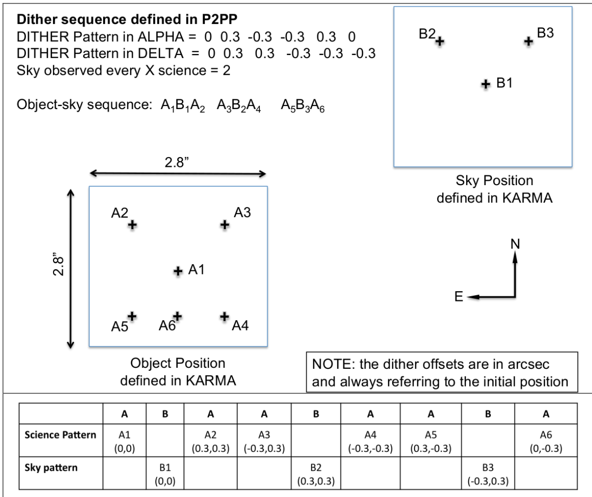
Figure 15: An illustration of the dither pattern that can be constructed with the free-dither template in P2PP. The sequence for just 1 IFU is shown, since it will be identical for all of them. This example is for 6 object frames and sky frequency = 2, which gives in total 3 sky frames in the sequence ABA ABA ABA.
