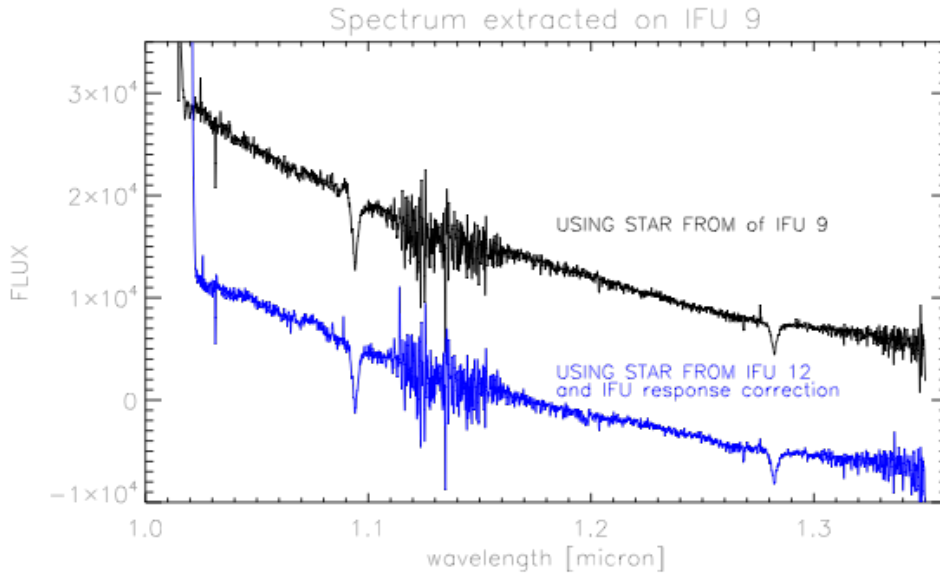
Figure 16: Black spectrum. Example of spectrum observed in IFU 9, calibrated using a telluric template from the same IFU, as foreseen by the template KMOS_spec_cal_stdstarscipatt (one telluric per IFU). Very similar results can be obtained by using the template KMOS_spec_cal_stdstar (that foresees the observation of just one template per detector) and taking into account the differential response correction provided with the pipeline. In this example (blue spectrum), the telluric standard observed in IFU 12 is used to calibrate the spectra of IFU 9.
