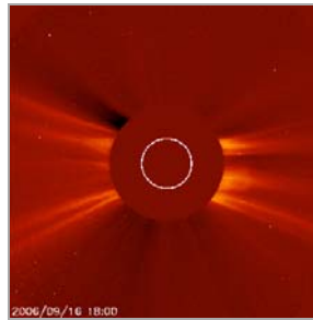
Figure 20: The solar corona (credit: SOHO – LASCO, ESA, NASA). The small ring presents the size of the Sun.
