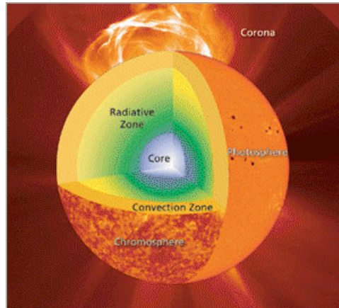
Figure 13: Solar structure (credit: SOHO, ESA, NASA).
