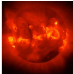
Figure 21: Sun in soft X-ray (credit: Yohkoh Soft X-ray Telescope). The solar surface is invisible, because it shines at wavelengths between 380 - 760 nm.
