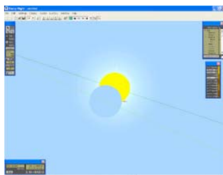
Figure 33: Work with Starry Night Bundle Edition.
