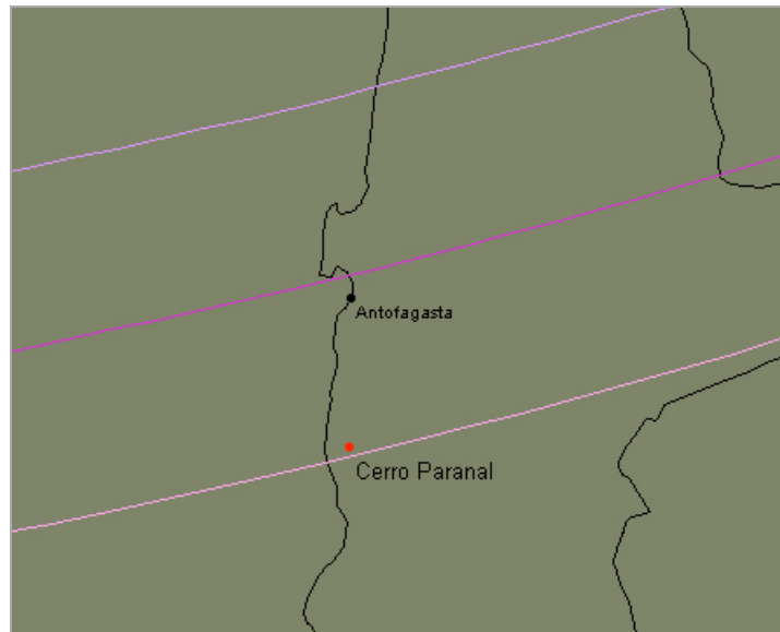
Figure 29: A part of the path of the annular solar eclipse on 11 th of February 2241 (from Redshift 5.1).
