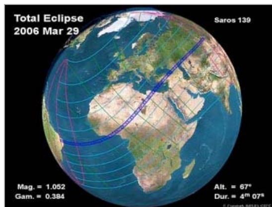
Figure 30: Path of totality of the total solar eclipse on 29 th of March 2006 (Fred Espenak, NASA's GSFC).
