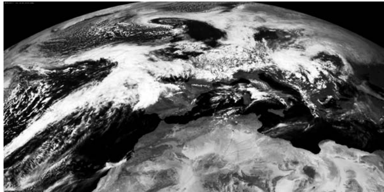
Figure 47: Satellite picture of the Europe on 29th of March 2006 at 12:00 UT (copyright © 2006 EUMETSAT).
