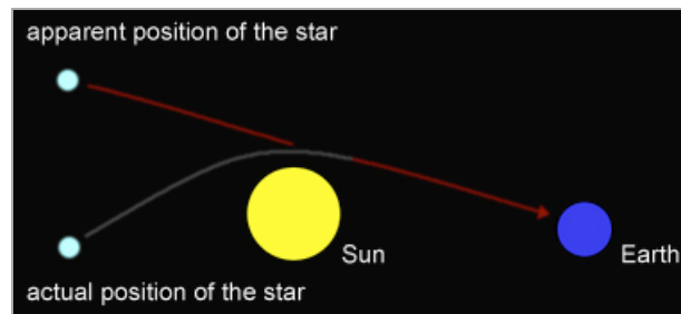
Figure 25: Bending of starlight by the sun.
