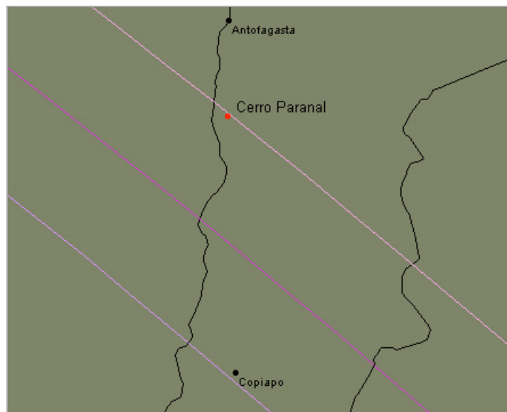
Figure 28: A part of the path of totality of the total solar eclipse on 2 nd of November 2339 (from Redshift 5.1).
