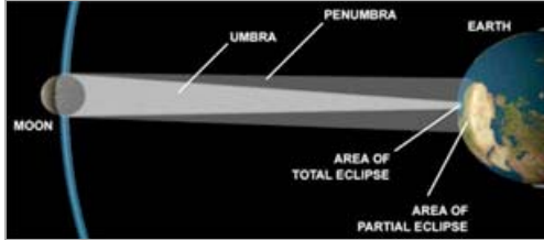
Figure 4: Total solar eclipse scheme (from 3D Atlas of the Universe).
