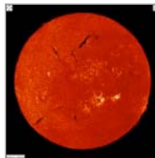
Figure 15: Sun in H-alpha (credit: Big Bear Solar Observatory).
