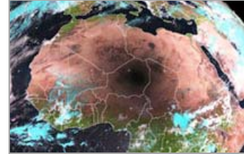
Figure 5: Lunar shadow during the total solar eclipse on 29 th of March 2006 (copyright © 2006 EUMETSAT).
