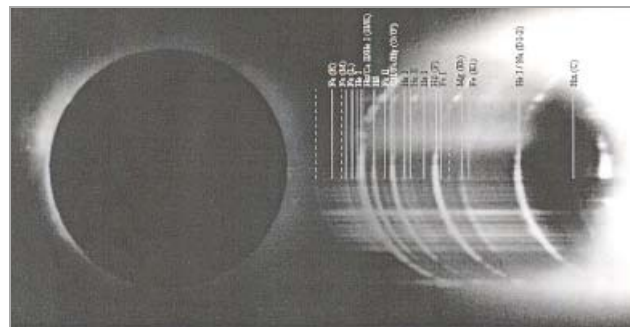
Figure 17: The flash spectrum during the total solar eclipse on 1 st of August 1999 (photo: Klaas Bakker, Amsterdam).
