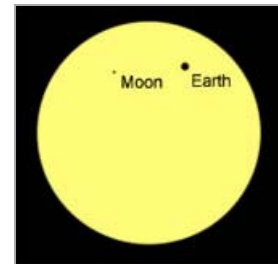
Figure 3: Earth transit observable from Mars in the year 2084.
