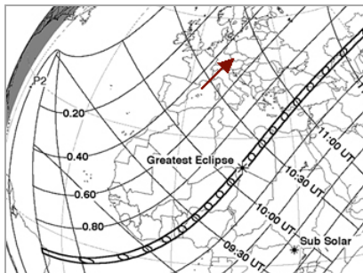
Figure 31: The approximate position of Písek on the map of the total solar eclipse (Fred Espenak, NASA's GSFC).
