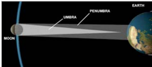
Figure 6: Annular solar eclipse scheme (from 3D Atlas of the Universe).
