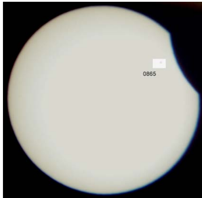
The partial solar eclipse during the finishing phase on the tablet behind the reflector. There is a group of sunspots in the picture.
