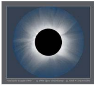
Figure 23: The solar corona during the total solar eclipse in the maximum of the solar activity (© 1995 Vojtech Rušin © 2004 Miloslav Druckmüller).
