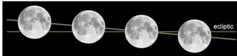
Figure 9: The Moon crosses the ecliptic.
