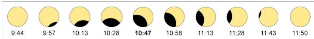
Figure 34: Graphic presentation of the eclipse (in UT).
