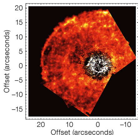
Figure 2. HST observations of the detached shell around R Scl in dust-scattered stellar light in the F814 filter observed with the Advanced Camera for Surveys (ACS) High Resolution Camera on HST. Due to the limited field of view of the ACS, only one third of the shell is covered in the image (from Olofsson et al., 2010).
