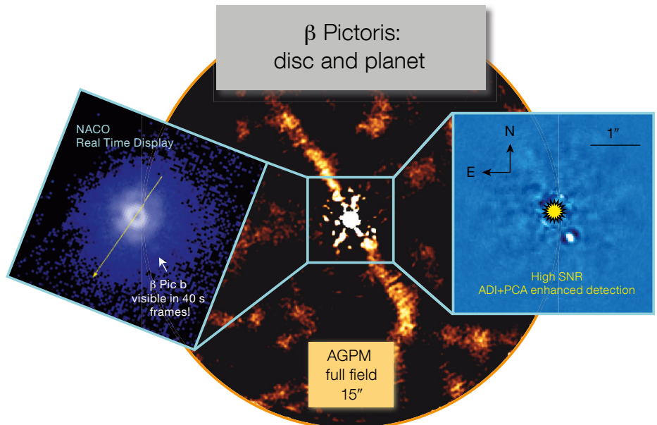
Figure 7. \beta Pictoris NACO+AGPM L' -band observations. This figure showcases the potential of the AGPM over a wide range of spatial scales: the central image represents the full field of view (15 arcseconds) of the AGPM with, at the centre, the masked star surrounded by both the planet (within 0.5 arcseconds) and the faint disc, several arcseconds away. On both sides, the central 4-arcsecond box is zoomed. The left image is a screen capture of the NACO real-time display (in log scale) which shows the star attenuated by the AGPM and the planet visible on single 40-second raw frames (DIT = 0.2 s, NDIT = 100). The right image shows the high signal-to-noise ratio detection of \beta Pictoris b applying modern post-processing techniques: angular differential imaging (ADI) and principal component analysis. North is up, east to the left.
