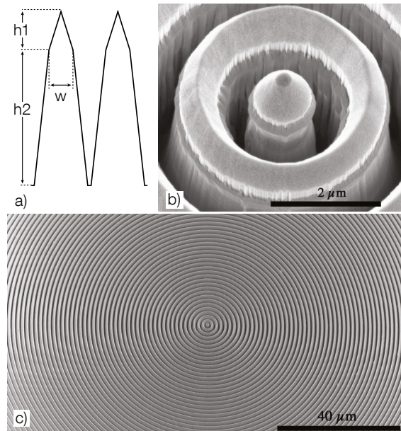
Figure 2. Scanning electron microscope images of the NACO AGPM made from diamond sub-wavelength gratings. a) The structure profile schematic, with h_2 = 5 \pm 0.1 \mu\text{m} , h_1 = 1 \pm 0.1 \mu\text{m} , and w = 0.65 \pm 0.03 \mu\text{m} (the grating pitch is 1.42 \mu\text{m} ). b) A zoom on the centre of the diamond AGPM. c) An overview of the structure showing the uniformity and original cleanliness of this particular device.
