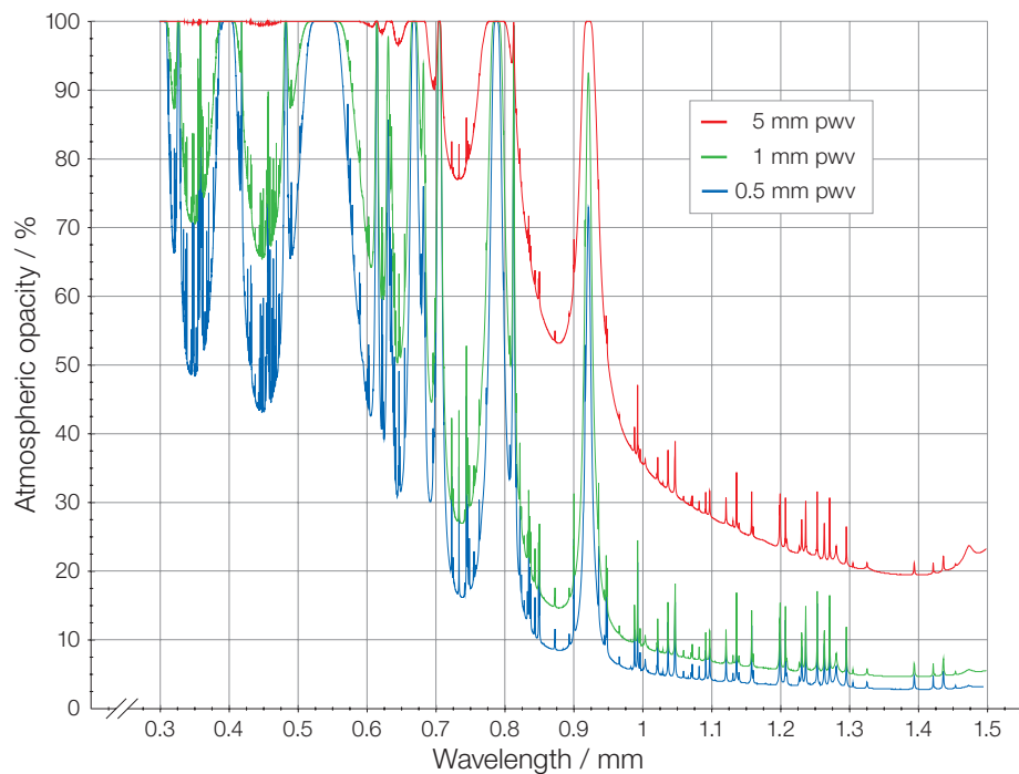
Figure 3.3 This graph shows a closer view of the millimetre and submillimetre wavelength region, with the different lines showing how the opacity depends strongly on the amount of precipitable water vapour (pwv) in the air. Credit: ESO/APEX
