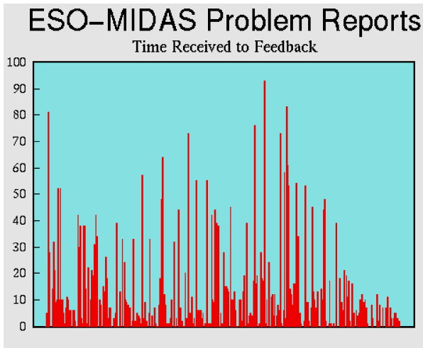
Figure 2.: Distribution of the feedback time, i.e. time between open and feedback state. The feedback time (ordinate, in days) is plotted for all 364 PRs (abscissa) received in the period May 1994 (left) till January 1995 (right).
