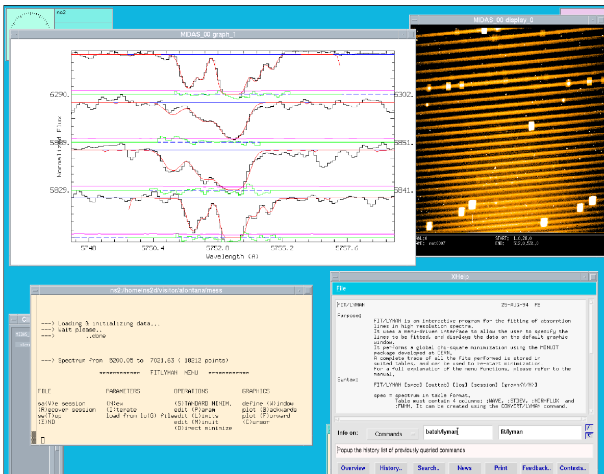
Example of a FITLYMAN session. The Main Menu is shown in the bottom left window. The graphic window over it displays a fit performed on a complex metal system at z=2.768 . Lines fitted are, from the top, Al_{1670} , CIV_{1550} , CIV_{1548} , SiII_{1526} . CIV doublet has been fitted with three components, lower ionization elements with five. Data from Giallongo et al. 1993 and J. Wampler.
