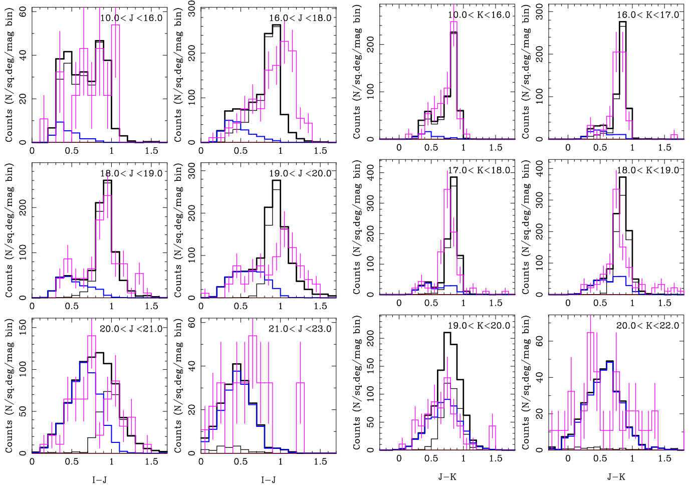
Fig. 6. ELECTRONIC ONLY Colour distributions, continued.
