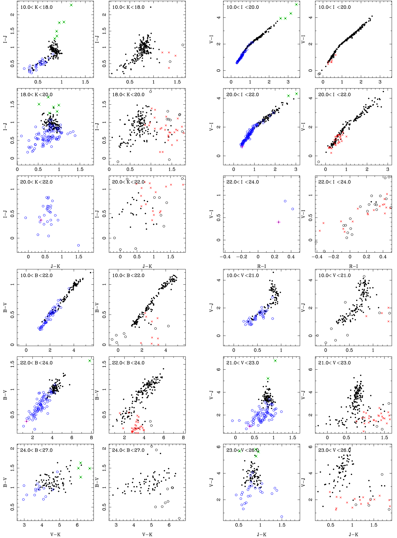
Fig. 4. ELECTRONIC ONLY Colour-colour diagrams for the seven passband catalogue, continued
