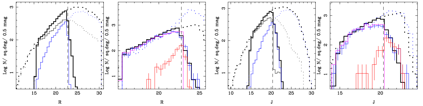
Fig. 3. Number counts in RJ with the power law form of the IMF from Chabrier (2001). The meaning of the curves is as in Fig. 2. The counts at R \sim 22 , J \sim 19.5 are about 20% larger than for the standard case with the lognormal form.
