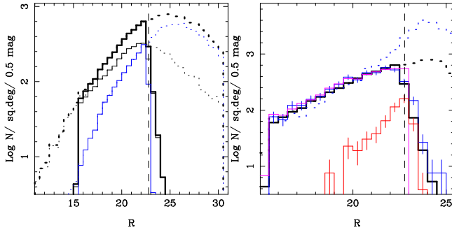
Fig. 2. Number counts in UBVRI from the five passband catalogue and in JK from the seven passband catalogue. This sample is for the R -band, and the full figure is only available in the on-line edition. In the lower right panel the R -band counts based on the seven passband catalogue are presented. They are in good agreement with those based on the five passband catalogue, as is the case for UBVI . Left panel: shown are the disk component (dashed and solid thin black histograms) and halo component (dashed and solid blue histograms), and their sum (dashed and solid thick black histograms) predicted by the galactic model. Distinguished are the predicted model counts taking into account the error model, saturation, completeness and the MAG_STAR_LIM in the individual passbands (the blue and black full histograms), as well as the “perfect” model (the blue and black dashed histograms). The morphological classification limits for the bands are indicated by the vertical dashed line. Right panel: comparison of the data (blue coloured histogram with errors bars) with the model. Note the different magnitude scale w.r.t. the left-hand panel. Shown are the predicted counts taking into account the error model, saturation and completeness (thick dotted black line), as well as the counts that additionally take into account the MAG_STAR_LIM limits in the individual passbands (thick solid black line; the same curve as in the left-hand panel). The pink histogram represents the observed number counts using the point source classification for that band only. The number counts of objects assigned “stellar” template spectra that are ranked 1 and \leq 3 in the full five and full seven passband catalogue respectively, based on the \chi^2 -technique only, are indicated by the dashed blue histogram. The QSO numbers counts (among the objects initially classified as point sources) are indicated by the red histogram. The morphological classification limits for the bands are indicated by the vertical dashed line.
