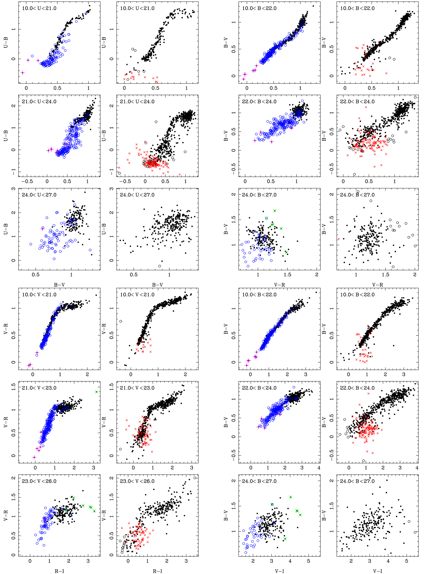
Fig. 4. ELECTRONIC ONLY Colour-colour diagram for different cuts in magnitude for the five passband catalogue. Left panel: Model predictions. Halo (open circles) and disk (filled circles), with stars with \log g > 7 (representing WDs) and stars with masses < 0.1 M_{\odot} (representing low mass stars) additionally marked by a plus and cross sign, respectively. Since the full simulation is run over n -times the observed area, only \frac{1}{n} of all model data points are plotted. Right panel: the data. Open circles represent outliers, in the sense that they are not
