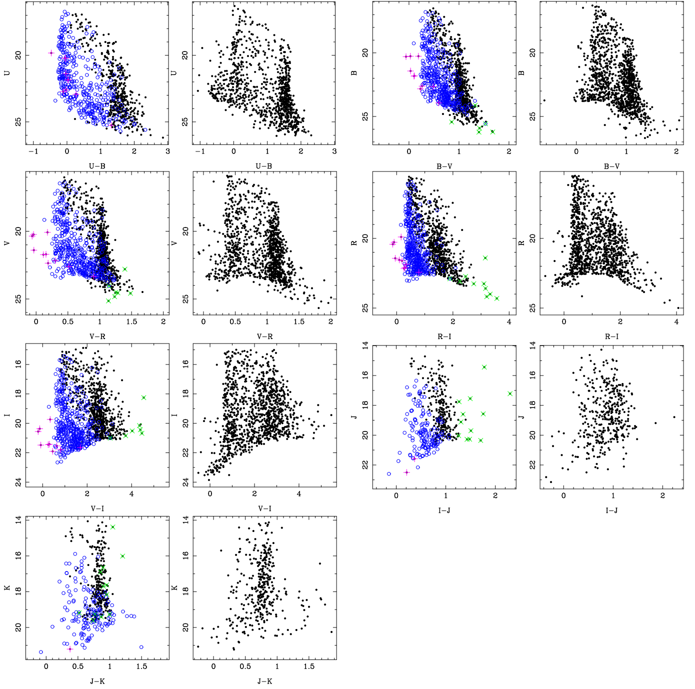
Fig. 5. ELECTRONIC ONLY Colour-magnitude diagram. Left panel: model results. The symbols have the same meaning as in Fig. 4. Since the full simulation is run over n -times the observed area, only \frac{1}{n} of all model data points are plotted. The right panel shows the data.
