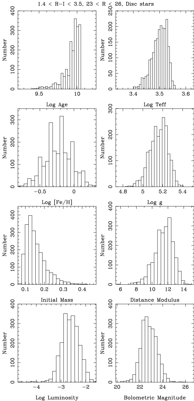
Fig. 7. Distributions over various parameters of all model stars which are formed in the disc and have 1.4 < R-I < 3.5 and 23 < R < 26 .
