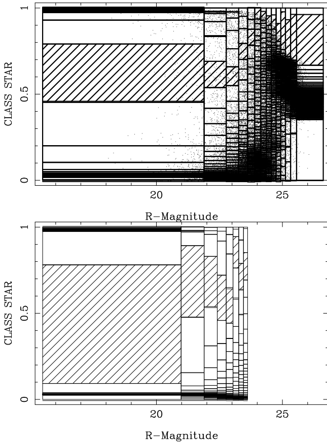
Fig. A.1. CLASS_STAR as a function of R -band magnitude, with the binning in magnitude and CLASS_STAR indicated, for the first pass (top), and second pass (bottom, without data points for clarity). The hatched bin is the one that defines the background of galaxies.
