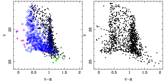
Fig. 5. Colour-magnitude diagram. This (V, V - R) diagram based on the five passband catalogue is a typical example and the full figure is only available through the on-line edition. Left panel: model results. The symbols have the same meaning as in Fig. 4. Since the full simulation is run over n -times the observed area, only \frac{1}{n} of all model data points are plotted. The right panel shows the data.
