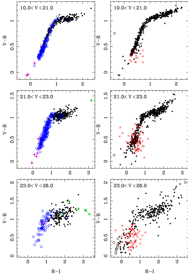
Fig. 4. Colour-colour diagram for different cuts in magnitude. This (V - R) - (R - I) diagram based on the five passband catalogue is a typical example and the full figure is only available through the on-line edition. Left panel: Model predictions. Halo (open circles) and disk (filled circles), with stars with \log g > 7 (representing WDs) and stars with masses < 0.1 M_{\odot} (representing low mass stars) additionally marked by a plus and cross sign, respectively. Since the full simulation is run over n -times the observed area, only \frac{1}{n} of all model data points are plotted. Right panel: the data. Open circles represent outliers, in the sense that they are not within a certain magnitude difference of any of the model data points in the left-hand panel (see text). Red crosses are objects identified as QSOs by the \chi^2 -technique.
