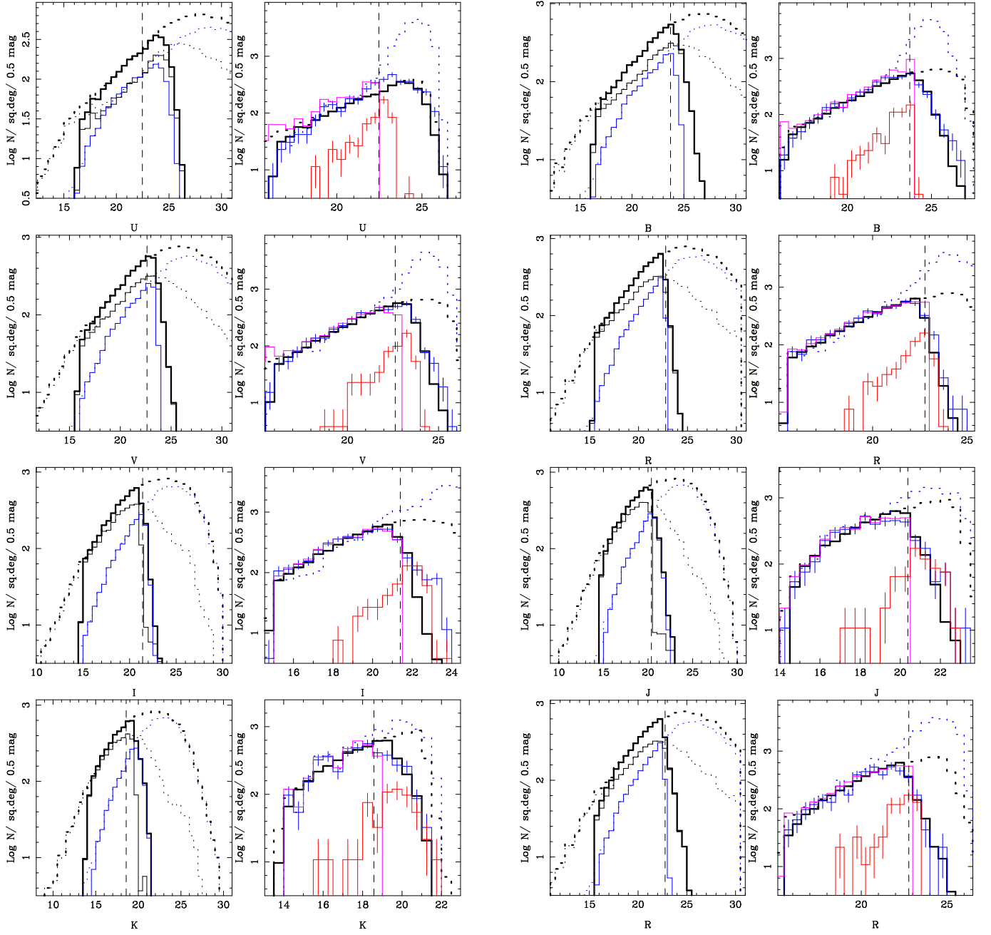
Fig. 2. ELECTRONIC ONLY Number counts in UBVRI from the five passband catalogue and in JK from the seven passband catalogue. In the lower right panel the R -band counts based on the seven passband catalogue are presented. They are in good agreement with those based on the five passband catalogue, as is the case for UBVI . Left panel: shown are the disk component (dashed and solid thin black histograms) and halo component (dashed and solid blue histograms), and their sum (dashed and solid thick black histograms) predicted by the galactic model. Distinguished are the predicted model counts taking into account the error model, saturation, completeness and the MAG_STAR_LIM in the individual passbands (the blue and black full histograms), as well as the “perfect” model (the blue and black dashed histograms). The morphological classification limits for the bands are indicated by the vertical dashed line. Right panel: comparison of the data (blue coloured histogram with errors bars) with the model. Note the different magnitude scale w.r.t. the left-hand panel. Shown are the predicted counts taking into account the error model, saturation and completeness (thick dotted black line), as well as the counts that additionally take into account the MAG_STAR_LIM limits in the individual passbands (thick solid black line; the same curve as in the left-hand panel). The pink histogram represents the observed number counts using the point source classification for that band only. The number counts of objects assigned “stellar” template spectra that are ranked 1 and \leq 3 in the full five and full seven passband catalogue respectively, based on the \chi^2 -technique only, are indicated by the dashed blue histogram. The QSO numbers counts (among the objects initially classified as point sources) are indicated by the red histogram. The morphological classification limits for the bands are indicated by the vertical dashed line.
