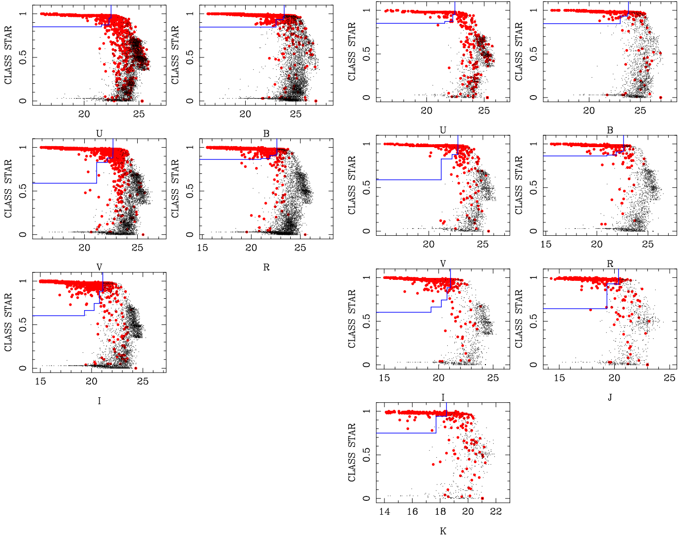
Fig. 8. ELECTRONIC ONLY \text{CLASS\_STAR} values of the objects that are classified as point sources in the five and seven passband colour catalogues (filled red circles). Black dots represent the \text{CLASS\_STAR} values of the objects that are classified as “stellar” and that are ranked 1 and \leq 3 in the full five and full seven passband catalogue respectively, when applying the \chi^2 -technique. \text{MAG\_STAR\_LIM} and \text{CLASS\_STAR} limits are indicated.
