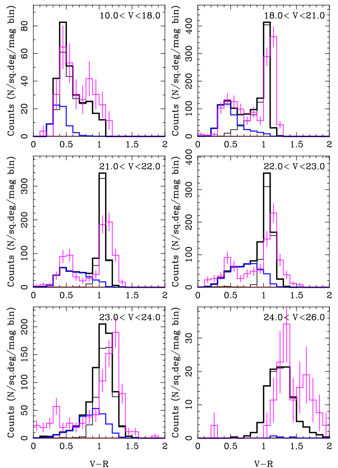
Fig. 6. Colour distributions for different cuts in magnitude. The full figure is only available through the on-line edition. Shown are the model predictions (the halo is the blue lined histogram; the disk the thin lined histogram, and their sum is the thick lined histogram) and the data (the pink histogram with the error bars).
