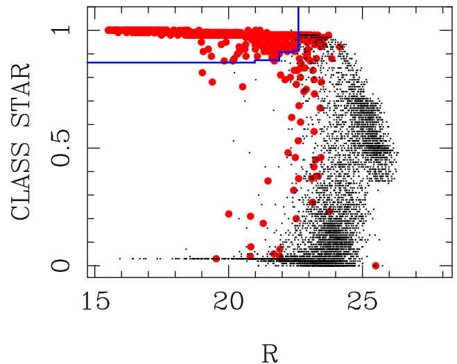
Fig. 8. CLASS\_STAR values of the objects that are classified as point sources in the five and seven passband colour catalogues (filled red circles). This panel shows the R -band based on the five passband catalogue as an example, and the full figure is only available through the on-line edition. Black dots represent the CLASS\_STAR values of the objects that are classified as “stellar” and that are ranked 1 and \leq 3 in the full five and full seven passband catalogue respectively, when applying the \chi^2 -technique. MAG\_STAR\_LIM and CLASS\_STAR limits are indicated.
