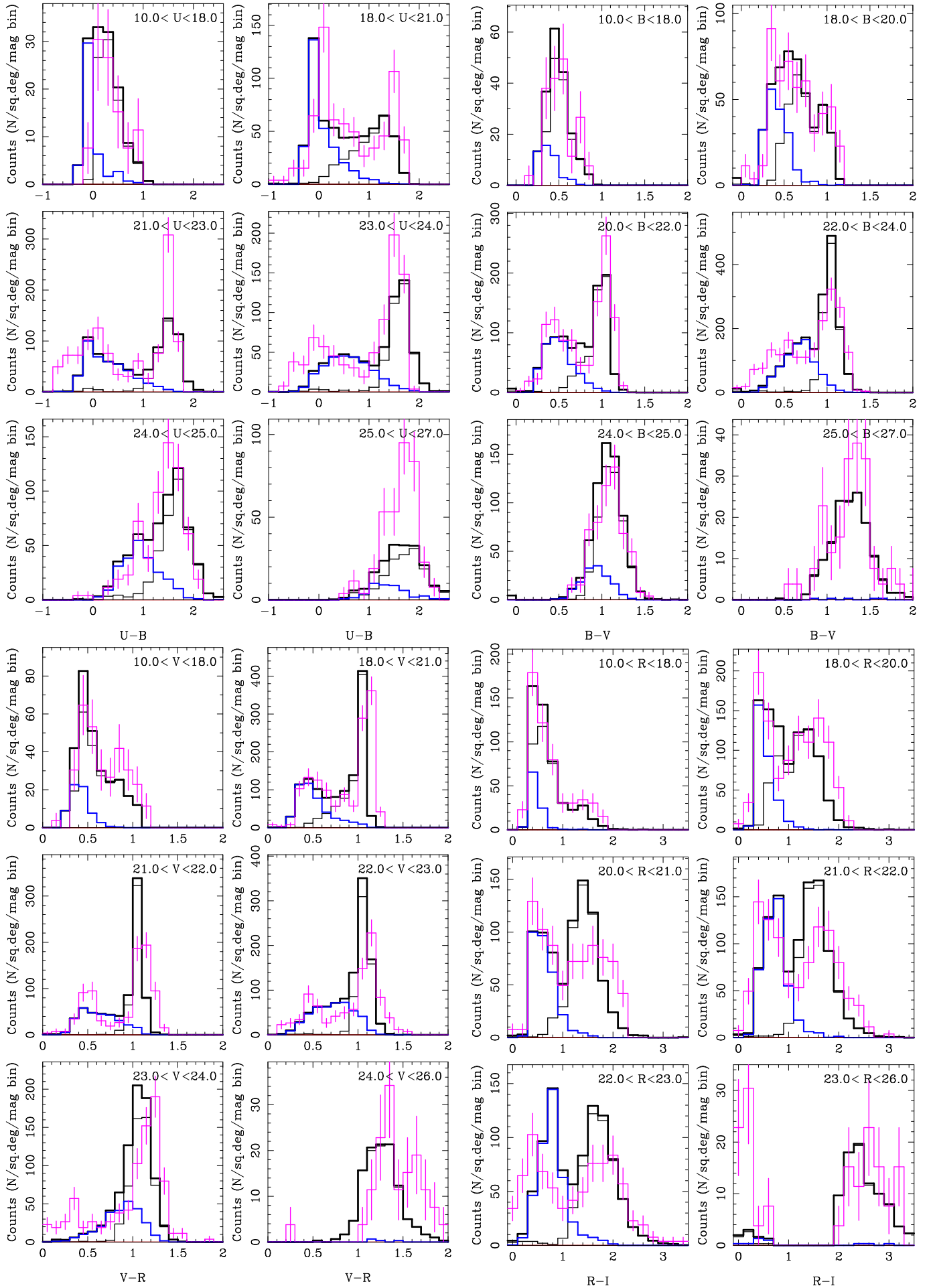
Fig. 6. ELECTRONIC ONLY Colour distributions for different cuts in magnitude. Shown are the model predictions (the halo is the blue lined histogram; the disk the thin lined histogram, and their sum is the thick lined histogram) and the data (the pink histogram with the error bars).
