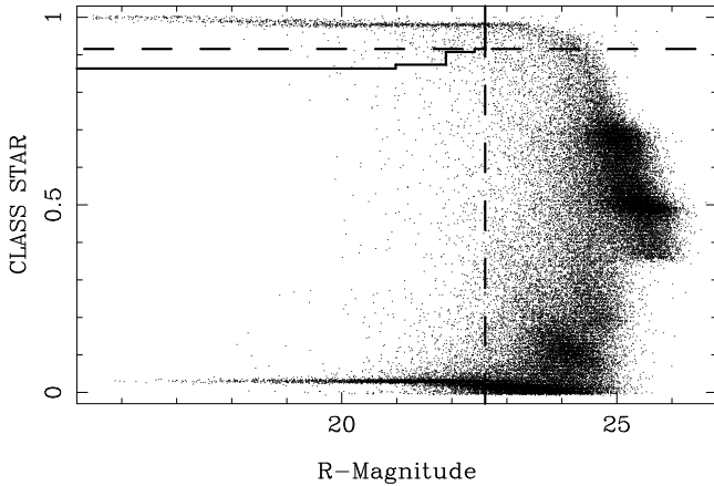
Fig. 1. SExtractor parameter CLASS_STAR versus magnitude for the R -band, with the finally adopted morphological classification limits indicated by the solid line. Objects in the upper left box are considered point sources in a single passband. The dashed line indicates the much simpler criterion used previously which only took into account the CLASS_STAR value at the faintest MAG_STAR_LIM .
