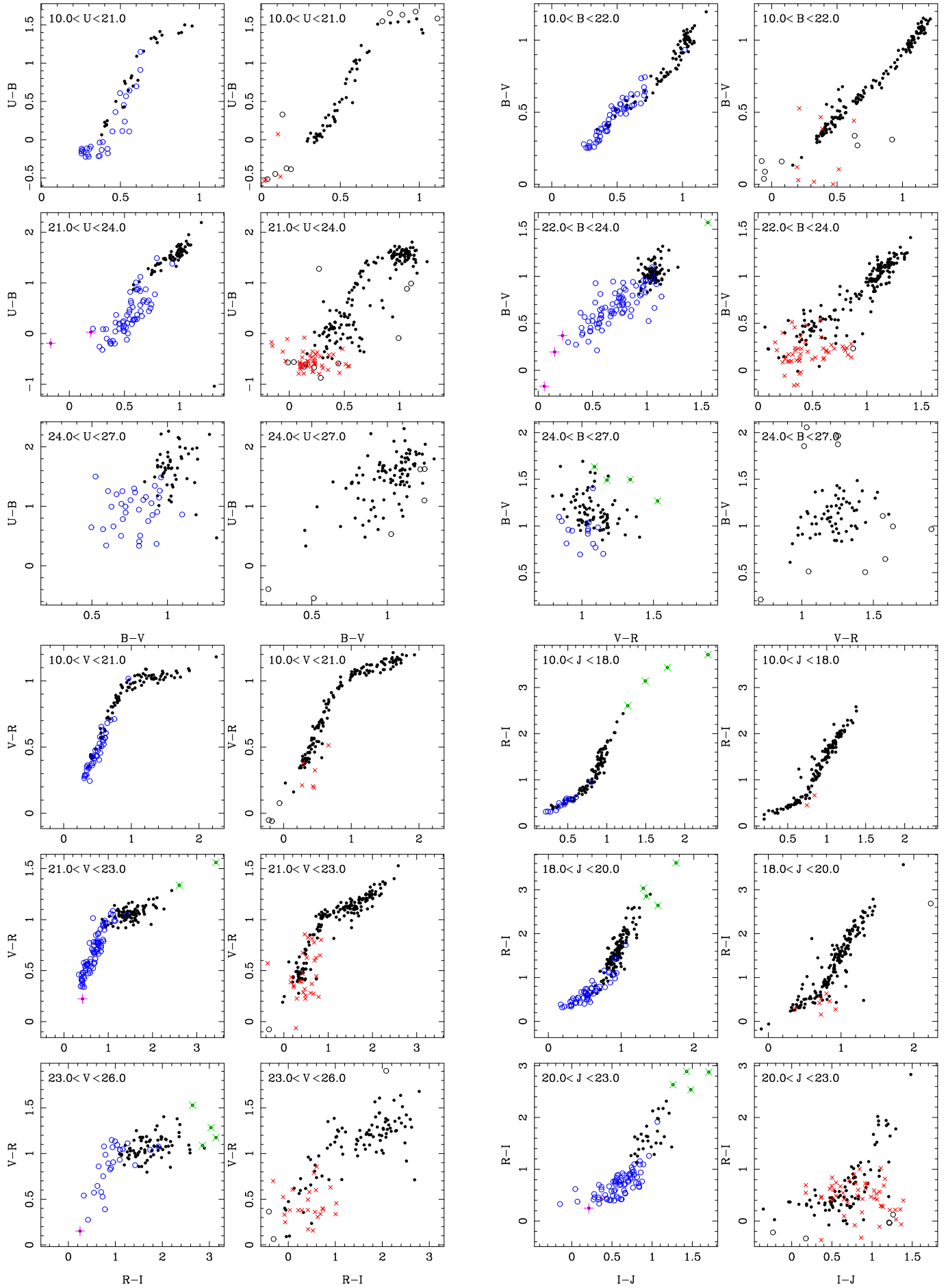
Fig. 4. ELECTRONIC ONLY Continued. Colour-colour diagram for different cuts in magnitude for the seven passband catalogue.
