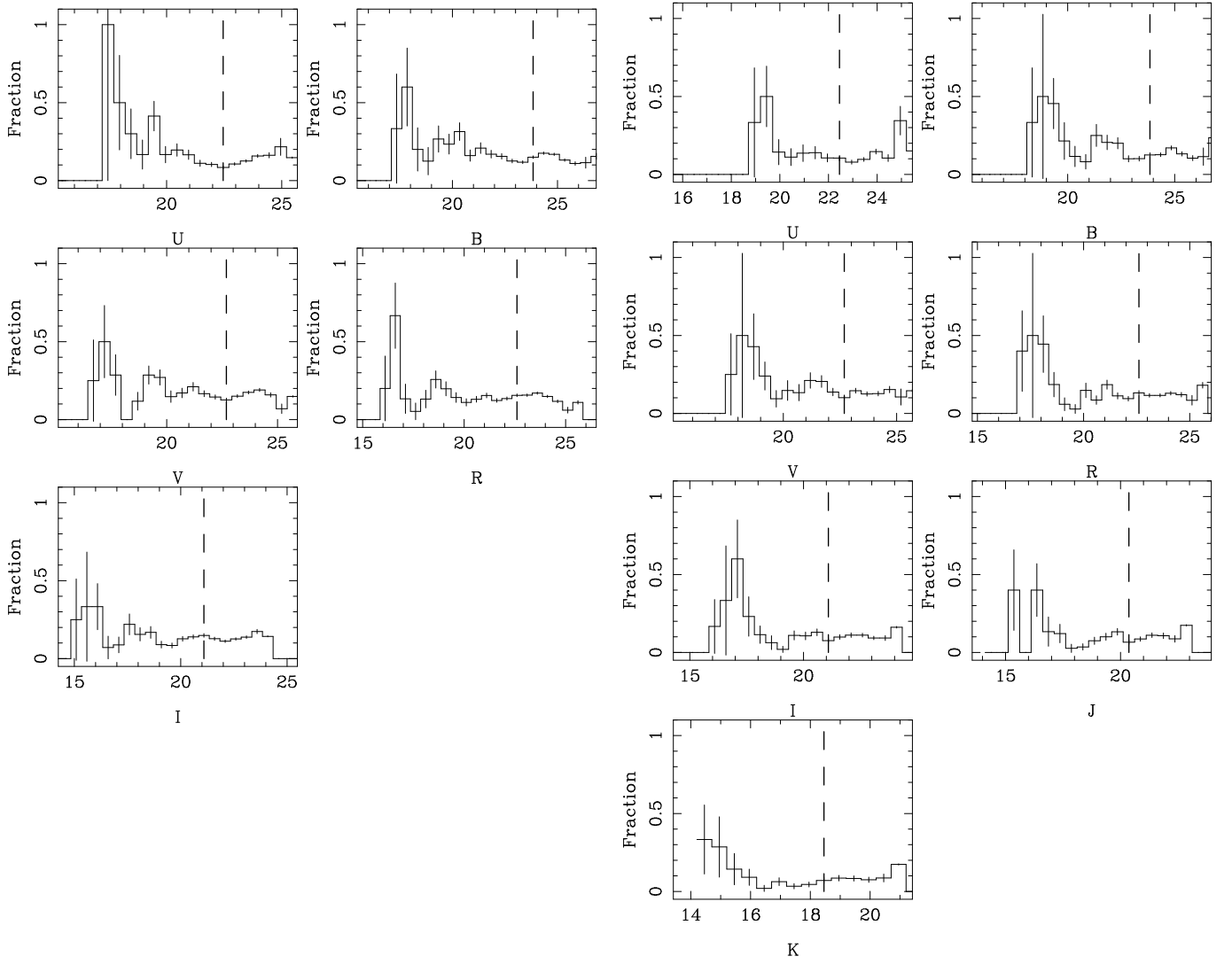
Fig. 9. ELECTRONIC ONLY Fraction of objects that are classified as “stellar” and that are ranked 1 and \leq 3 in the full five and full seven passband catalogue respectively, when applying the \chi^2 -technique and that have a CLASS\_STAR less than 0.1. MAG\_STAR\_LIM limits are indicated.
