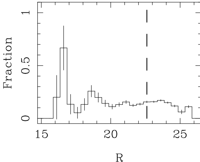
Fig. 9. Fraction of objects that are classified as “stellar” and that are ranked 1 and \leq 3 in the full five and full seven passband catalogue respectively, when applying the \chi^2 -technique and that have a CLASS_STAR less than 0.1. MAG_STAR_LIM limits are indicated. This panel shows the R -band based on the five passband catalogue as an example and the full figure is only available through the on-line edition.
